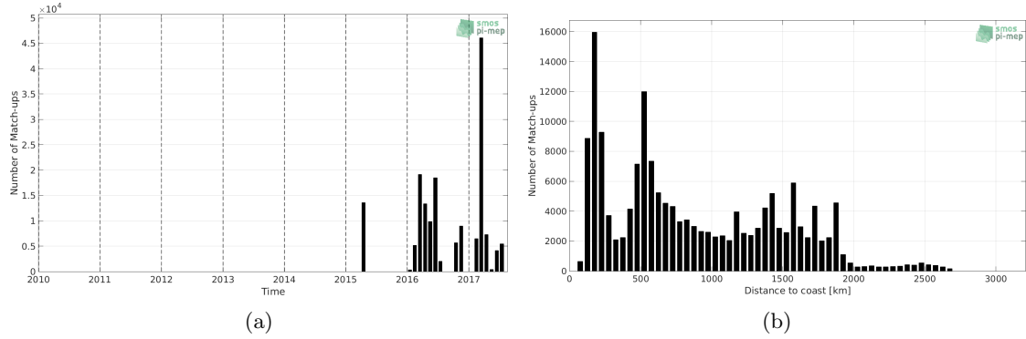
Figure 1: Number of match-ups between TSG-GOSUD-Research-vessel and SMAP-L3-RSS-V3-MONTHLY-70KM SSS as a function of time (a) and as function of the distance to coast (b) over the Tropical Atlantic Ocean Pi-MEP region and for the full satellite product period.
