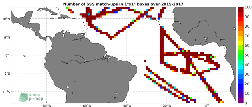
Figure 4: Number of SSS match-ups between TSG-GOSUD-Research-vessel SSS and the SMAP-L3-RSS-V3-MONTHLY-70KM SSS product for the Tropical Atlantic Ocean Pi-MEP region over 1^\circ \times 1^\circ boxes and for the full satellite product period.
