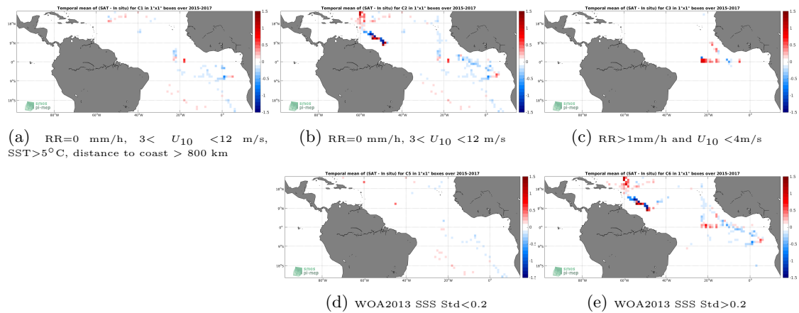
Figure 12: Temporal mean gridded over spatial boxes of size 1^\circ \times 1^\circ of \Delta SSS (SMAP-L3-RSS-V3-MONTHLY-70KM - TSG-GOSUD-Research-vessel) for 5 different subdatasets corresponding to:RR=0 mm/h, 3 < U_{10} < 12 m/s, SST >5^\circ C, distance to coast > 800 km (a), RR=0 mm/h, 3 < U_{10} < 12 m/s (b), RR >1 mm/h and U_{10} < 4 m/s (c), WOA2013 SSS Std <0.2 (d), WOA2013 SSS Std >0.2 (e).
