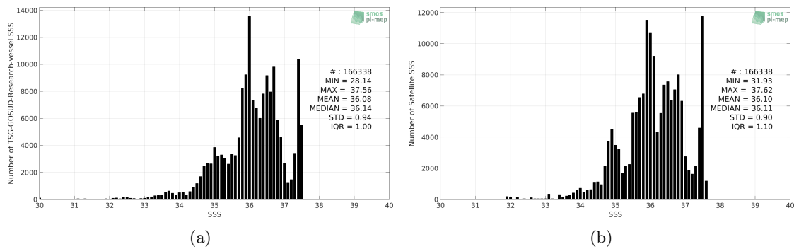
Figure 2: Histograms of SSS from TSG-GOSUD-Research-vessel (a) and SMAP-L3-RSS-V3-MONTHLY-70KM (b) considering all match-up pairs per bins of 0.1 over the Tropical Atlantic Ocean Pi-MEP region and for the full satellite product period.
