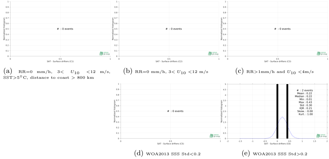
Figure 12: Normalized histogram of \Delta\text{SSS} (SMAP-L3-RSS-V3-MONTHLY-70KM - Surface drifters) for 5 different subdatasets corresponding to: RR=0 mm/h, 3 < U_{10} < 12 m/s, SST > 5^\circ\text{C} , distance to coast > 800 km (a), RR=0 mm/h, 3 < U_{10} < 12 m/s (b), RR > 1\text{mm/h} and U_{10} < 4\text{m/s} (c), WOA2013 SSS Std < 0.2 (d), WOA2013 SSS Std > 0.2 (e).
