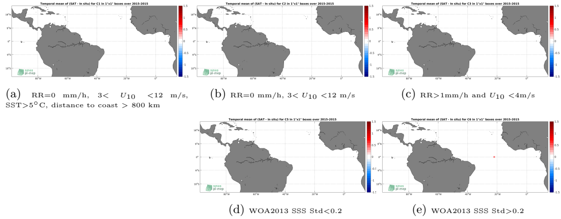
Figure 11: Temporal mean gridded over spatial boxes of size 1^\circ \times 1^\circ of \Delta SSS (SMAP-L3-RSS-V3-MONTHLY-70KM - Surface drifters) for 5 different subdatasets corresponding to: RR=0 mm/h, 3 < U_{10} < 12 m/s, SST > 5^\circ C , distance to coast > 800 km (a), RR=0 mm/h, 3 < U_{10} < 12 m/s (b), RR > 1 mm/h and U_{10} < 4 m/s (c), WOA2013 SSS Std < 0.2 (d), WOA2013 SSS Std > 0.2 (e).
