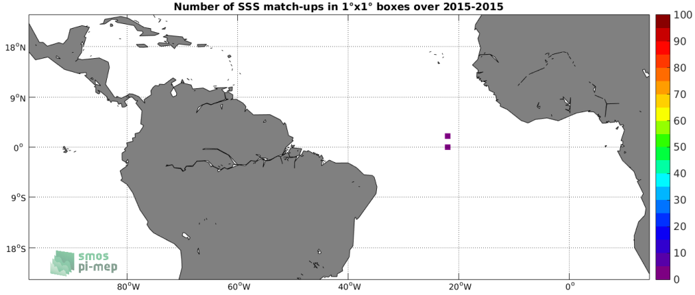
Figure 3: Number of SSS match-ups between Surface drifters SSS and the SMAP-L3-RSS-V3-MONTHLY-70KM SSS product for the Tropical Atlantic Ocean Pi-MEP region over 1^\circ \times 1^\circ boxes and for the full satellite product period.
