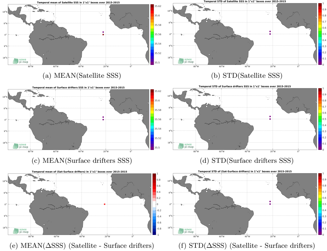
Figure 5: Temporal mean (left) and STD (right) of SSS from SMAP-L3-RSS-V3-MONTHLY-70KM (top), Surface drifters (middle), and of \Delta SSS (Satellite - Surface drifters). Only match-up pairs are used to generate these maps.
