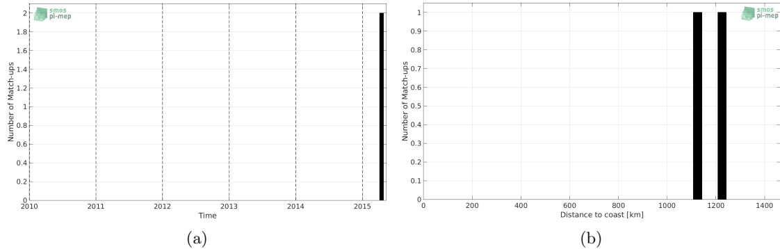
Figure 1: Number of match-ups between Surface drifters and SMAP-L3-RSS-V3-MONTHLY-70KM SSS as a function of time (a) and as function of the distance to coast (b) over the Tropical Atlantic Ocean Pi-MEP region and for the full satellite product period.
