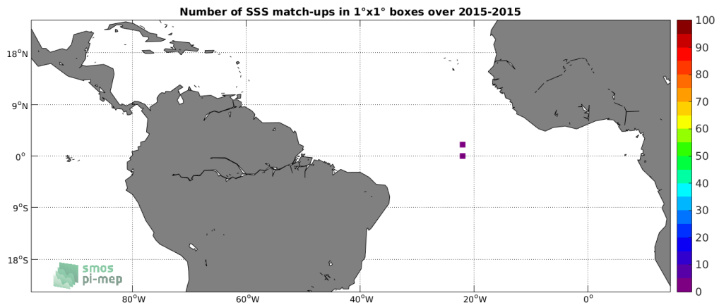
Figure 3: Number of SSS match-ups between Surface drifters SSS and the SMAP-L3-RSS-V3-MONTHLY-70KM SSS product for the Tropical Atlantic Ocean Pi-MEP region over 1°x1° boxes and for the full satellite product period.
