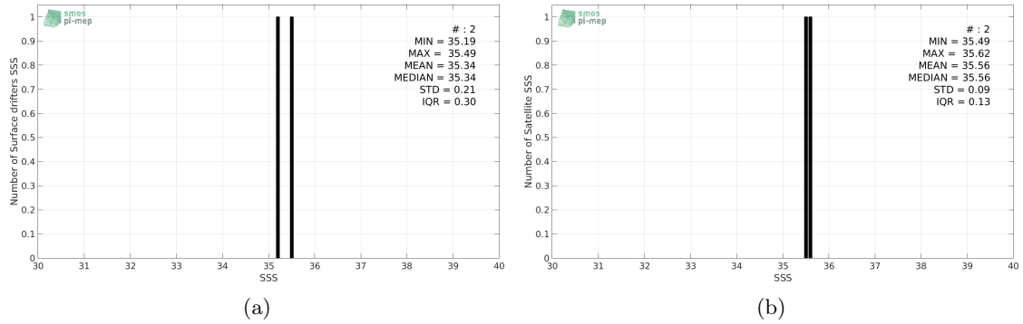
Figure 2: Histograms of SSS from Surface drifters (a) and SMAP-L3-RSS-V3-MONTHLY-70KM (b) considering all match-up pairs per bins of 0.1 over the Tropical Atlantic Ocean Pi-MEP region and for the full satellite product period.
