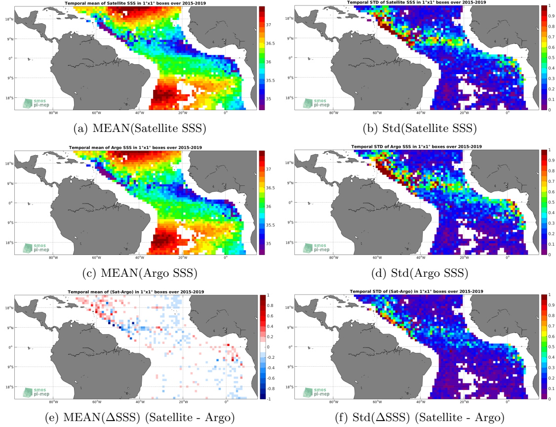
Figure 6: Temporal mean (left) and Std (right) of SSS from SMAP-L3-RSS-V3-MONTHLY-70KM (top), Argo (middle), and of \Delta SSS (Satellite - Argo). Only match-up pairs are used to generate these maps.
