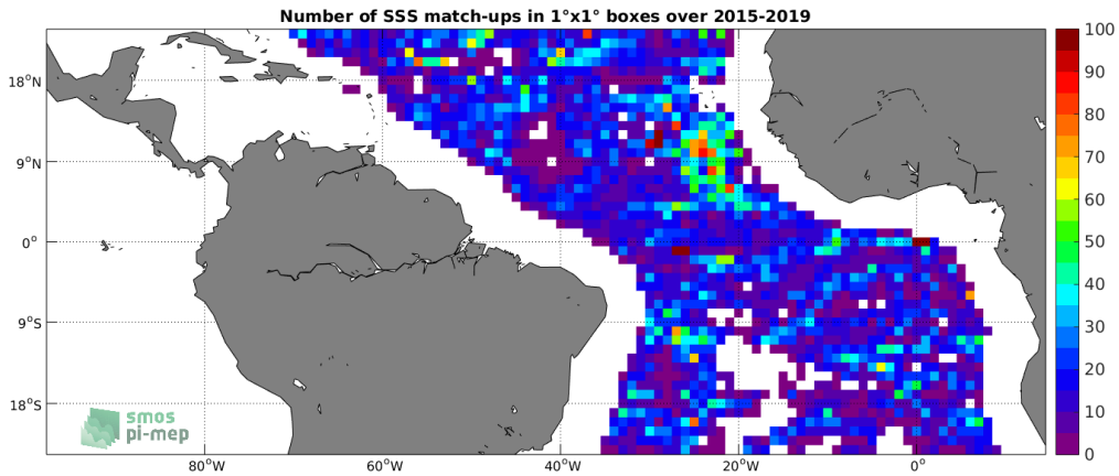
Figure 4: Number of SSS match-ups between Argo SSS and the SMAP-L3-RSS-V3-MONTHLY-70KM SSS product for the Tropical Atlantic Ocean Pi-MEP region over 1^\circ \times 1^\circ boxes and for the full satellite product period.
