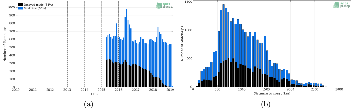
Figure 1: Number of match-ups between Argo and SMAP-L3-RSS-V3-MONTHLY-70KM SSS as a function of time (a) and as function of the distance to coast (b) over the Tropical Atlantic Ocean Pi-MEP region and for the full satellite product period.
