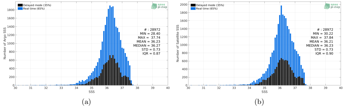
Figure 2: Histograms of SSS from Argo (a) and SMAP-L3-RSS-V3-MONTHLY-70KM (b) considering all match-up pairs per bins of 0.1 over the Tropical Atlantic Ocean Pi-MEP region and for the full satellite product period.
