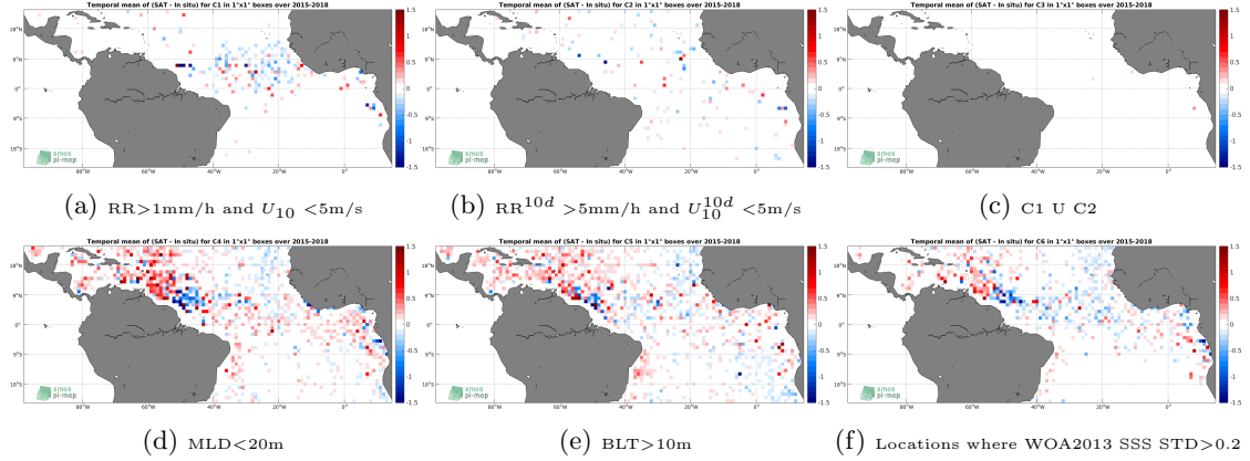
Figure 12: Temporal mean gridded over spatial boxes of size 1^\circ \times 1^\circ of \Delta SSS (SMAP-L3-RSS-V3-MONTHLY-70KM - Argo) for 6 different subdatasets corresponding to: RR > 1\text{mm/h} and U_{10} < 5\text{m/s} (a), RR^{10d} > 5\text{mm/h} and U_{10}^{10d} < 5\text{m/s} (b), C1 U C2 (c), MLD < 20\text{m} (d), BLT > 10\text{m} (e), Locations where WOA2013 SSS STD > 0.2 (f).
