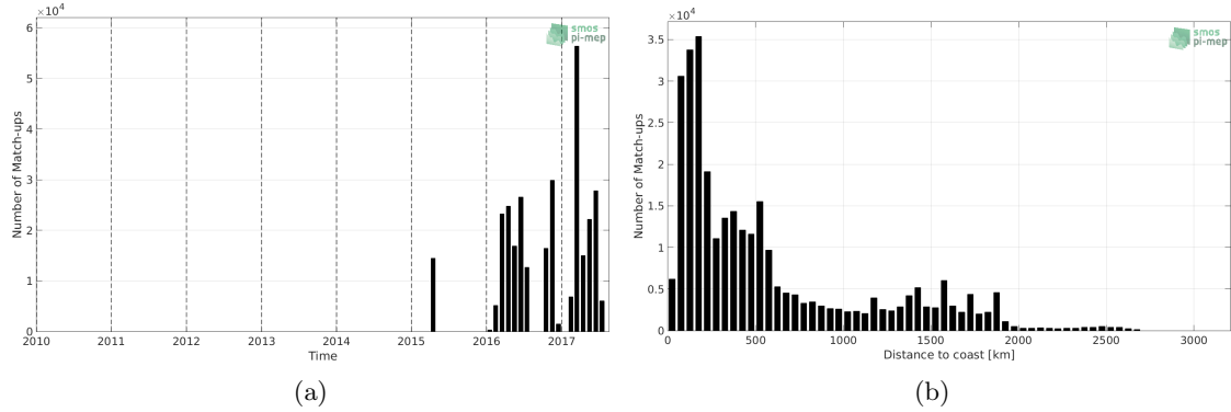
Figure 1: Number of match-ups between TSG-GOSUD-Research-vessel and SMAP-L3-RSS-V3-MONTHLY-0.25DEG-40KM SSS as a function of time (a) and as function of the distance to coast (b) over the Tropical Atlantic Ocean Pi-MEP region and for the full satellite product period.
