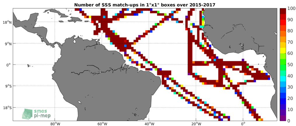
Figure 4: Number of SSS match-ups between TSG-GOSUD-Research-vessel SSS and the SMAP-L3-RSS-V3-MONTHLY-0.25DEG-40KM SSS product for the Tropical Atlantic Ocean Pi-MEP region over 1^\circ \times 1^\circ boxes and for the full satellite product period.
