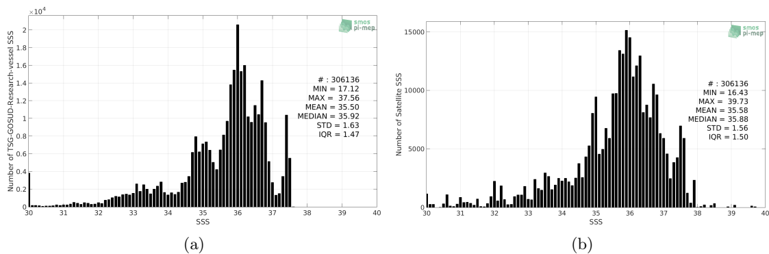
Figure 2: Histograms of SSS from TSG-GOSUD-Research-vessel (a) and SMAP-L3-RSS-V3-MONTHLY-0.25DEG-40KM (b) considering all match-up pairs per bins of 0.1 over the Tropical Atlantic Ocean Pi-MEP region and for the full satellite product period.
