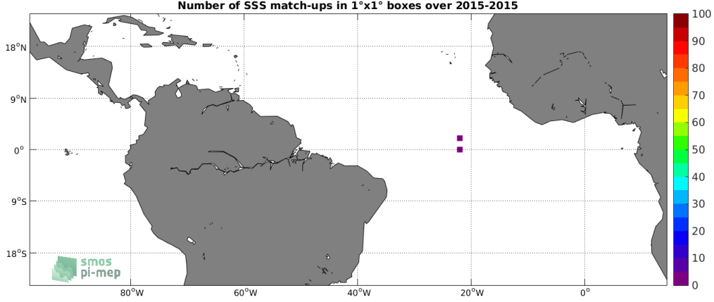
Figure 3: Number of SSS match-ups between Surface drifters SSS and the SMAP-L3-RSS-V3-MONTHLY-0.25DEG-40KM SSS product for the Tropical Atlantic Ocean Pi-MEP region over 1^\circ \times 1^\circ boxes and for the full satellite product period.
