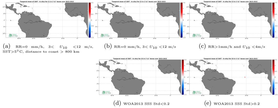
Figure 11: Temporal mean gridded over spatial boxes of size 1^\circ \times 1^\circ of \Delta SSS (SMAP-L3-RSS-V3-MONTHLY-0.25DEG-40KM - Surface drifters) for 5 different subdatasets corresponding to: RR=0 mm/h, 3 < U_{10} < 12 m/s, SST > 5^\circ C , distance to coast > 800 km (a), RR=0 mm/h, 3 < U_{10} < 12 m/s (b), RR > 1 mm/h and U_{10} < 4 m/s (c), WOA2013 SSS Std < 0.2 (d), WOA2013 SSS Std > 0.2 (e).
