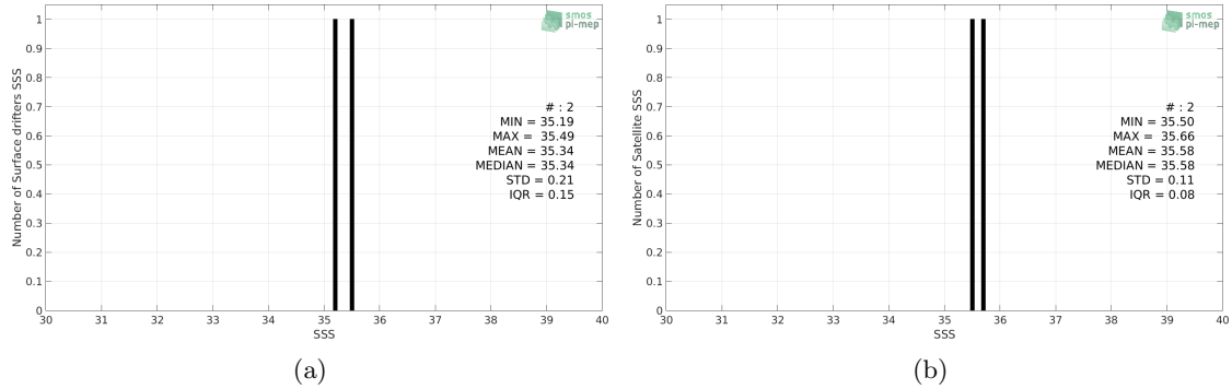
Figure 2: Histograms of SSS from Surface drifters (a) and SMAP-L3-RSS-V3-MONTHLY-0.25DEG-40KM (b) considering all match-up pairs per bins of 0.1 over the Tropical Atlantic Ocean Pi-MEP region and for the full satellite product period.
