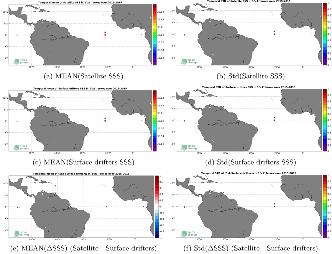
Figure 5: Temporal mean (left) and Std (right) of SSS from SMAP-L3-RSS-V3-MONTHLY-0.25DEG-40KM (top), Surface drifters (middle), and of \Delta SSS (Satellite - Surface drifters). Only match-up pairs are used to generate these maps.
