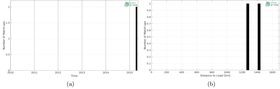
Figure 1: Number of match-ups between Surface drifters and SMAP-L3-RSS-V3-MONTHLY-0.25DEG-40KM SSS as a function of time (a) and as function of the distance to coast (b) over the Tropical Atlantic Ocean Pi-MEP region and for the full satellite product period.
