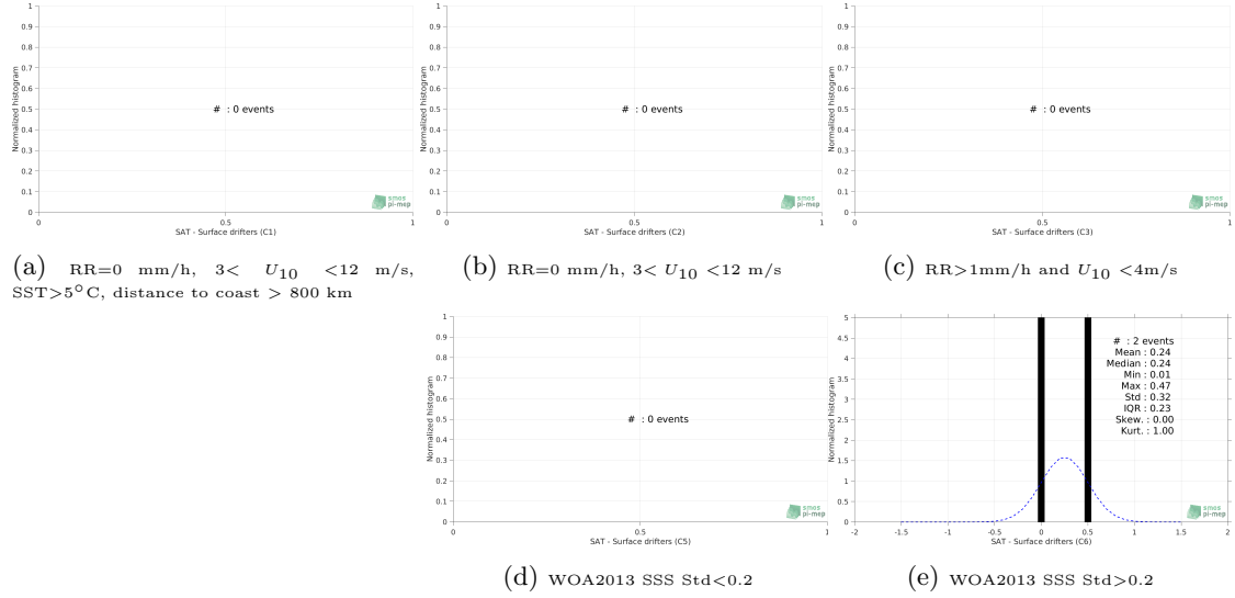
Figure 12: Normalized histogram of \Delta\text{SSS} (SMAP-L3-RSS-V3-MONTHLY-0.25DEG-40KM - Surface drifters) for 5 different subdatasets corresponding to: RR=0 mm/h, 3 < U_{10} < 12 m/s, SST > 5^\circ\text{C} , distance to coast > 800 km (a), RR=0 mm/h, 3 < U_{10} < 12 m/s (b), RR > 1 mm/h and U_{10} < 4 m/s (c), WOA2013 SSS Std < 0.2 (d), WOA2013 SSS Std > 0.2 (e).
