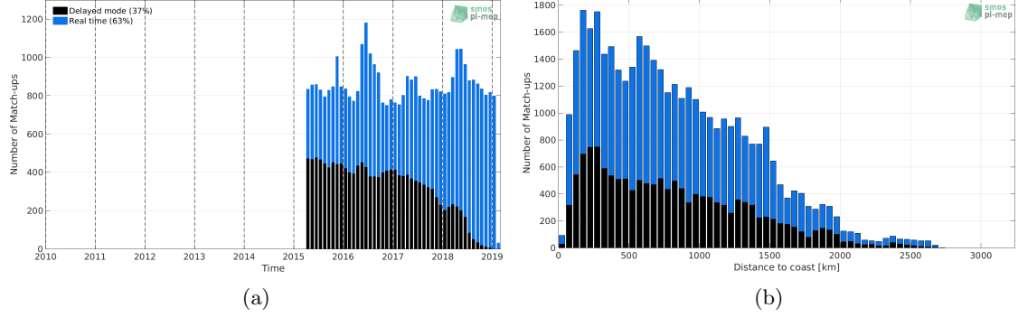
Figure 1: Number of match-ups between Argo and SMAP-L3-RSS-V3-MONTHLY-0.25DEG-40KM SSS as a function of time (a) and as function of the distance to coast (b) over the Tropical Atlantic Ocean Pi-MEP region and for the full satellite product period.
