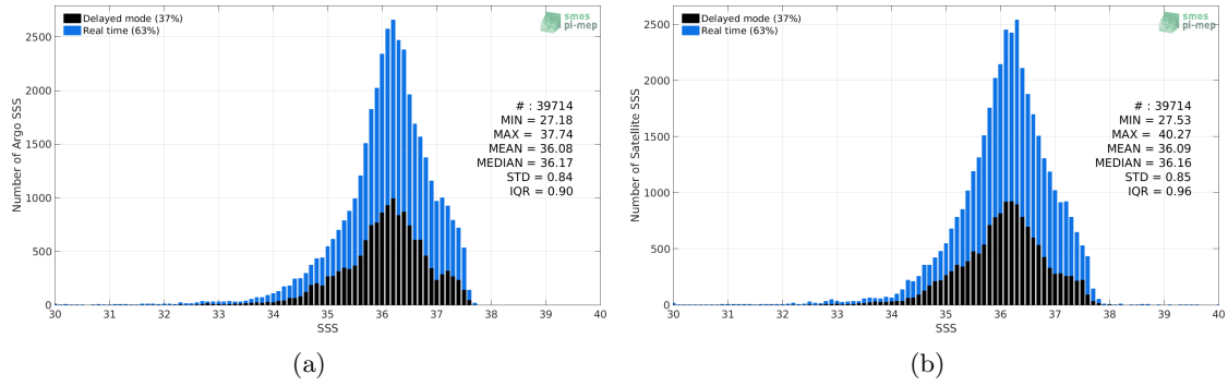
Figure 2: Histograms of SSS from Argo (a) and SMAP-L3-RSS-V3-MONTHLY-0.25DEG-40KM (b) considering all match-up pairs per bins of 0.1 over the Tropical Atlantic Ocean Pi-MEP region and for the full satellite product period.
