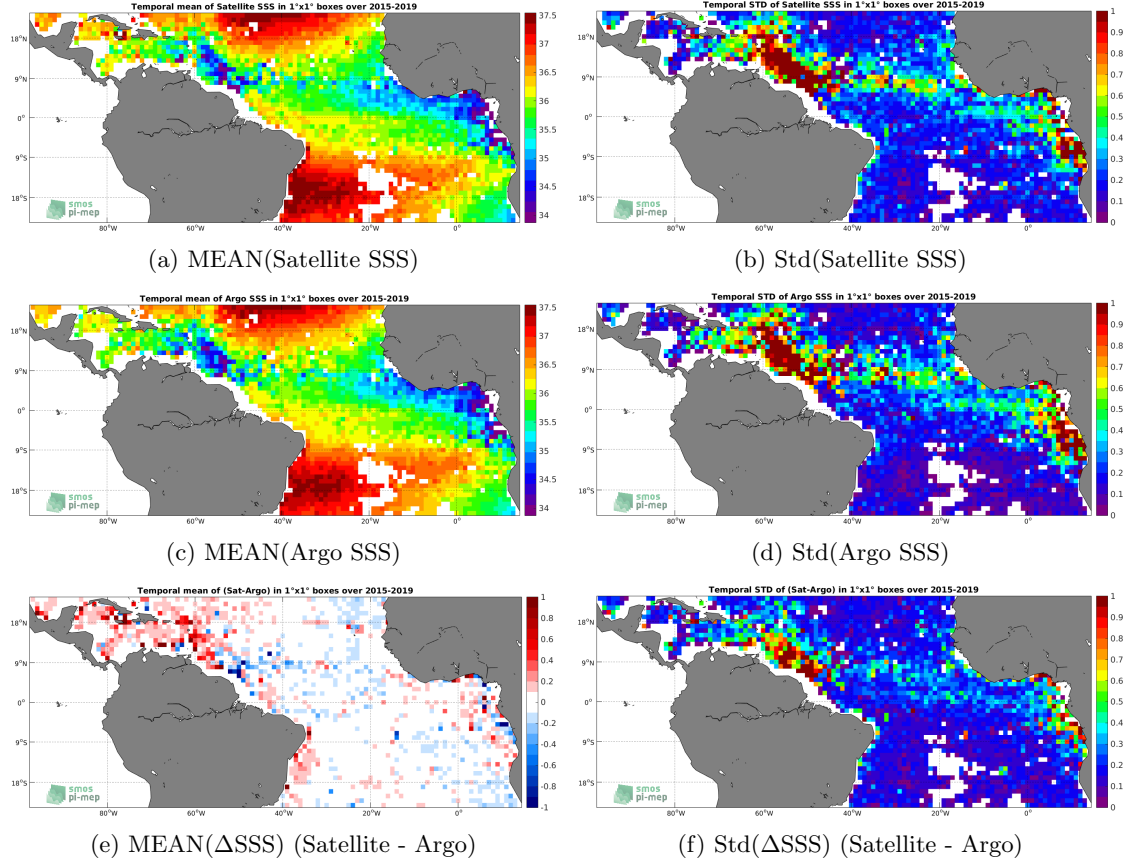
Figure 6: Temporal mean (left) and Std (right) of SSS from SMAP-L3-RSS-V3-MONTHLY-0.25DEG-40KM (top), Argo (middle), and of \Delta SSS (Satellite - Argo). Only match-up pairs are used to generate these maps.
