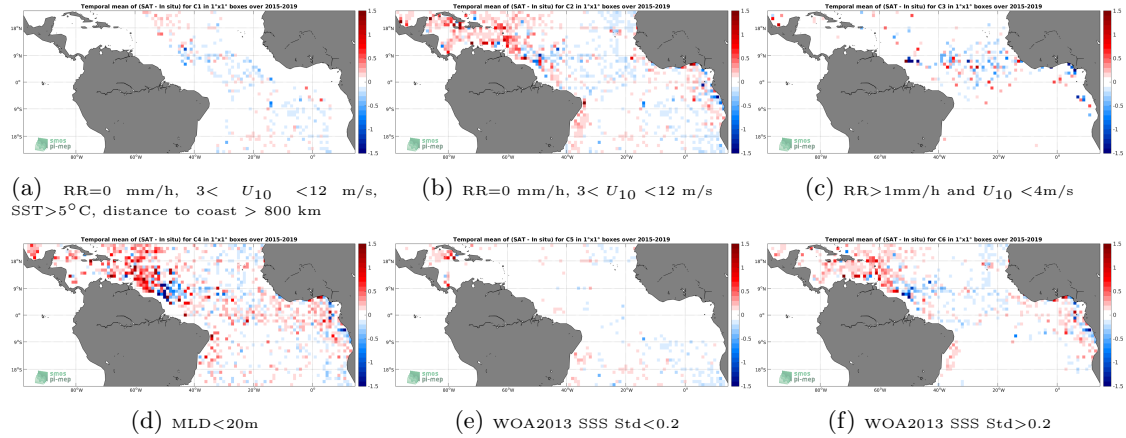
Figure 12: Temporal mean gridded over spatial boxes of size 1^\circ \times 1^\circ of \Delta SSS (SMAP-L3-RSS-V3-MONTHLY-0.25DEG-40KM - Argo) for 6 different subdatasets corresponding to: RR=0 mm/h, 3 < U_{10} < 12 m/s, SST > 5^\circ\text{C} , distance to coast > 800 km (a), RR=0 mm/h, 3 < U_{10} < 12 m/s (b), RR > 1 mm/h and U_{10} < 4 m/s (c), MLD < 20 m (d), WOA2013 SSS Std < 0.2 (e), WOA2013 SSS Std > 0.2 (f).
