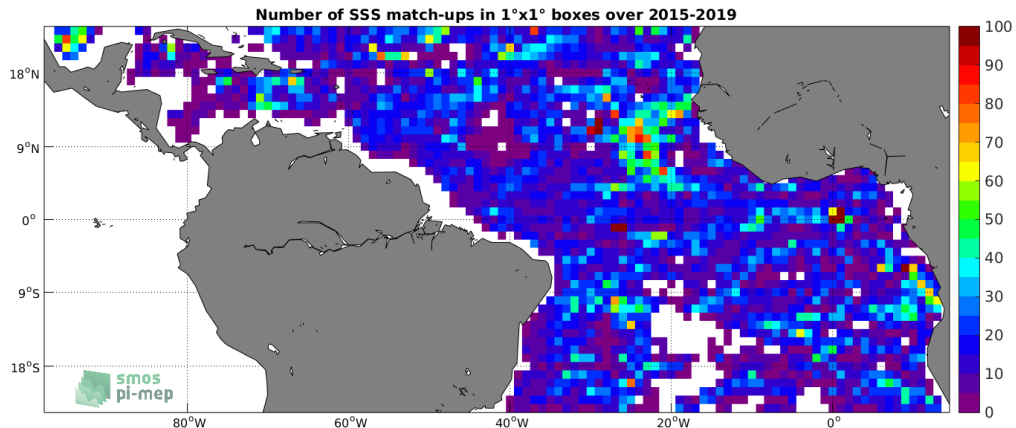
Figure 4: Number of SSS match-ups between Argo SSS and the SMAP-L3-RSS-V3-MONTHLY-0.25DEG-40KM SSS product for the Tropical Atlantic Ocean Pi-MEP region over 1^\circ \times 1^\circ boxes and for the full satellite product period.
