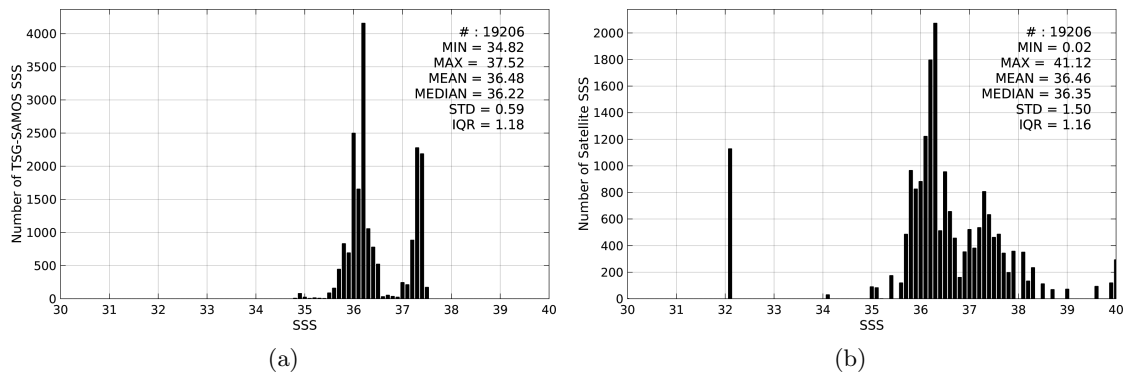
Figure 2: Histograms of SSS from TSG-SAMOS (a) and SMAP-L3-RSS-V2-8DAY-RUNNING-40KM (b) considering all match-up pairs per bins of 0.1 over the Tropical Atlantic Ocean Pi-MEP region and for the full satellite product period.
