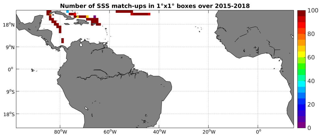
Figure 4: Number of SSS match-ups between TSG-SAMOS SSS and the SMAP-L3-RSS-V2-8DAY-RUNNING-40KM SSS product for the Tropical Atlantic Ocean Pi-MEP region over 1^\circ \times 1^\circ boxes and for the full satellite product period.
