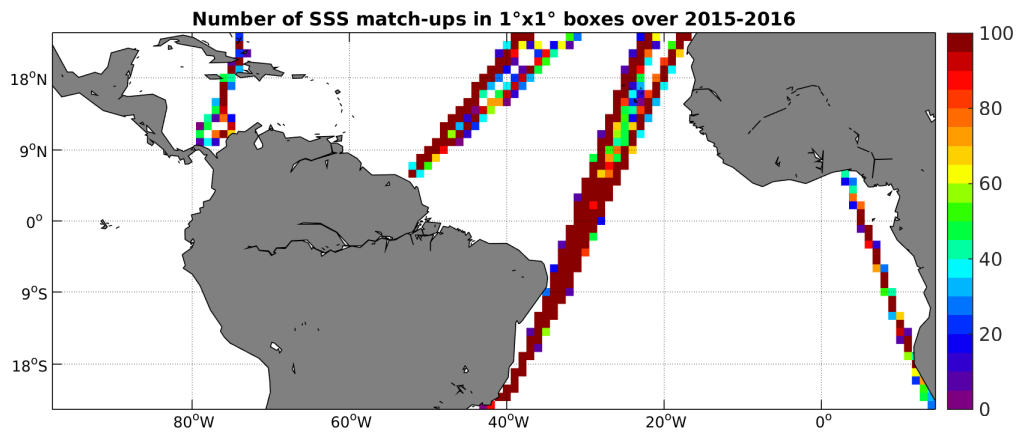
Figure 4: Number of SSS match-ups between TSG-LEGOS-DM SSS and the SMAP-L3-RSS-V2-8DAY-RUNNING-40KM SSS product for the Tropical Atlantic Ocean Pi-MEP region over 1°x1° boxes and for the full satellite product period.
