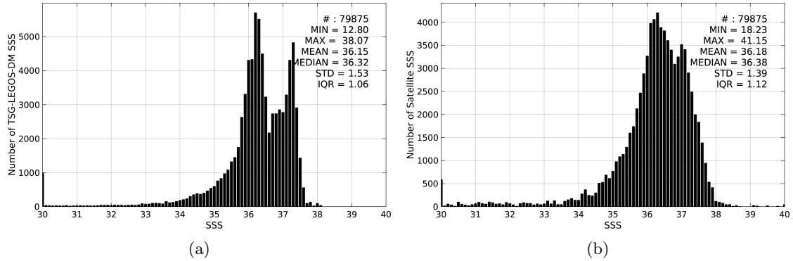
Figure 2: Histograms of SSS from TSG-LEGOS-DM (a) and SMAP-L3-RSS-V2-8DAY-RUNNING-40KM (b) considering all match-up pairs per bins of 0.1 over the Tropical Atlantic Ocean Pi-MEP region and for the full satellite product period.
