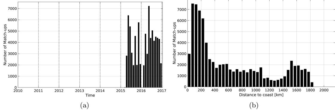
Figure 1: Number of match-ups between TSG-LEGOS-DM and SMAP-L3-RSS-V2-8DAY-RUNNING-40KM SSS as a function of time (a) and as function of the distance to coast (b) over the Tropical Atlantic Ocean Pi-MEP region and for the full satellite product period.
