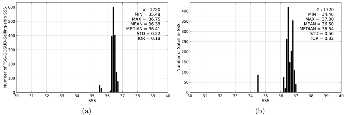
Figure 2: Histograms of SSS from TSG-GOSUD-Sailing-ship (a) and SMAP-L3-RSS-V2-8DAY-RUNNING-40KM (b) considering all match-up pairs per bins of 0.1 over the Tropical Atlantic Ocean Pi-MEP region and for the full satellite product period.
