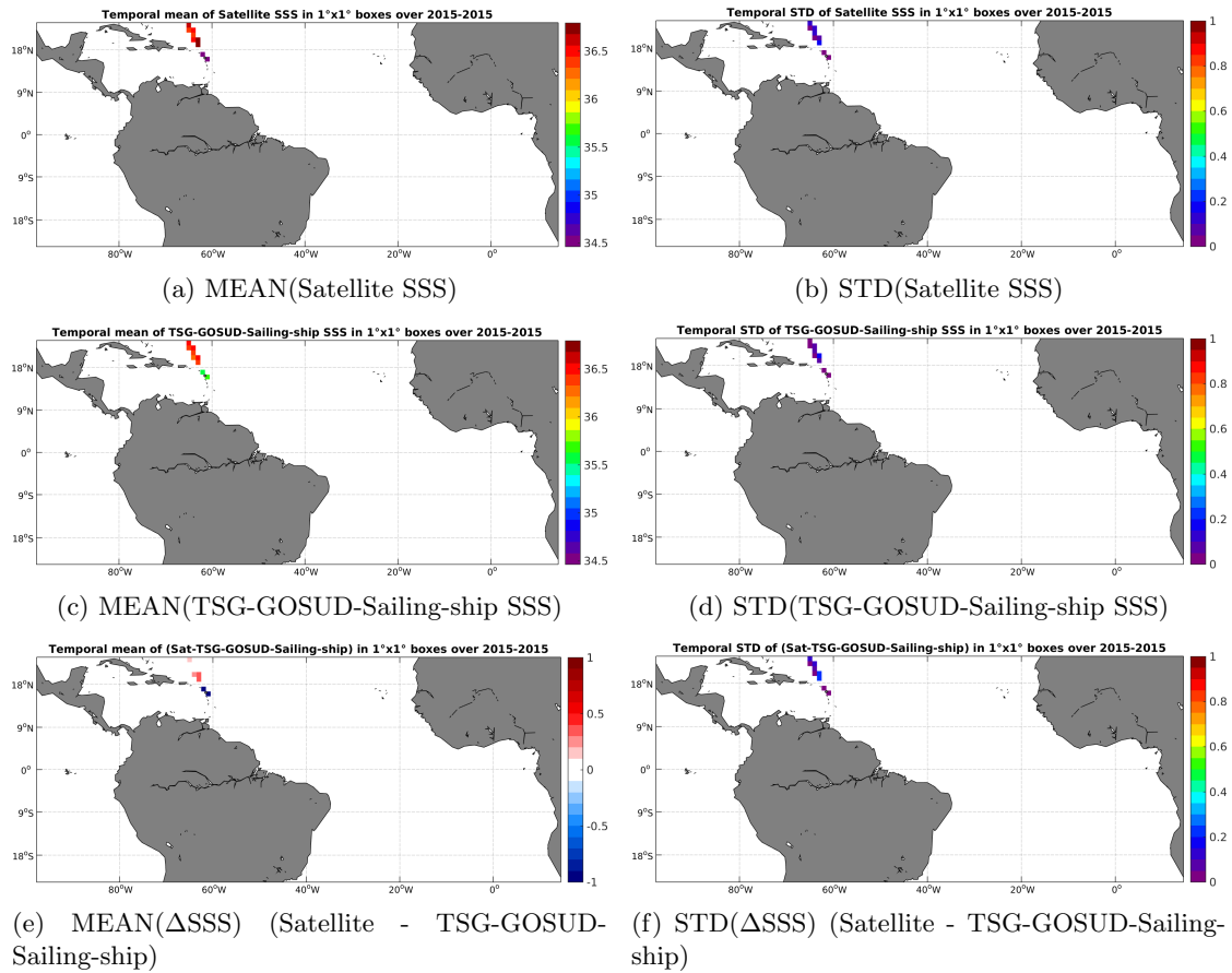
Figure 6: Temporal mean (left) and STD (right) of SSS from SMAP-L3-RSS-V2-8DAY-RUNNING-40KM (top), TSG-GOSUD-Sailing-ship (middle), and of \Delta SSS (Satellite - TSG-GOSUD-Sailing-ship). Only match-up pairs are used to generate these maps.
