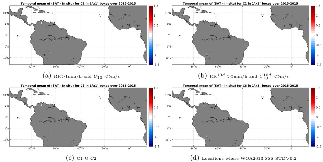
Figure 12: Temporal mean gridded over spatial boxes of size 1^\circ \times 1^\circ of \Delta SSS (SMAP-L3-RSS-V2-8DAY-RUNNING-40KM - TSG-GOSUD-Sailing-ship) for 4 different subdatasets corresponding to: RR > 1\text{mm/h} and U_{10} < 5\text{m/s} (a), RR^{10d} > 5\text{mm/h} and U_{10}^{10d} < 5\text{m/s} (b), C1 U C2 (c), Locations where WOA2013 SSS STD > 0.2 (d).
