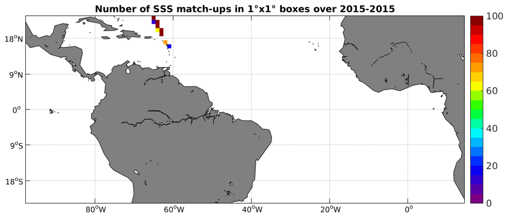
Figure 4: Number of SSS match-ups between TSG-GOSUD-Sailing-ship SSS and the SMAP-L3-RSS-V2-8DAY-RUNNING-40KM SSS product for the Tropical Atlantic Ocean Pi-MEP region over 1^\circ \times 1^\circ boxes and for the full satellite product period.
