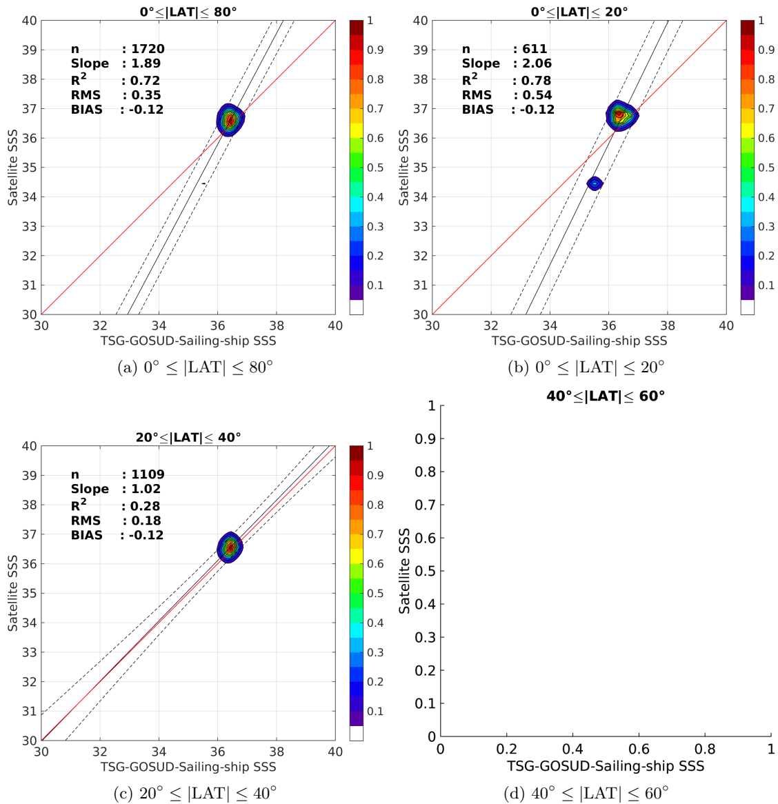
Figure 9: Contour maps of the concentration of SMAP-L3-RSS-V2-8DAY-RUNNING-40KM SSS (y-axis) versus TSG-GOSUD-Sailing-ship SSS (x-axis) at match-up pairs for different latitude bands. For each plot, the red line shows x=y . The black thin and dashed lines indicate a linear fit through the data cloud and the \pm 95\% confidence levels, respectively. The number match-up pairs n , the slope and R^2 coefficient of the linear fit, the root mean square (RMS) and the mean bias between satellite and in situ data are indicated for each latitude band in each plots.
