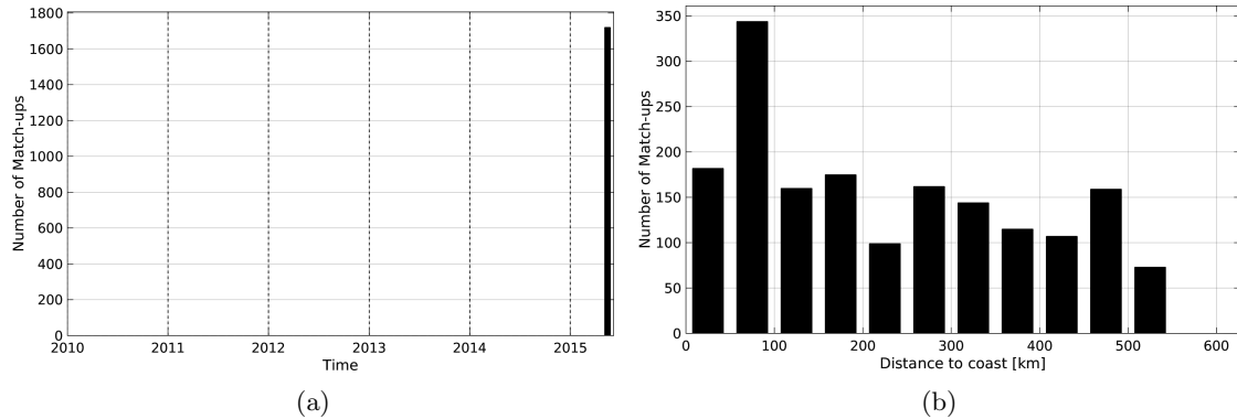
Figure 1: Number of match-ups between TSG-GOSUD-Sailing-ship and SMAP-L3-RSS-V2-8DAY-RUNNING-40KM SSS as a function of time (a) and as function of the distance to coast (b) over the Tropical Atlantic Ocean Pi-MEP region and for the full satellite product period.
