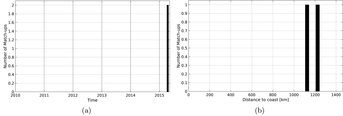
Figure 1: Number of match-ups between Surface drifters and SMAP-L3-RSS-V2-8DAY-RUNNING-40KM SSS as a function of time (a) and as function of the distance to coast (b) over the Tropical Atlantic Ocean Pi-MEP region and for the full satellite product period.
