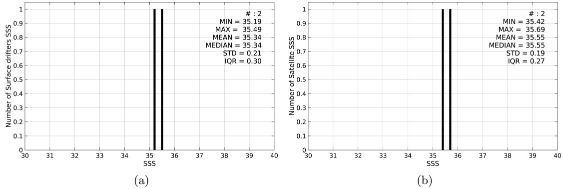
Figure 2: Histograms of SSS from Surface drifters (a) and SMAP-L3-RSS-V2-8DAY-RUNNING-40KM (b) considering all match-up pairs per bins of 0.1 over the Tropical Atlantic Ocean Pi-MEP region and for the full satellite product period.
