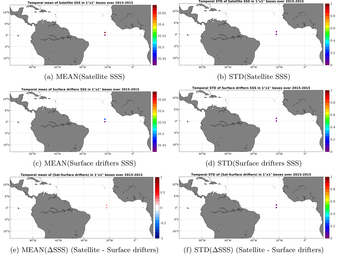
Figure 5: Temporal mean (left) and STD (right) of SSS from SMAP-L3-RSS-V2-8DAY-RUNNING-40KM (top), Surface drifters (middle), and of \Delta SSS (Satellite - Surface drifters). Only match-up pairs are used to generate these maps.
