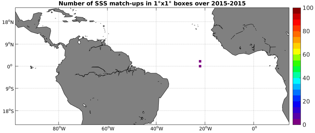
Figure 3: Number of SSS match-ups between Surface drifters SSS and the SMAP-L3-RSS-V2-8DAY-RUNNING-40KM SSS product for the Tropical Atlantic Ocean Pi-MEP region over 1^\circ \times 1^\circ boxes and for the full satellite product period.
