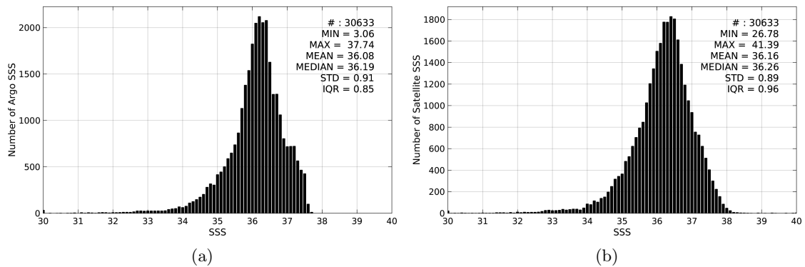
Figure 2: Histograms of SSS from Argo (a) and SMAP-L3-RSS-V2-8DAY-RUNNING-40KM (b) considering all match-up pairs per bins of 0.1 over the Tropical Atlantic Ocean Pi-MEP region and for the full satellite product period.
