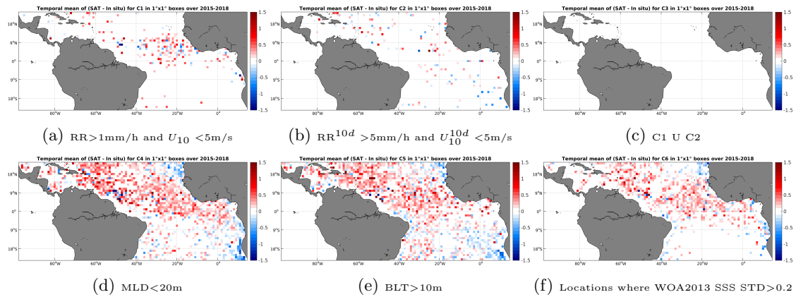
Figure 12: Temporal mean gridded over spatial boxes of size 1^\circ \times 1^\circ of \Delta SSS (SMAP-L3-RSS-V2-8DAY-RUNNING-40KM - Argo) for 6 different subdatasets corresponding to:RR >1 mm/h and U_{10} < 5 m/s (a), RR ^{10d} > 5 mm/h and U_{10}^{10d} < 5 m/s (b), C1 U C2 (c),MLD <20 m (d),BLT >10 m (e),Locations where WOA2013 SSS STD >0.2 (f).
