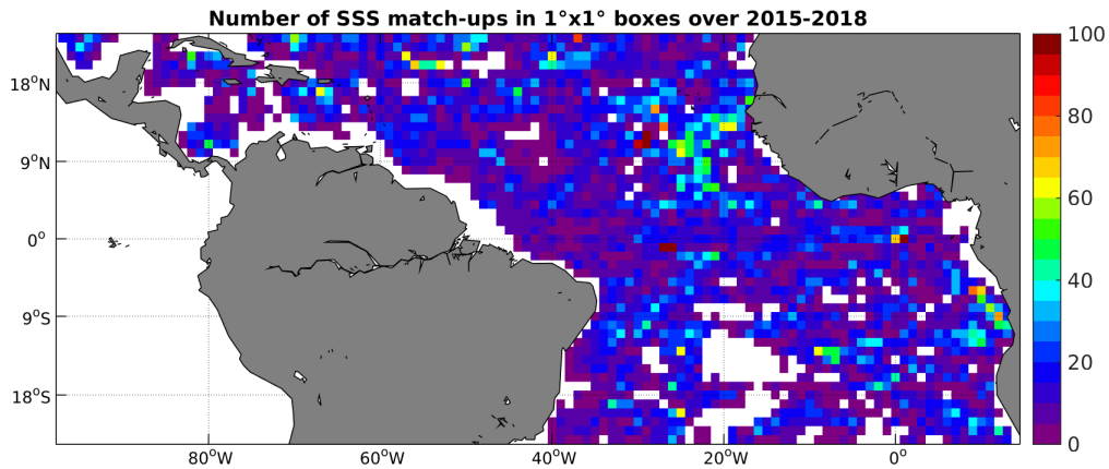
Figure 4: Number of SSS match-ups between Argo SSS and the SMAP-L3-RSS-V2-8DAY-RUNNING-40KM SSS product for the Tropical Atlantic Ocean Pi-MEP region over 1^\circ \times 1^\circ boxes and for the full satellite product period.
