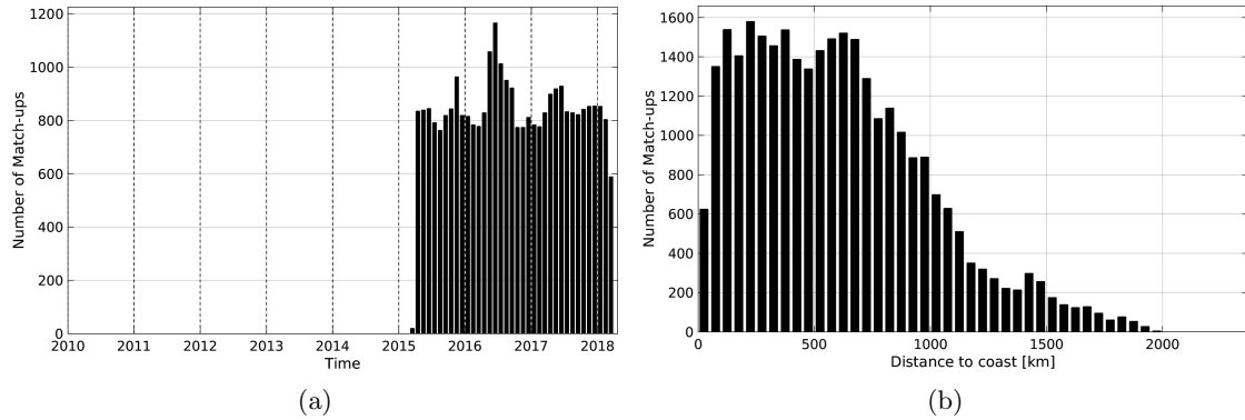
Figure 1: Number of match-ups between Argo and SMAP-L3-RSS-V2-8DAY-RUNNING-40KM SSS as a function of time (a) and as function of the distance to coast (b) over the Tropical Atlantic Ocean Pi-MEP region and for the full satellite product period.
