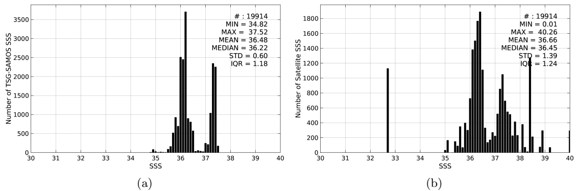
Figure 2: Histograms of SSS from TSG-SAMOS (a) and SMAP-L3-RSS-V2-MONTHLY-0.25DEG-40KM (b) considering all match-up pairs per bins of 0.1 over the Tropical Atlantic Ocean Pi-MEP region and for the full satellite product period.
