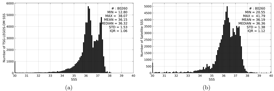
Figure 2: Histograms of SSS from TSG-LEGOS-DM (a) and SMAP-L3-RSS-V2-MONTHLY-0.25DEG-40KM (b) considering all match-up pairs per bins of 0.1 over the Tropical Atlantic Ocean Pi-MEP region and for the full satellite product period.
