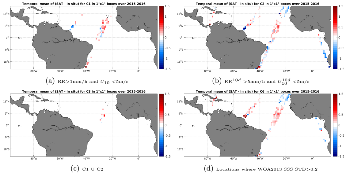
Figure 12: Temporal mean gridded over spatial boxes of size 1^\circ \times 1^\circ of \Delta SSS (SMAP-L3-RSS-V2-MONTHLY-0.25DEG-40KM - TSG-LEGOS-DM) for 4 different subdatasets corresponding to: RR > 1\text{mm/h} and U_{10} < 5\text{m/s} (a), RR^{10d} > 5\text{mm/h} and U_{10}^{10d} < 5\text{m/s} (b), C1 U C2 (c), Locations where WOA2013 SSS STD > 0.2 (d).
