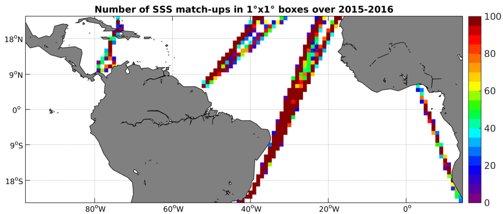
Figure 4: Number of SSS match-ups between TSG-LEGOS-DM SSS and the SMAP-L3-RSS-V2-MONTHLY-0.25DEG-40KM SSS product for the Tropical Atlantic Ocean Pi-MEP region over 1^\circ \times 1^\circ boxes and for the full satellite product period.
