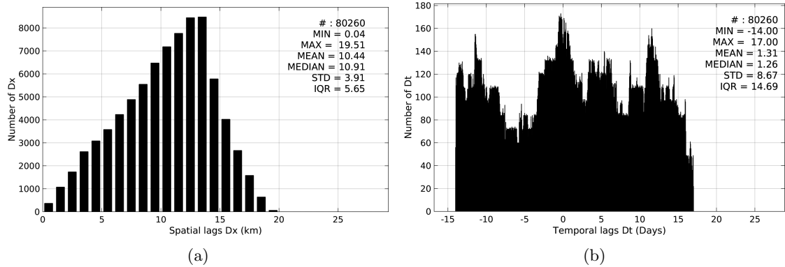
Figure 5: Histograms of the spatial (a) and temporal (b) lags between the time of the TSG-LEGOS-DM measurements and the date of the corresponding SMAP-L3-RSS-V2-MONTHLY-0.25DEG-40KM SSS product.
