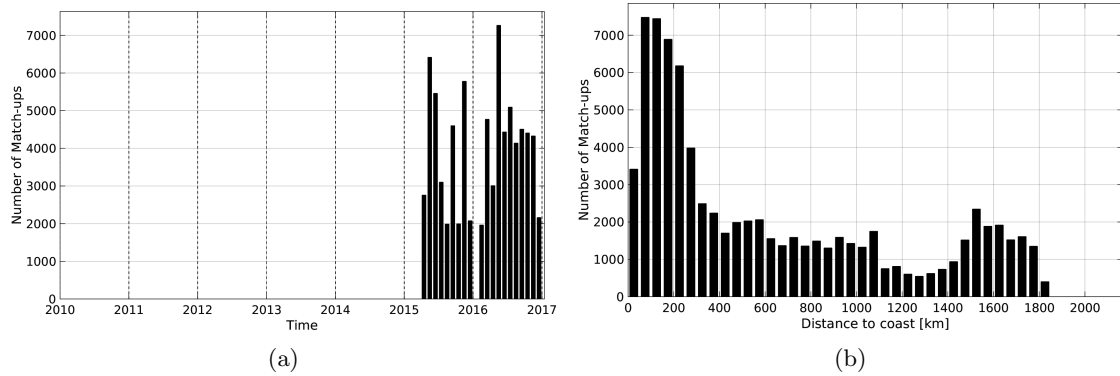
Figure 1: Number of match-ups between TSG-LEGOS-DM and SMAP-L3-RSS-V2-MONTHLY-0.25DEG-40KM SSS as a function of time (a) and as function of the distance to coast (b) over the Tropical Atlantic Ocean Pi-MEP region and for the full satellite product period.
