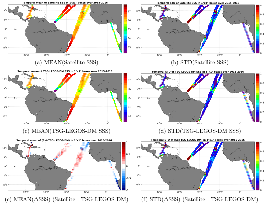
Figure 6: Temporal mean (left) and STD (right) of SSS from SMAP-L3-RSS-V2-MONTHLY-0.25DEG-40KM (top), TSG-LEGOS-DM (middle), and of \Delta SSS (Satellite - TSG-LEGOS-DM). Only match-up pairs are used to generate these maps.
