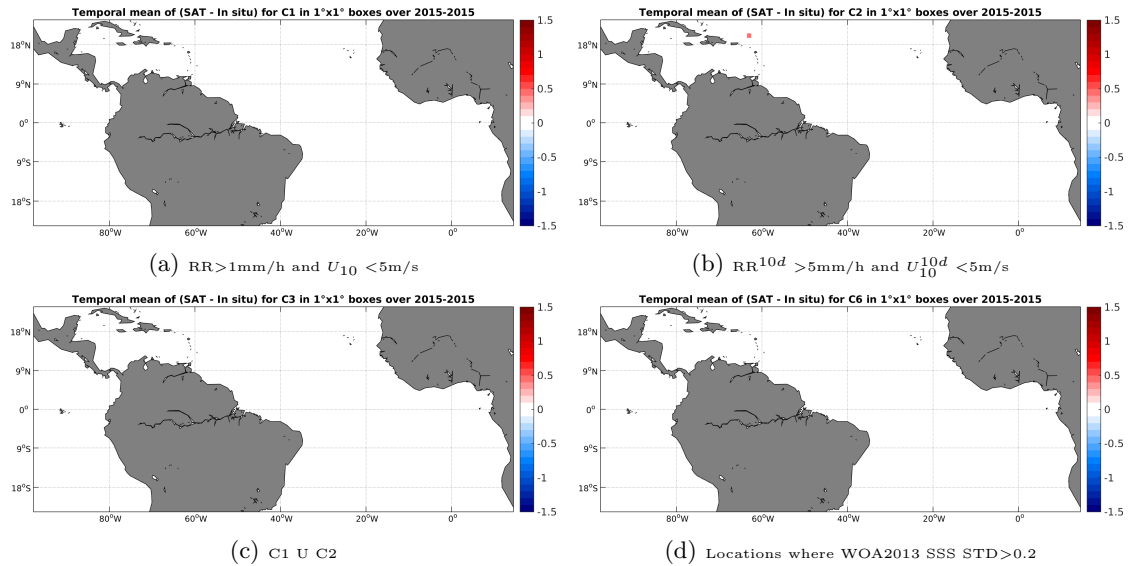
Figure 12: Temporal mean gridded over spatial boxes of size 1^\circ \times 1^\circ of \Delta SSS (SMAP-L3-RSS-V2-MONTHLY-0.25DEG-40KM - TSG-GOSUD-Sailing-ship) for 4 different subdatasets corresponding to: RR > 1mm/h and U_{10} < 5\text{m/s} (a), RR^{10d} > 5\text{mm/h} and U_{10}^{10d} < 5\text{m/s} (b), C1 U C2 (c), Locations where WOA2013 SSS STD > 0.2 (d).
