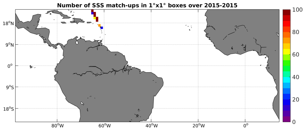
Figure 4: Number of SSS match-ups between TSG-GOSUD-Sailing-ship SSS and the SMAP-L3-RSS-V2-MONTHLY-0.25DEG-40KM SSS product for the Tropical Atlantic Ocean Pi-MEP region over 1^{\circ} \times 1^{\circ} boxes and for the full satellite product period.
