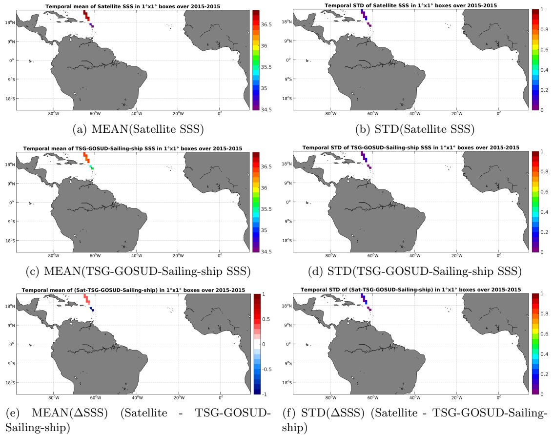
Figure 6: Temporal mean (left) and STD (right) of SSS from SMAP-L3-RSS-V2-MONTHLY-0.25DEG-40KM (top), TSG-GOSUD-Sailing-ship (middle), and of \Delta SSS (Satellite - TSG-GOSUD-Sailing-ship). Only match-up pairs are used to generate these maps.
