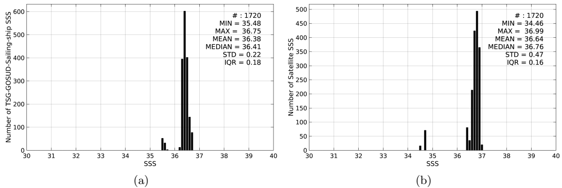
Figure 2: Histograms of SSS from TSG-GOSUD-Sailing-ship (a) and SMAP-L3-RSS-V2-MONTHLY-0.25DEG-40KM (b) considering all match-up pairs per bins of 0.1 over the Tropical Atlantic Ocean Pi-MEP region and for the full satellite product period.
