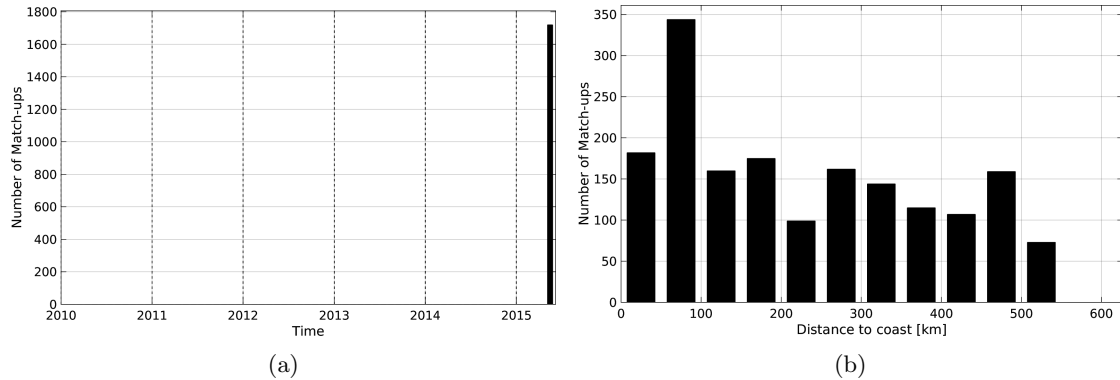
Figure 1: Number of match-ups between TSG-GOSUD-Sailing-ship and SMAP-L3-RSS-V2-MONTHLY-0.25DEG-40KM SSS as a function of time (a) and as function of the distance to coast (b) over the Tropical Atlantic Ocean Pi-MEP region and for the full satellite product period.
