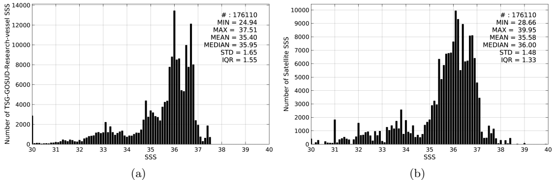
Figure 2: Histograms of SSS from TSG-GOSUD-Research-vessel (a) and SMAP-L3-RSS-V2-MONTHLY-0.25DEG-40KM (b) considering all match-up pairs per bins of 0.1 over the Tropical Atlantic Ocean Pi-MEP region and for the full satellite product period.
