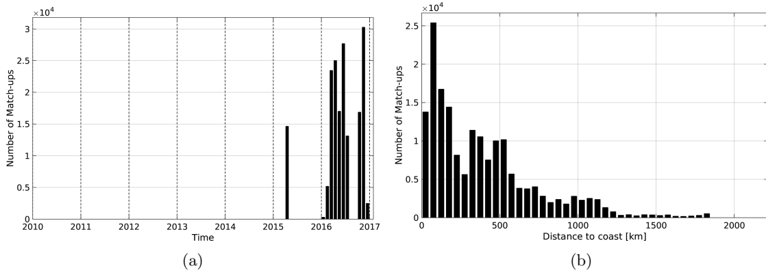
Figure 1: Number of match-ups between TSG-GOSUD-Research-vessel and SMAP-L3-RSS-V2-MONTHLY-0.25DEG-40KM SSS as a function of time (a) and as function of the distance to coast (b) over the Tropical Atlantic Ocean Pi-MEP region and for the full satellite product period.
