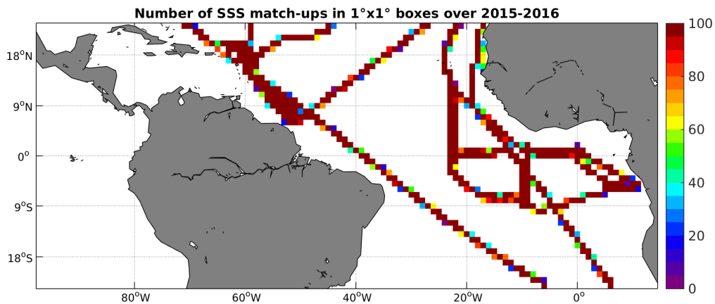
Figure 4: Number of SSS match-ups between TSG-GOSUD-Research-vessel SSS and the SMAP-L3-RSS-V2-MONTHLY-0.25DEG-40KM SSS product for the Tropical Atlantic Ocean Pi-MEP region over 1^\circ \times 1^\circ boxes and for the full satellite product period.
