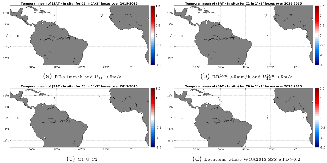
Figure 11: Temporal mean gridded over spatial boxes of size 1^\circ \times 1^\circ of \Delta SSS (SMAP-L3-RSS-V2-MONTHLY-0.25DEG-40KM - Surface drifters) for 4 different subdatasets corresponding to: RR > 1mm/h and U_{10} < 5\text{m/s} (a), RR^{10d} > 5\text{mm/h} and U_{10}^{10d} < 5\text{m/s} (b), C1 U C2 (c), Locations where WOA2013 SSS STD > 0.2 (d).
