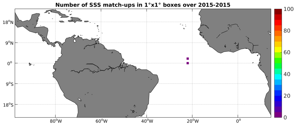
Figure 3: Number of SSS match-ups between Surface drifters SSS and the SMAP-L3-RSS-V2-MONTHLY-0.25DEG-40KM SSS product for the Tropical Atlantic Ocean Pi-MEP region over 1^\circ \times 1^\circ boxes and for the full satellite product period.
