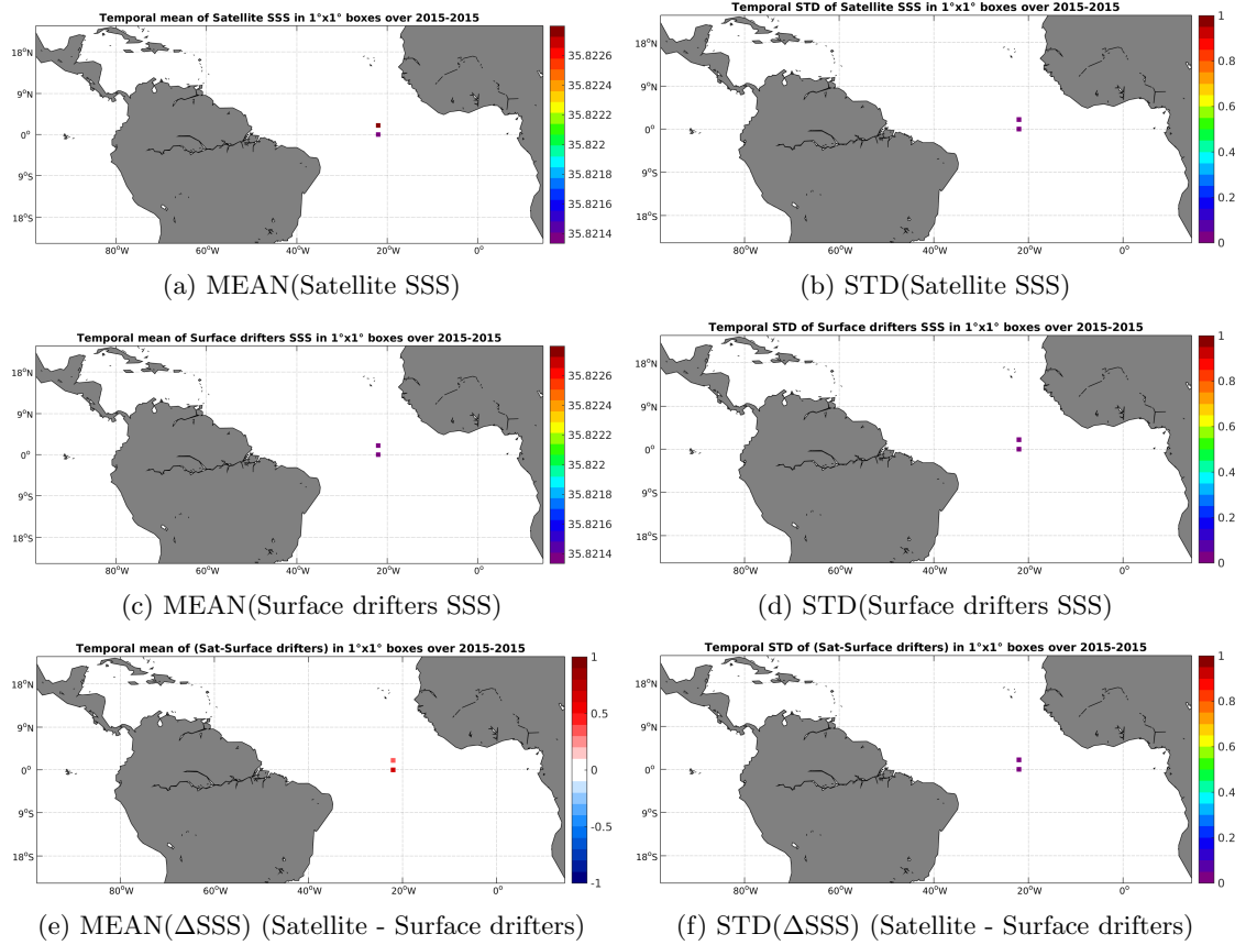
Figure 5: Temporal mean (left) and STD (right) of SSS from SMAP-L3-RSS-V2-MONTHLY-0.25DEG-40KM (top), Surface drifters (middle), and of \Delta SSS (Satellite - Surface drifters). Only match-up pairs are used to generate these maps.
