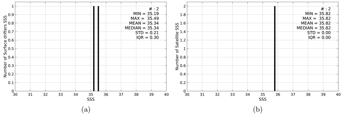
Figure 2: Histograms of SSS from Surface drifters (a) and SMAP-L3-RSS-V2-MONTHLY-0.25DEG-40KM (b) considering all match-up pairs per bins of 0.1 over the Tropical Atlantic Ocean Pi-MEP region and for the full satellite product period.
