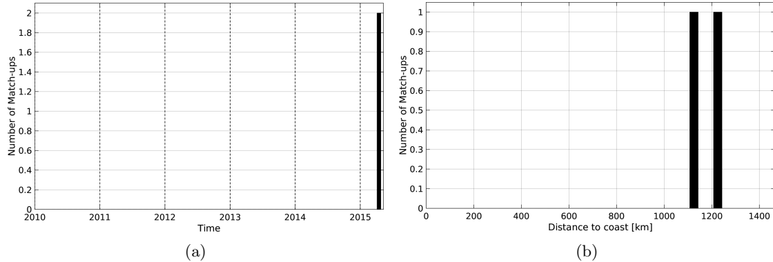
Figure 1: Number of match-ups between Surface drifters and SMAP-L3-RSS-V2-MONTHLY-0.25DEG-40KM SSS as a function of time (a) and as function of the distance to coast (b) over the Tropical Atlantic Ocean Pi-MEP region and for the full satellite product period.
