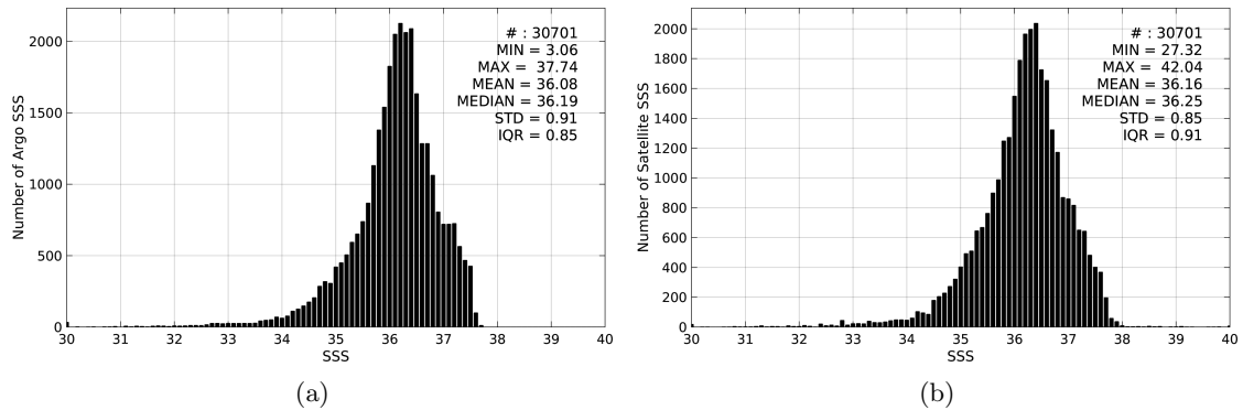
Figure 2: Histograms of SSS from Argo (a) and SMAP-L3-RSS-V2-MONTHLY-0.25DEG-40KM (b) considering all match-up pairs per bins of 0.1 over the Tropical Atlantic Ocean Pi-MEP region and for the full satellite product period.
