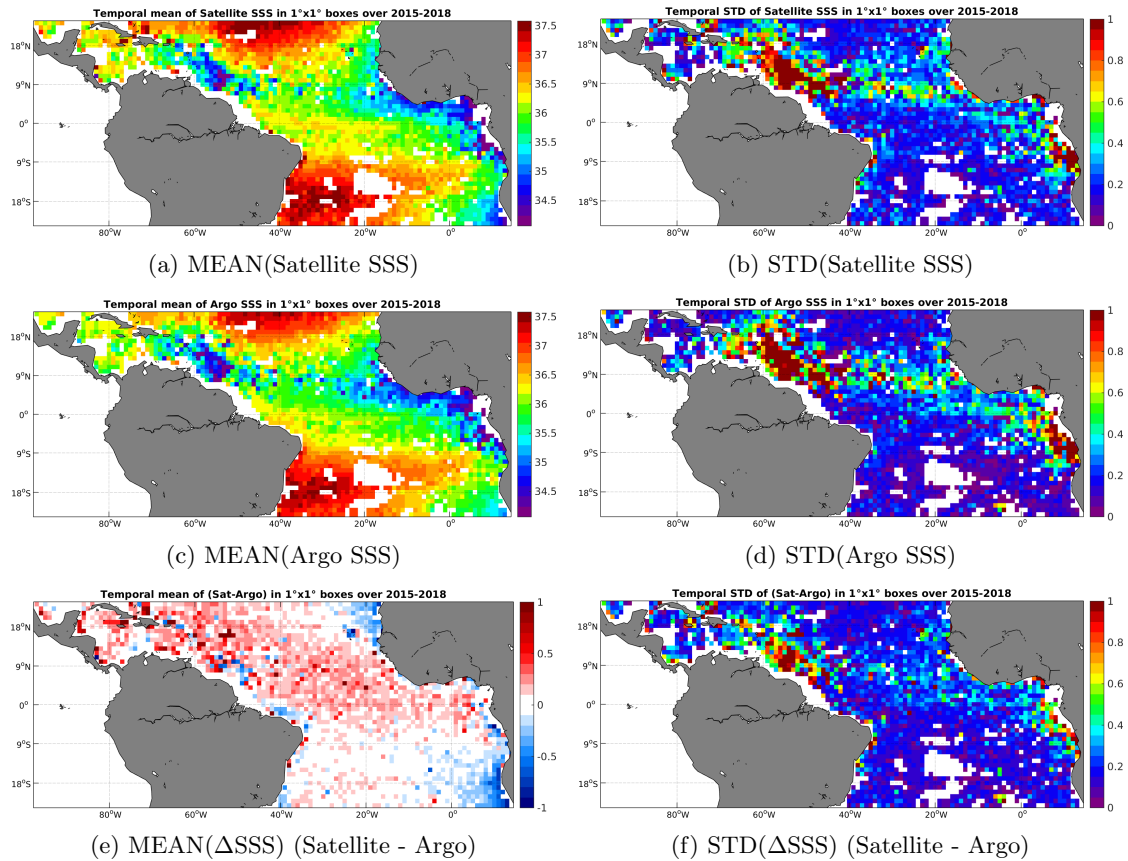
Figure 6: Temporal mean (left) and STD (right) of SSS from SMAP-L3-RSS-V2-MONTHLY-0.25DEG-40KM (top), Argo (middle), and of \Delta SSS (Satellite - Argo). Only match-up pairs are used to generate these maps.
