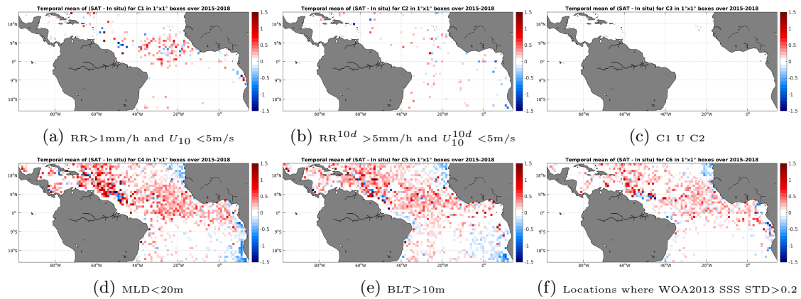
Figure 12: Temporal mean gridded over spatial boxes of size 1^\circ \times 1^\circ of \Delta SSS (SMAP-L3-RSS-V2-MONTHLY-0.25DEG-40KM - Argo) for 6 different subdatasets corresponding to:RR > 1mm/h and U_{10} < 5 m/s (a), RR^{10d} > 5 mm/h and U_{10}^{10d} < 5 m/s (b), C1 U C2 (c),MLD < 20m (d),BLT > 10m (e),Locations where WOA2013 SSS STD > 0.2 (f).
