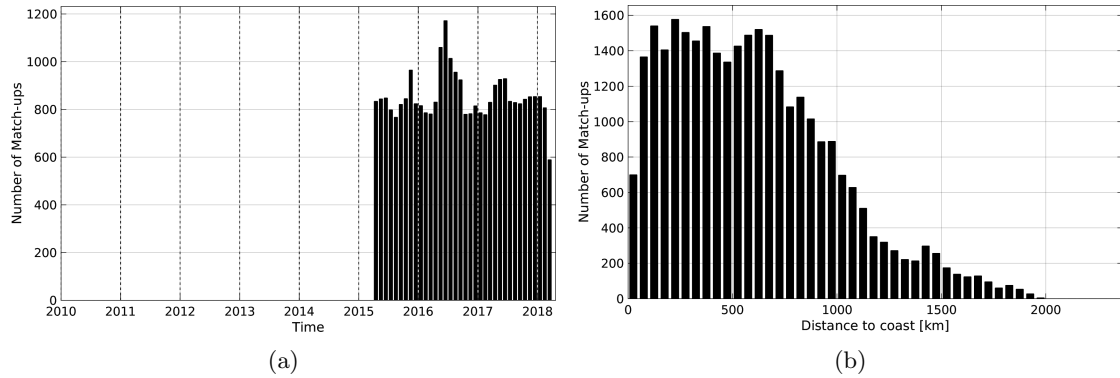
Figure 1: Number of match-ups between Argo and SMAP-L3-RSS-V2-MONTHLY-0.25DEG-40KM SSS as a function of time (a) and as function of the distance to coast (b) over the Tropical Atlantic Ocean Pi-MEP region and for the full satellite product period.
