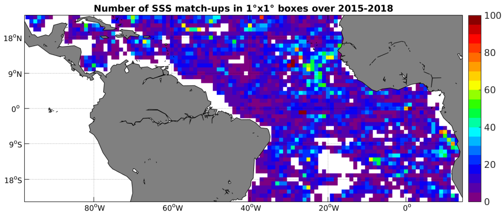
Figure 4: Number of SSS match-ups between Argo SSS and the SMAP-L3-RSS-V2-MONTHLY-0.25DEG-40KM SSS product for the Tropical Atlantic Ocean Pi-MEP region over 1^\circ \times 1^\circ boxes and for the full satellite product period.
