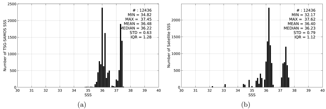
Figure 2: Histograms of SSS from TSG-SAMOS (a) and SMAP-L3-RSS-V2-MONTHLY-70KM (b) considering all match-up pairs per bins of 0.1 over the Tropical Atlantic Ocean Pi-MEP region and for the full satellite product period.
