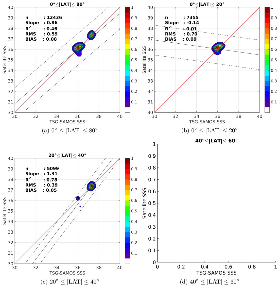
Figure 9: Contour maps of the concentration of SMAP-L3-RSS-V2-MONTHLY-70KM SSS (y-axis) versus TSG-SAMOS SSS (x-axis) at match-up pairs for different latitude bands. For each plot, the red line shows x=y . The black thin and dashed lines indicate a linear fit through the data cloud and the \pm 95\% confidence levels, respectively. The number match-up pairs n , the slope and R^2 coefficient of the linear fit, the root mean square (RMS) and the mean bias between satellite and in situ data are indicated for each latitude band in each plots.
