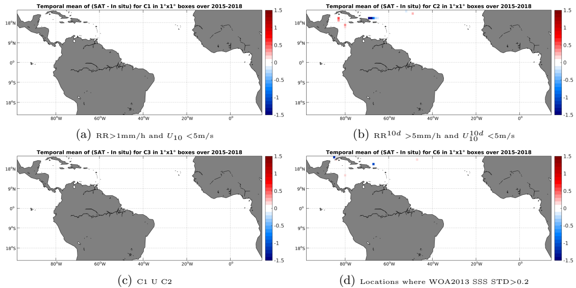
Figure 12: Temporal mean gridded over spatial boxes of size 1^\circ \times 1^\circ of \Delta SSS (SMAP-L3-RSS-V2-MONTHLY-70KM - TSG-SAMOS) for 4 different subdatasets corresponding to: RR > 1\text{mm/h} and U_{10} < 5\text{m/s} (a), RR^{10d} > 5\text{mm/h} and U_{10}^{10d} < 5\text{m/s} (b), C1 U C2 (c), Locations where WOA2013 SSS STD > 0.2 (d).
