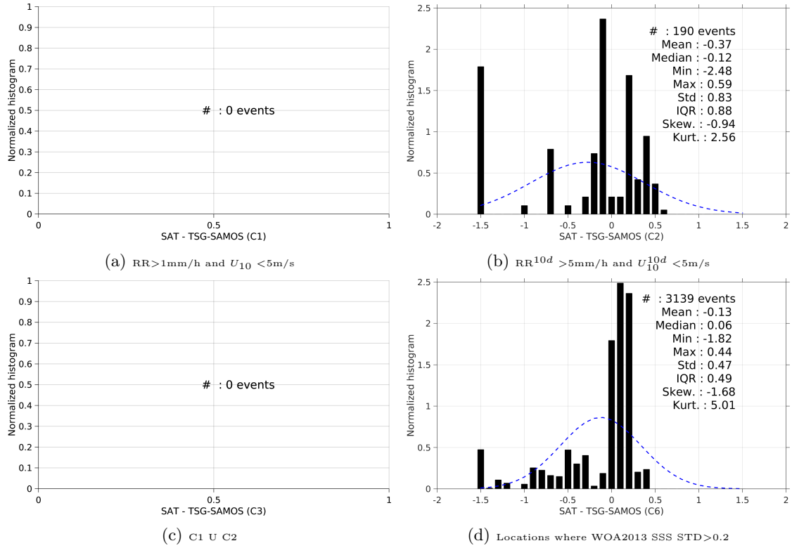
Figure 13: Normalized histogram of \Delta\text{SSS} (SMAP-L3-RSS-V2-MONTHLY-70KM - TSG-SAMOS) for 6 different subdatasets corresponding to: RR > 1\text{mm/h} and U_{10} < 5\text{m/s} (a), RR^{10d} > 5\text{mm/h} and U_{10}^{10d} < 5\text{m/s} (b), C1 \cup C2 (c), Locations where WOA2013 SSS STD > 0.2 (d).
