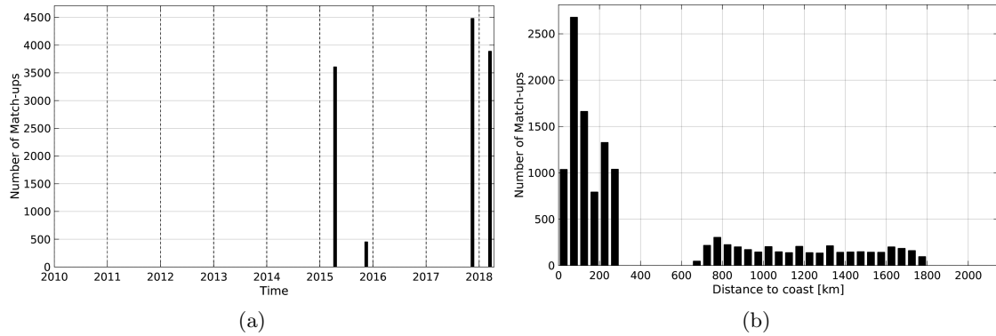
Figure 1: Number of match-ups between TSG-SAMOS and SMAP-L3-RSS-V2-MONTHLY-70KM SSS as a function of time (a) and as function of the distance to coast (b) over the Tropical Atlantic Ocean Pi-MEP region and for the full satellite product period.
