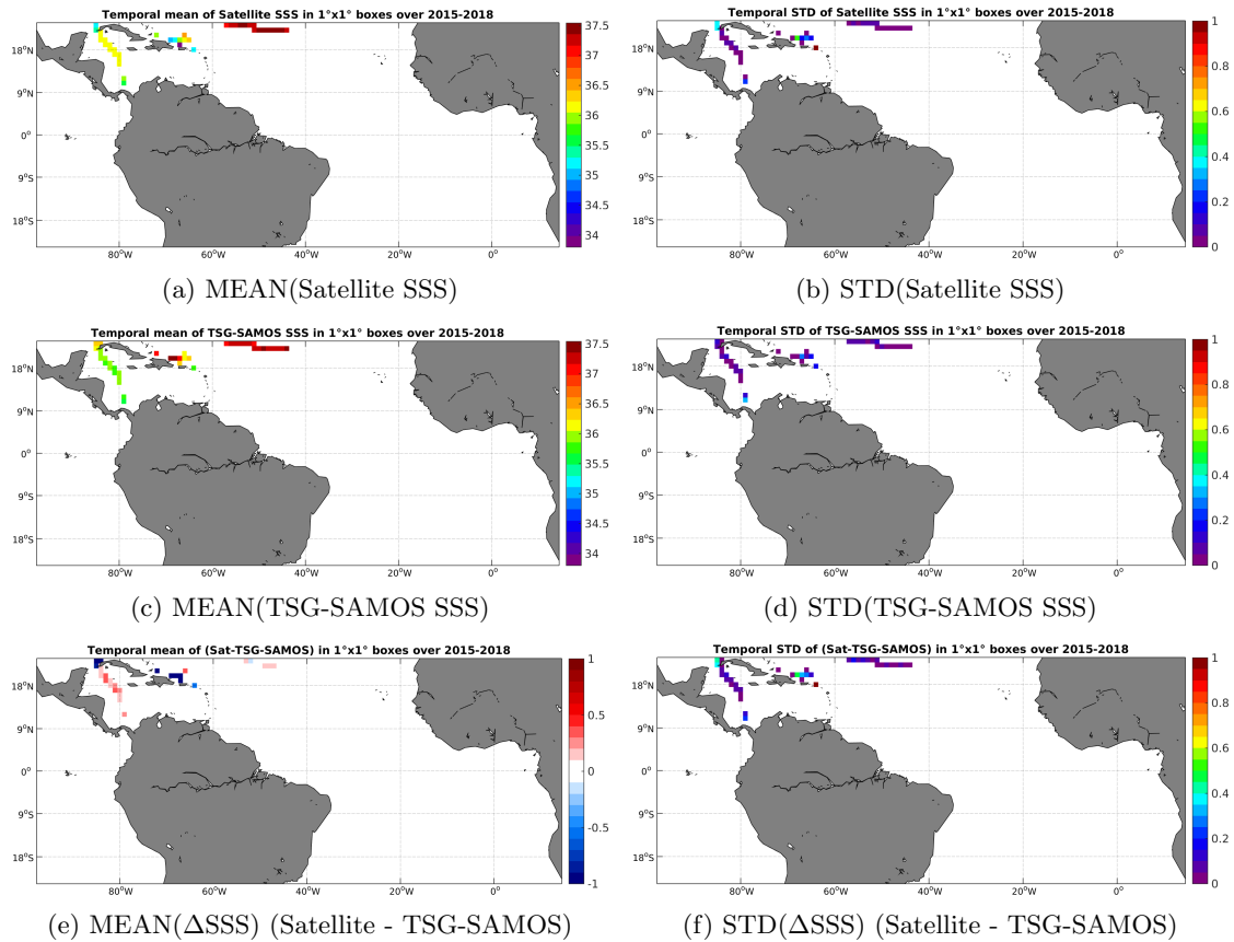
Figure 6: Temporal mean (left) and STD (right) of SSS from SMAP-L3-RSS-V2-MONTHLY-70KM (top), TSG-SAMOS (middle), and of \Delta SSS (Satellite - TSG-SAMOS). Only match-up pairs are used to generate these maps.
