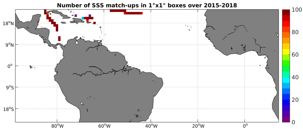
Figure 4: Number of SSS match-ups between TSG-SAMOS SSS and the SMAP-L3-RSS-V2-MONTHLY-70KM SSS product for the Tropical Atlantic Ocean Pi-MEP region over 1^\circ \times 1^\circ boxes and for the full satellite product period.
