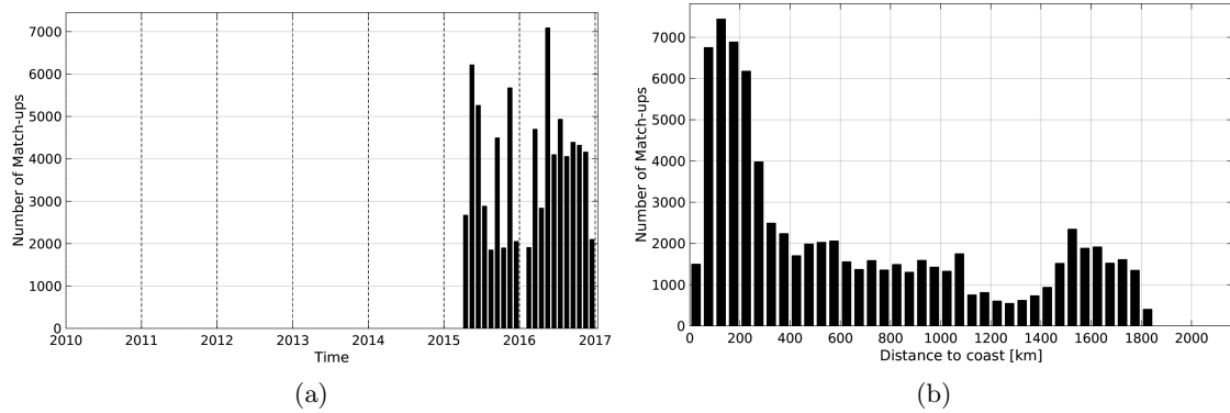
Figure 1: Number of match-ups between TSG-LEGOS-DM and SMAP-L3-RSS-V2-MONTHLY-70KM SSS as a function of time (a) and as function of the distance to coast (b) over the Tropical Atlantic Ocean Pi-MEP region and for the full satellite product period.
