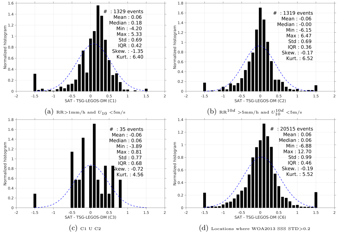
Figure 13: Normalized histogram of \Delta SSS (SMAP-L3-RSS-V2-MONTHLY-70KM - TSG-LEGOS-DM) for 6 different subdatasets corresponding to: RR > 1mm/h and U_{10} < 5 m/s (a), RR^{10d} > 5 mm/h and U_{10}^{10d} < 5 m/s (b), C1 U C2 (c), Locations where WOA2013 SSS STD > 0.2 (d).
