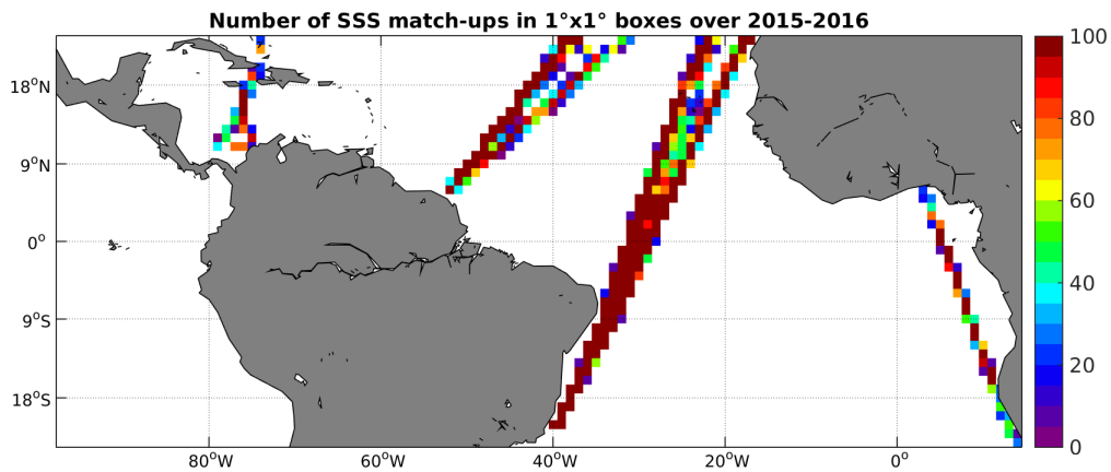
Figure 4: Number of SSS match-ups between TSG-LEGOS-DM SSS and the SMAP-L3-RSS-V2-MONTHLY-70KM SSS product for the Tropical Atlantic Ocean Pi-MEP region over 1^\circ \times 1^\circ boxes and for the full satellite product period.
