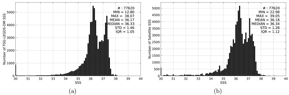
Figure 2: Histograms of SSS from TSG-LEGOS-DM (a) and SMAP-L3-RSS-V2-MONTHLY-70KM (b) considering all match-up pairs per bins of 0.1 over the Tropical Atlantic Ocean Pi-MEP region and for the full satellite product period.
