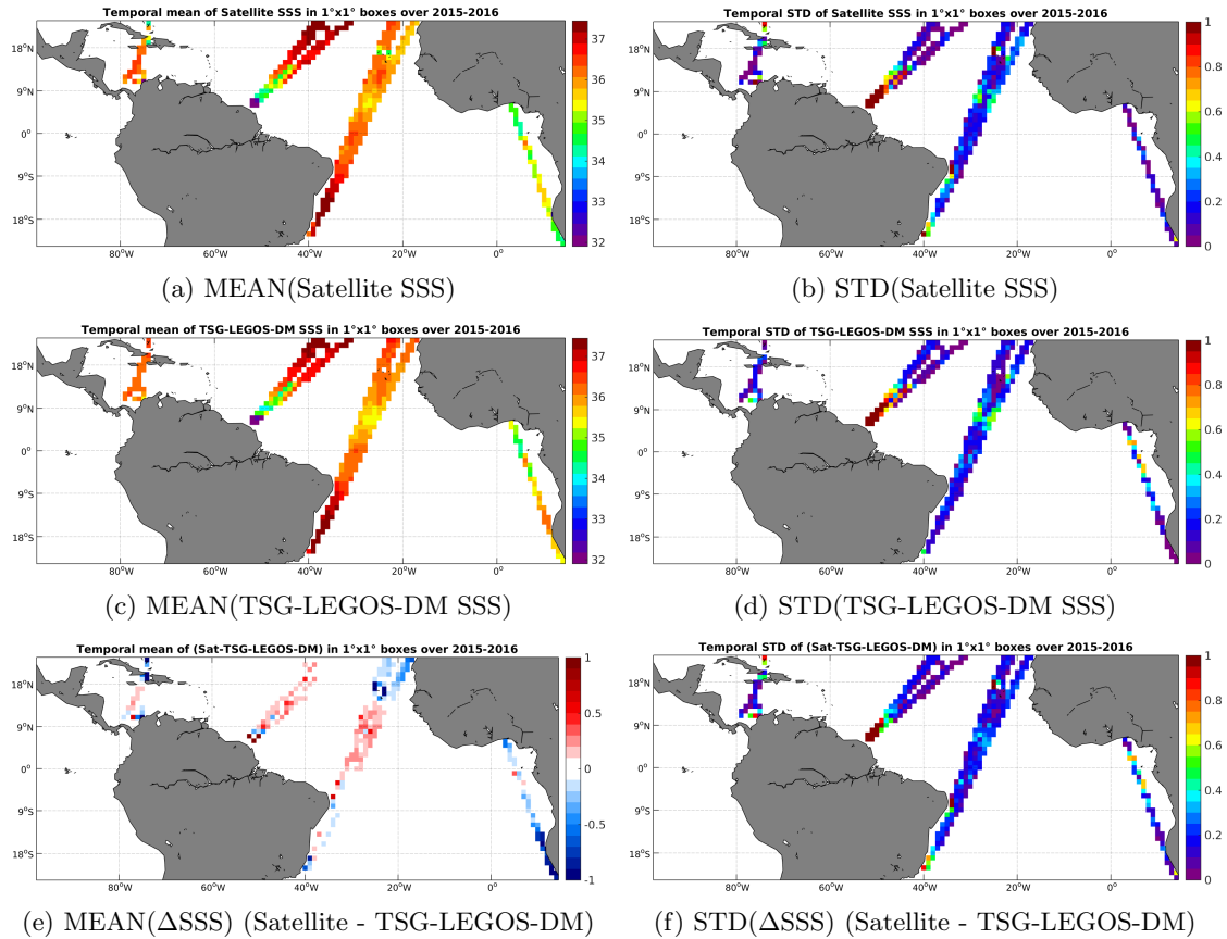
Figure 6: Temporal mean (left) and STD (right) of SSS from SMAP-L3-RSS-V2-MONTHLY-70KM (top), TSG-LEGOS-DM (middle), and of \Delta SSS (Satellite - TSG-LEGOS-DM). Only match-up pairs are used to generate these maps.
