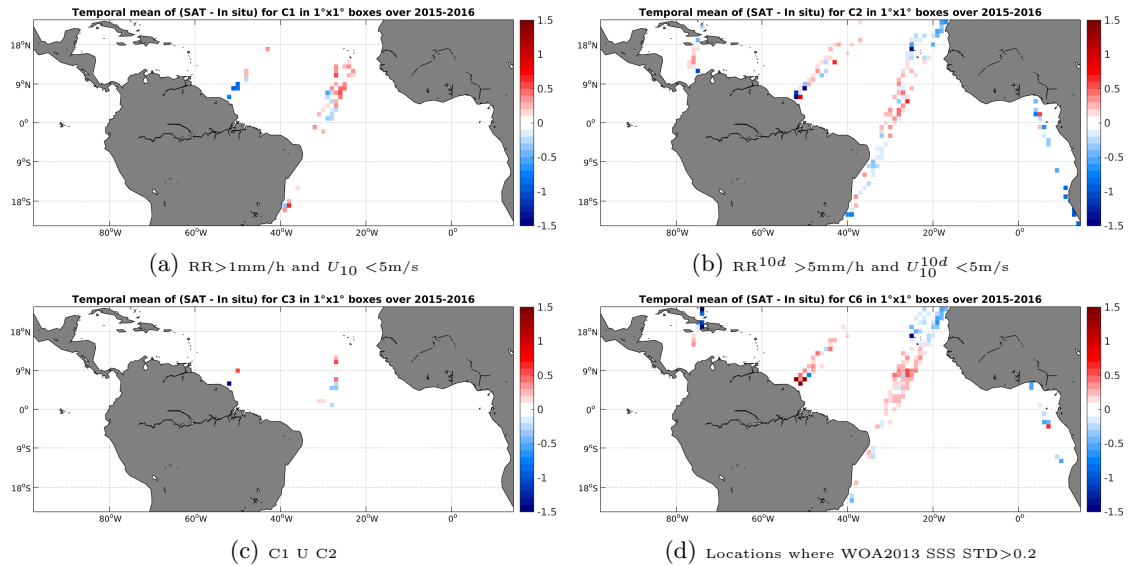
Figure 12: Temporal mean gridded over spatial boxes of size 1^\circ \times 1^\circ of \Delta SSS (SMAP-L3-RSS-V2-MONTHLY-70KM - TSG-LEGOS-DM) for 4 different subdatasets corresponding to:RR>1mm/h and U_{10} < 5 m/s (a), RR^{10d} > 5 mm/h and U_{10}^{10d} < 5 m/s (b), C1 U C2 (c),Locations where WOA2013 SSS STD>0.2 (d).
