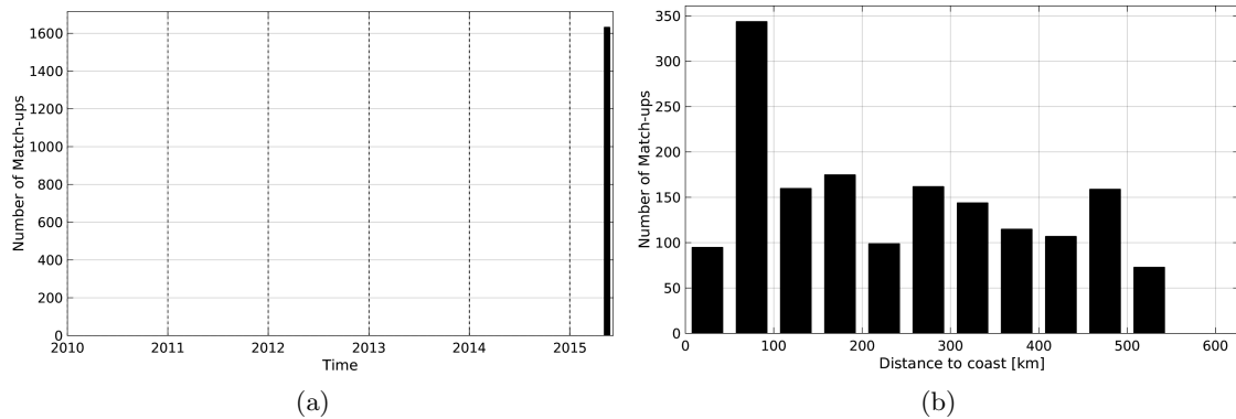
Figure 1: Number of match-ups between TSG-GOSUD-Sailing-ship and SMAP-L3-RSS-V2-MONTHLY-70KM SSS as a function of time (a) and as function of the distance to coast (b) over the Tropical Atlantic Ocean Pi-MEP region and for the full satellite product period.
