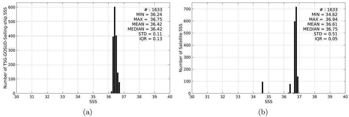
Figure 2: Histograms of SSS from TSG-GOSUD-Sailing-ship (a) and SMAP-L3-RSS-V2-MONTHLY-70KM (b) considering all match-up pairs per bins of 0.1 over the Tropical Atlantic Ocean Pi-MEP region and for the full satellite product period.
