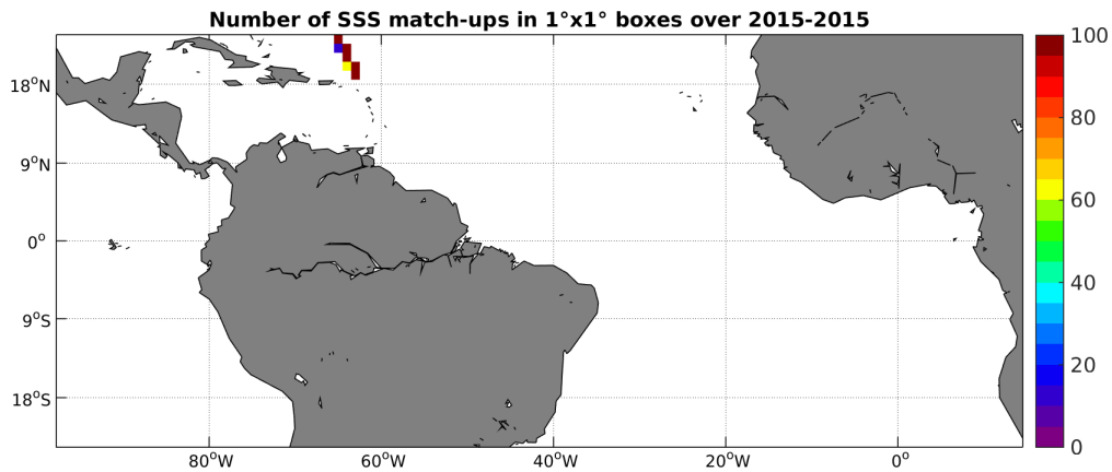
Figure 4: Number of SSS match-ups between TSG-GOSUD-Sailing-ship SSS and the SMAP-L3-RSS-V2-MONTHLY-70KM SSS product for the Tropical Atlantic Ocean Pi-MEP region over 1^\circ \times 1^\circ boxes and for the full satellite product period.
