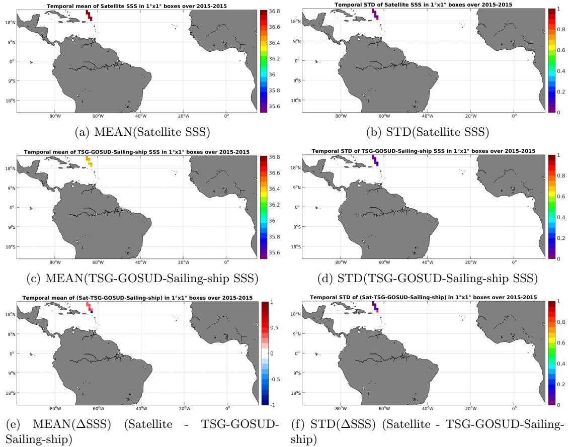
Figure 6: Temporal mean (left) and STD (right) of SSS from SMAP-L3-RSS-V2-MONTHLY-70KM (top), TSG-GOSUD-Sailing-ship (middle), and of \Delta SSS (Satellite - TSG-GOSUD-Sailing-ship). Only match-up pairs are used to generate these maps.
