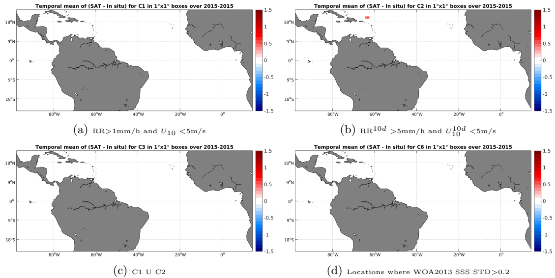
Figure 12: Temporal mean gridded over spatial boxes of size 1^\circ \times 1^\circ of \Delta SSS (SMAP-L3-RSS-V2-MONTHLY-70KM - TSG-GOSUD-Sailing-ship) for 4 different subdatasets corresponding to: RR > 1\text{mm/h} and U_{10} < 5\text{m/s} (a), RR^{10d} > 5\text{mm/h} and U_{10}^{10d} < 5\text{m/s} (b), C1 U C2 (c), Locations where WOA2013 SSS STD > 0.2 (d).
