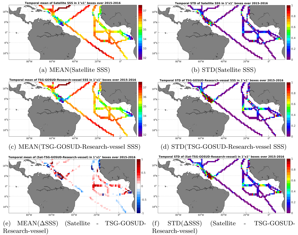
Figure 6: Temporal mean (left) and STD (right) of SSS from SMAP-L3-RSS-V2-MONTHLY-70KM (top), TSG-GOSUD-Research-vessel (middle), and of \Delta SSS (Satellite - TSG-GOSUD-Research-vessel). Only match-up pairs are used to generate these maps.
