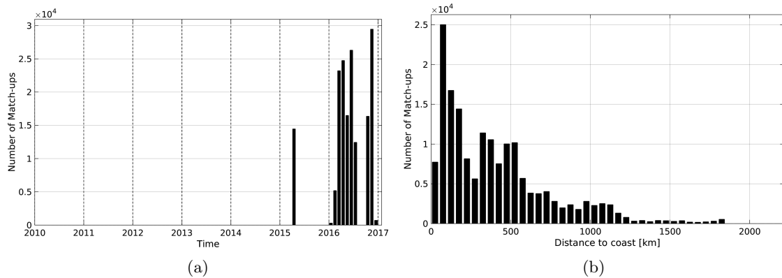
Figure 1: Number of match-ups between TSG-GOSUD-Research-vessel and SMAP-L3-RSS-V2-MONTHLY-70KM SSS as a function of time (a) and as function of the distance to coast (b) over the Tropical Atlantic Ocean Pi-MEP region and for the full satellite product period.
