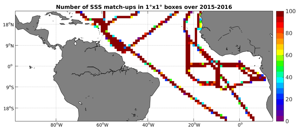
Figure 4: Number of SSS match-ups between TSG-GOSUD-Research-vessel SSS and the SMAP-L3-RSS-V2-MONTHLY-70KM SSS product for the Tropical Atlantic Ocean Pi-MEP region over 1^\circ \times 1^\circ boxes and for the full satellite product period.
