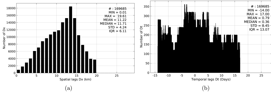
Figure 5: Histograms of the spatial (a) and temporal (b) lags between the time of the TSG-GOSUD-Research-vessel measurements and the date of the corresponding SMAP-L3-RSS-V2-MONTHLY-70KM SSS product.
