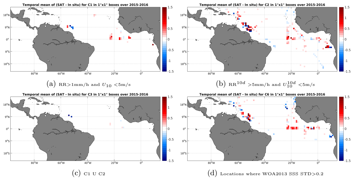
Figure 12: Temporal mean gridded over spatial boxes of size 1^\circ \times 1^\circ of \Delta SSS (SMAP-L3-RSS-V2-MONTHLY-70KM - TSG-GOSUD-Research-vessel) for 4 different subdatasets corresponding to:RR >1 mm/h and U_{10} < 5 m/s (a), RR^{10d} > 5 mm/h and U_{10}^{10d} < 5 m/s (b), C1 U C2 (c),Locations where WOA2013 SSS STD >0.2 (d).
