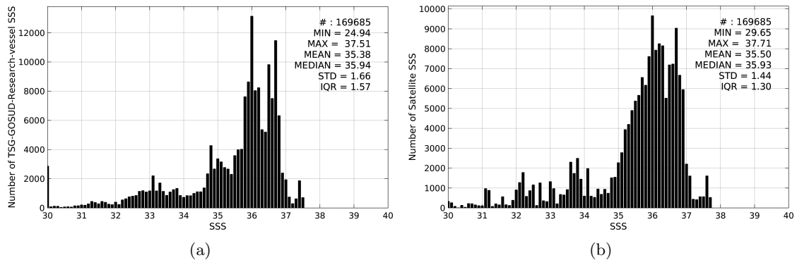
Figure 2: Histograms of SSS from TSG-GOSUD-Research-vessel (a) and SMAP-L3-RSS-V2-MONTHLY-70KM (b) considering all match-up pairs per bins of 0.1 over the Tropical Atlantic Ocean Pi-MEP region and for the full satellite product period.
