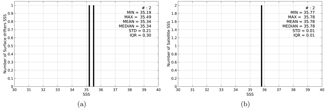
Figure 2: Histograms of SSS from Surface drifters (a) and SMAP-L3-RSS-V2-MONTHLY-70KM (b) considering all match-up pairs per bins of 0.1 over the Tropical Atlantic Ocean Pi-MEP region and for the full satellite product period.
