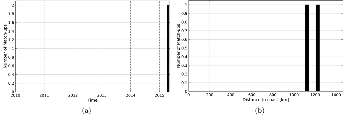
Figure 1: Number of match-ups between Surface drifters and SMAP-L3-RSS-V2-MONTHLY-70KM SSS as a function of time (a) and as function of the distance to coast (b) over the Tropical Atlantic Ocean Pi-MEP region and for the full satellite product period.
