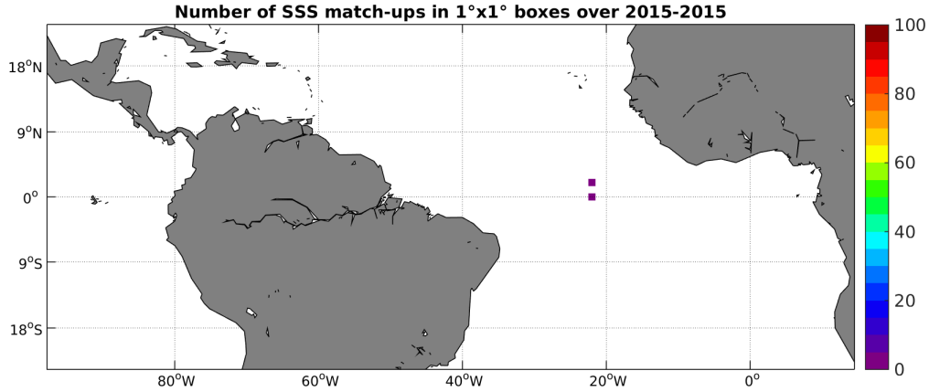
Figure 3: Number of SSS match-ups between Surface drifters SSS and the SMAP-L3-RSS-V2-MONTHLY-70KM SSS product for the Tropical Atlantic Ocean Pi-MEP region over 1^\circ \times 1^\circ boxes and for the full satellite product period.
