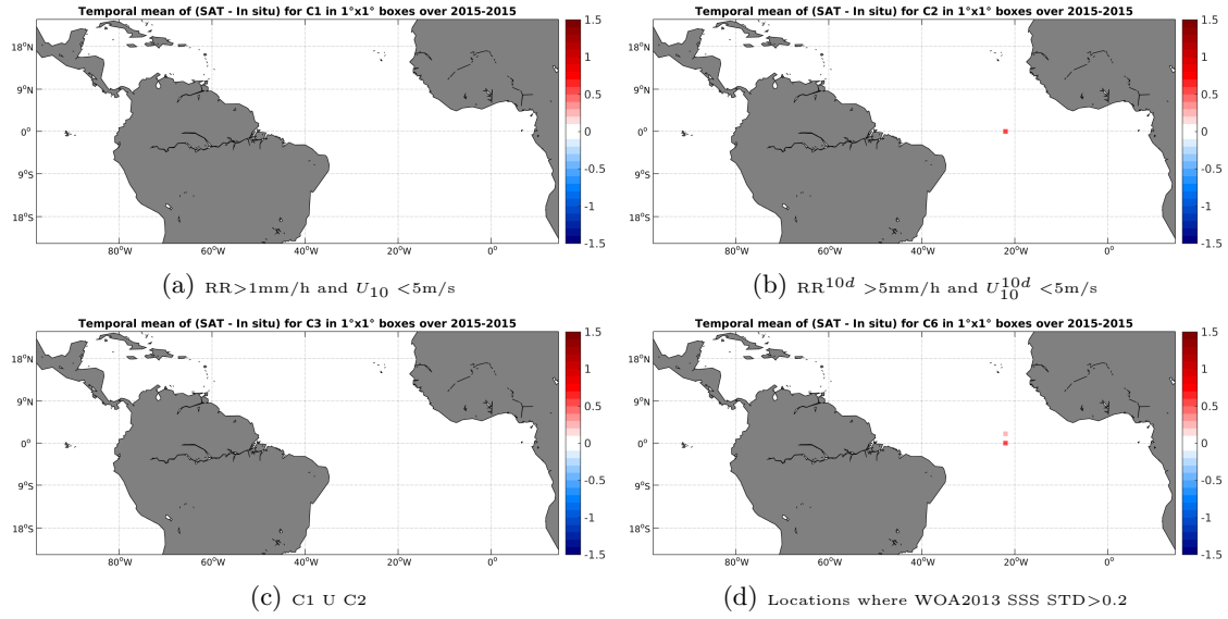
Figure 11: Temporal mean gridded over spatial boxes of size 1^\circ \times 1^\circ of \Delta SSS (SMAP-L3-RSS-V2-MONTHLY-70KM - Surface drifters) for 4 different subdatasets corresponding to: RR > 1 mm/h and U_{10} < 5 m/s (a), RR^{10d} > 5 mm/h and U_{10}^{10d} < 5 m/s (b), C1 U C2 (c), Locations where WOA2013 SSS STD > 0.2 (d).
