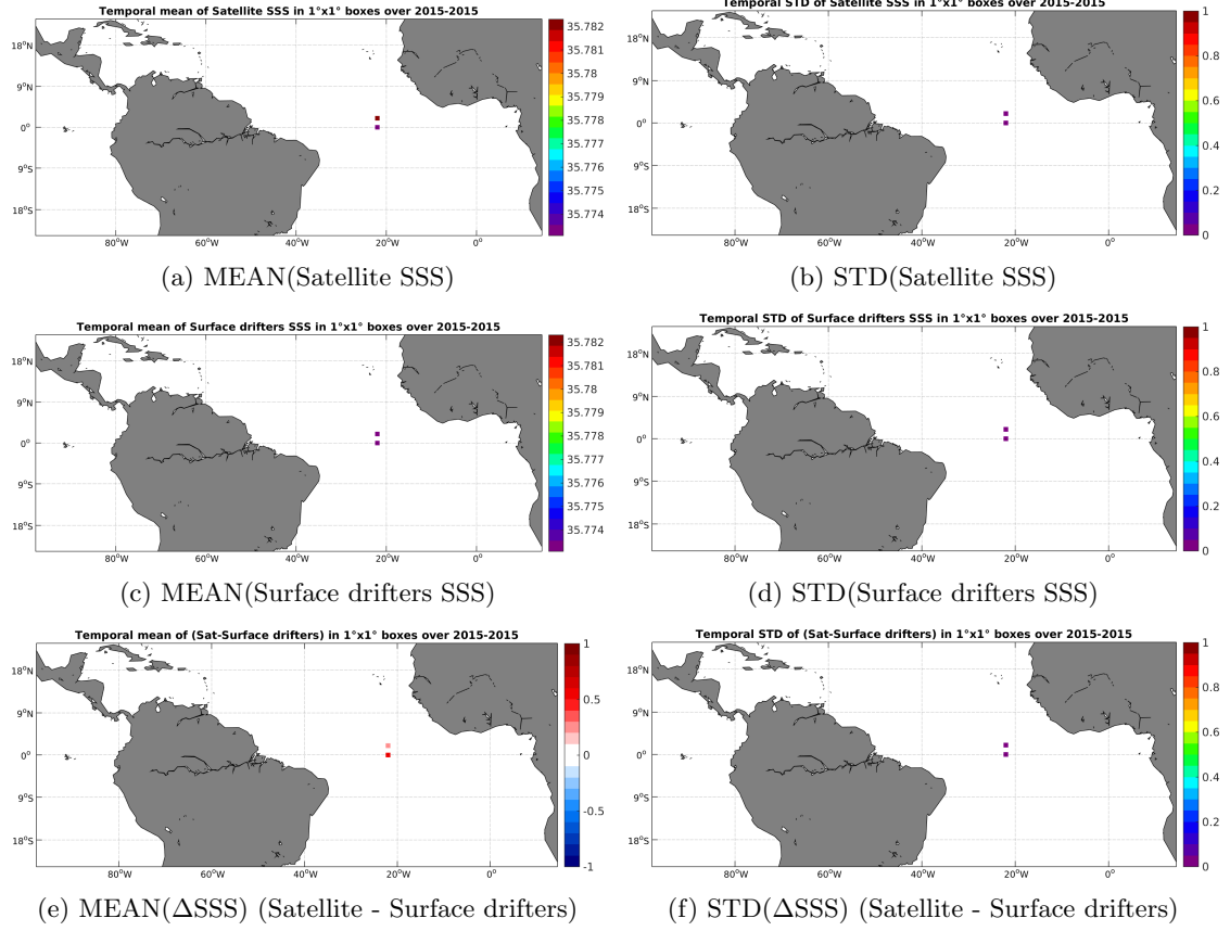
Figure 5: Temporal mean (left) and STD (right) of SSS from SMAP-L3-RSS-V2-MONTHLY-70KM (top), Surface drifters (middle), and of \Delta SSS (Satellite - Surface drifters). Only match-up pairs are used to generate these maps.
