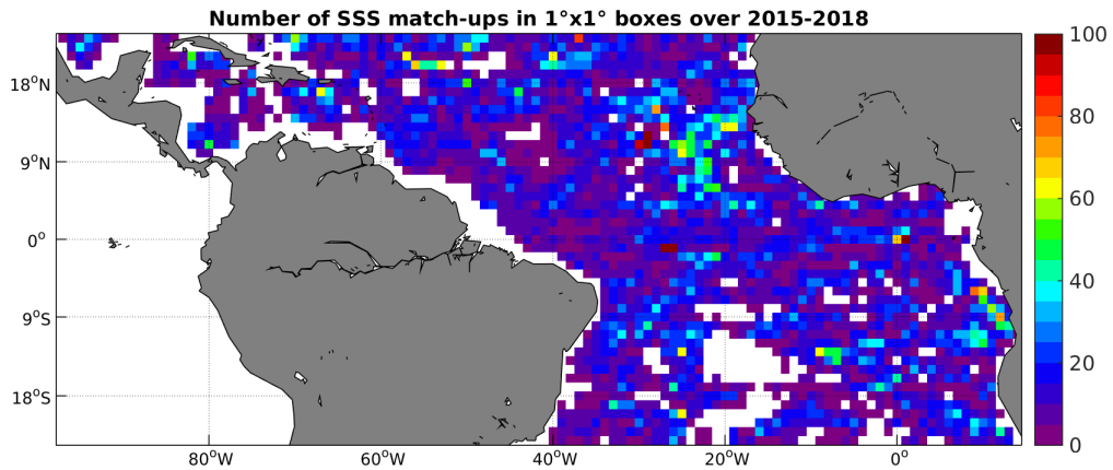
Figure 4: Number of SSS match-ups between Argo SSS and the SMAP-L3-RSS-V2-MONTHLY-70KM SSS product for the Tropical Atlantic Ocean Pi-MEP region over 1^\circ \times 1^\circ boxes and for the full satellite product period.
