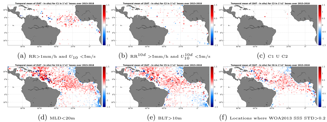
Figure 12: Temporal mean gridded over spatial boxes of size 1^\circ \times 1^\circ of \Delta SSS (SMAP-L3-RSS-V2-MONTHLY-70KM - Argo) for 6 different subdatasets corresponding to:RR>1mm/h and U_{10} < 5\text{m/s} (a), RR^{10d} > 5\text{mm/h} and U_{10}^{10d} < 5\text{m/s} (b), C1 U C2 (c),MLD<20m (d),BLT>10m (e),Locations where WOA2013 SSS STD>0.2 (f).
