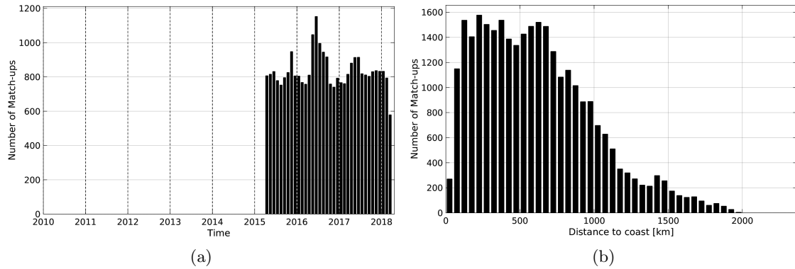
Figure 1: Number of match-ups between Argo and SMAP-L3-RSS-V2-MONTHLY-70KM SSS as a function of time (a) and as function of the distance to coast (b) over the Tropical Atlantic Ocean Pi-MEP region and for the full satellite product period.
