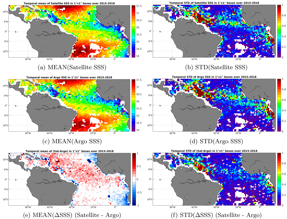
Figure 6: Temporal mean (left) and STD (right) of SSS from SMAP-L3-RSS-V2-MONTHLY-70KM (top), Argo (middle), and of \Delta SSS (Satellite - Argo). Only match-up pairs are used to generate these maps.
