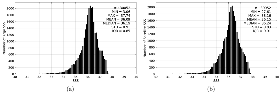
Figure 2: Histograms of SSS from Argo (a) and SMAP-L3-RSS-V2-MONTHLY-70KM (b) considering all match-up pairs per bins of 0.1 over the Tropical Atlantic Ocean Pi-MEP region and for the full satellite product period.
