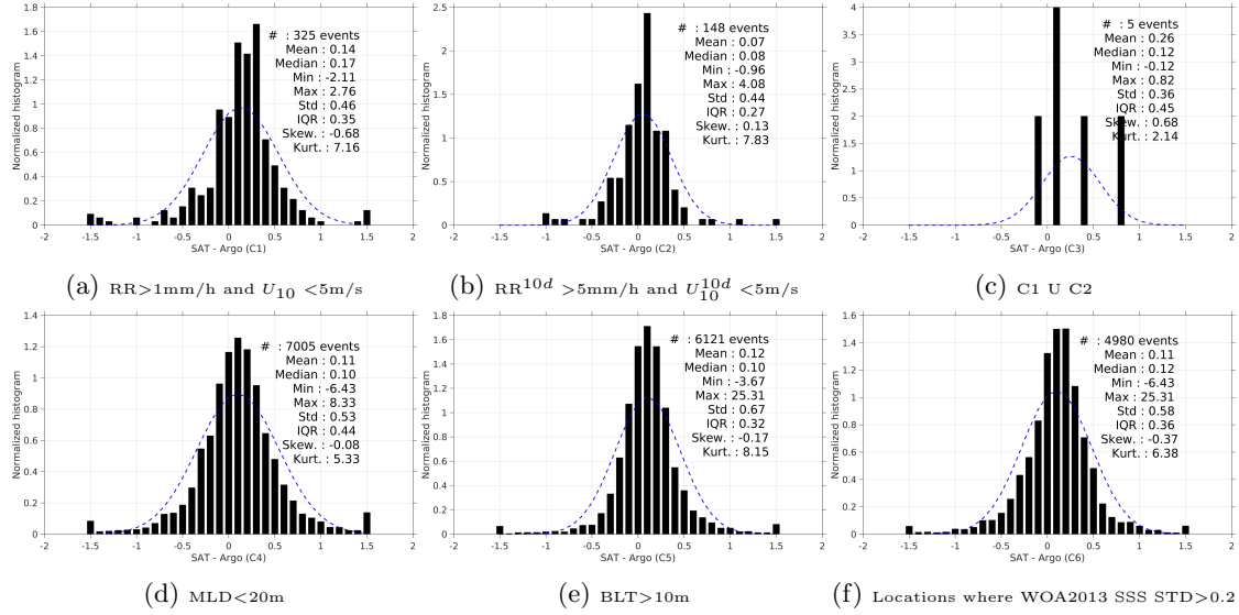
Figure 13: Normalized histogram of \Delta SSS (SMAP-L3-RSS-V2-MONTHLY-70KM - Argo) for 6 different subdatasets corresponding to: RR > 1mm/h and U_{10} < 5 m/s (a), RR^{10d} > 5 mm/h and U_{10}^{10d} < 5 m/s (b), C1 U C2 (c), MLD < 20m (d), BLT > 10m (e), Locations where WOA2013 SSS STD > 0.2 (f).
