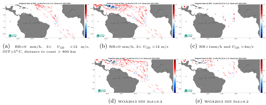
Figure 14: Temporal mean gridded over spatial boxes of size 1^\circ \times 1^\circ of \Delta\text{SSS} (SMAP SSS L3 v5.0 - 8-Day running (JPL) - TSG (SAMOS)) for 5 different subdatasets corresponding to:RR=0 mm/h, 3 < U_{10} < 12 m/s, SST >5^\circ\text{C} , distance to coast > 800 km (a), RR=0 mm/h, 3 < U_{10} < 12 m/s (b), RR >1 mm/h and U_{10} < 4 m/s (c), WOA2013 SSS Std <0.2 (d), WOA2013 SSS Std >0.2 (e).
