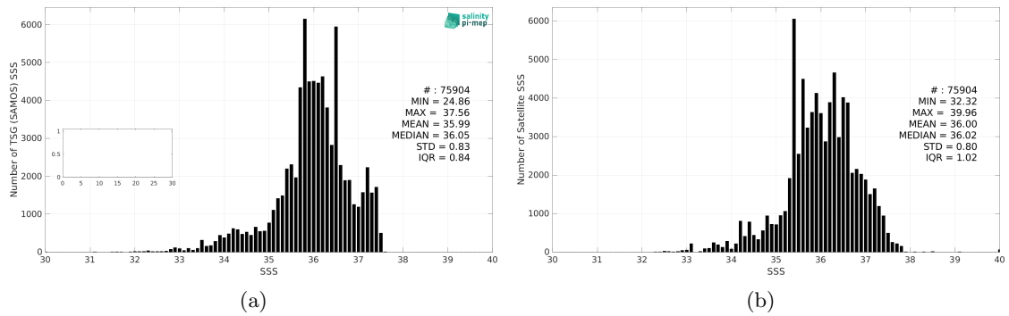
Figure 3: Histograms of SSS from TSG (SAMOS) (a) and SMAP SSS L3 v5.0 - 8-Day running (JPL) (b) considering all match-up pairs per bins of 0.1 over the Tropical Atlantic Ocean Pi-MEP region and for the full satellite product period.
