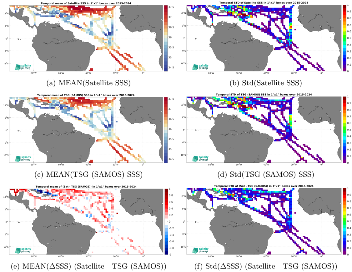
Figure 7: Temporal mean (left) and Std (right) of SSS from SMAP SSS L3 v5.0 - 8-Day running (JPL) (top), TSG (SAMOS) (middle), and of \Delta SSS (Satellite - TSG (SAMOS)). Only match-up pairs are used to generate these maps.
