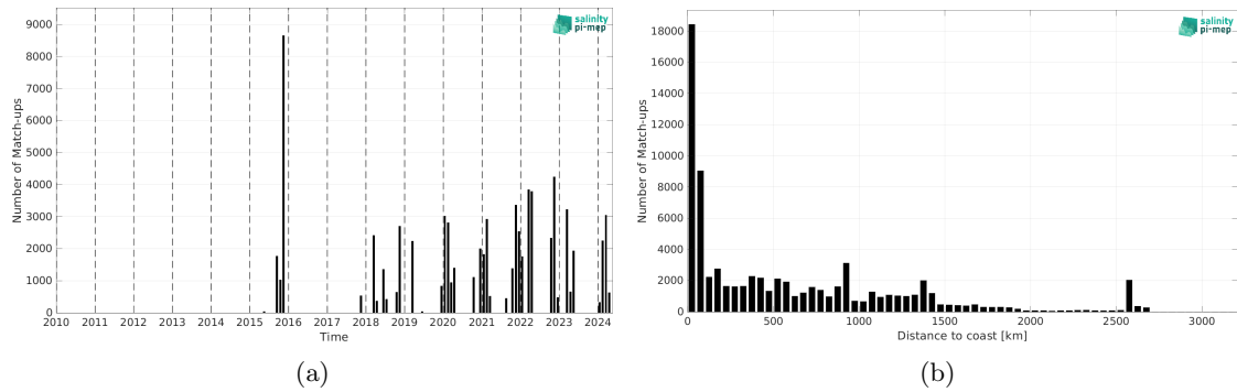
Figure 2: Number of match-ups between TSG (SAMOS) and SMAP SSS L3 v5.0 - 8-Day running (JPL) SSS as a function of time (a) and as function of the distance to coast (b) over the Tropical Atlantic Ocean Pi-MEP region and for the full satellite product period.
