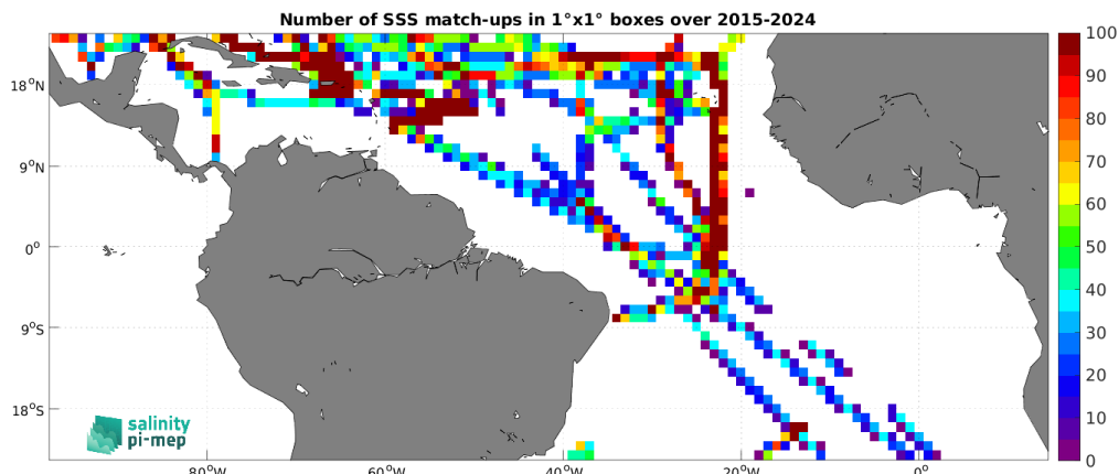
Figure 5: Number of SSS match-ups between TSG (SAMOS) SSS and the SMAP SSS L3 v5.0 - 8-Day running (JPL) SSS product for the Tropical Atlantic Ocean Pi-MEP region over 1^\circ \times 1^\circ boxes and for the full satellite product period.
