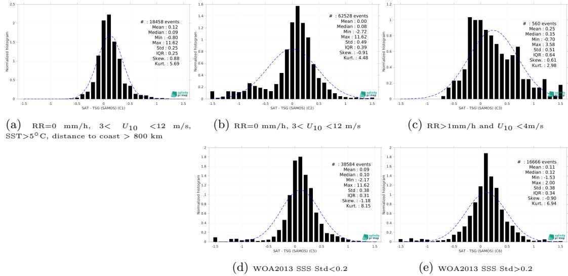
Figure 15: Normalized histogram of \Delta\text{SSS} (SMAP SSS L3 v5.0 - 8-Day running (JPL) - TSG (SAMOS)) for 5 different subdatasets corresponding to: RR=0 mm/h, 3 < U_{10} < 12 m/s, SST>5°C, distance to coast > 800 km (a), RR=0 mm/h, 3 < U_{10} < 12 m/s (b), RR>1mm/h and U_{10} < 4 m/s (c), WOA2013 SSS Std<0.2 (d), WOA2013 SSS Std>0.2 (e).
