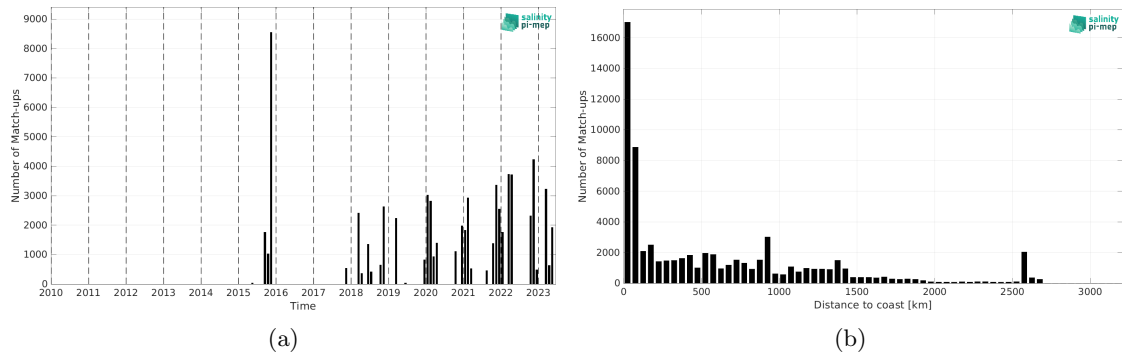
Figure 1: Number of match-ups between TSG (SAMOS) and SMAP SSS L3 v5.0 - 8-Day running (JPL) SSS as a function of time (a) and as function of the distance to coast (b) over the Tropical Atlantic Ocean Pi-MEP region and for the full satellite product period.
