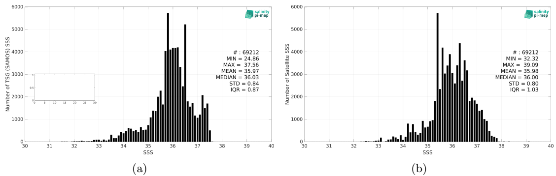
Figure 2: Histograms of SSS from TSG (SAMOS) (a) and SMAP SSS L3 v5.0 - 8-Day running (JPL) (b) considering all match-up pairs per bins of 0.1 over the Tropical Atlantic Ocean Pi-MEP region and for the full satellite product period.
