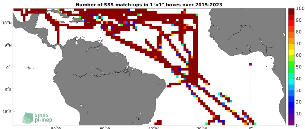
Figure 4: Number of SSS match-ups between TSG (SAMOS) SSS and the SMAP SSS L3 v5.0 - 8-Day running (JPL) SSS product for the Tropical Atlantic Ocean Pi-MEP region over 1^\circ \times 1^\circ boxes and for the full satellite product period.
