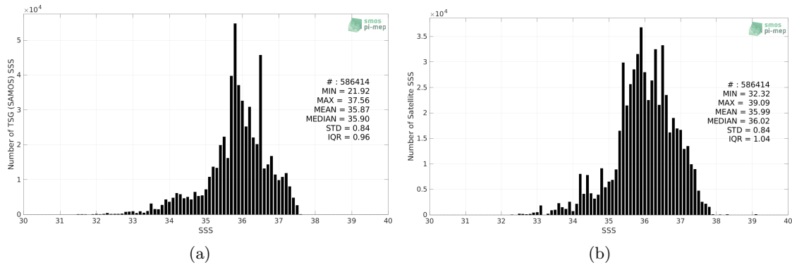
Figure 2: Histograms of SSS from TSG (SAMOS) (a) and SMAP SSS L3 v5.0 - 8-Day running (JPL) (b) considering all match-up pairs per bins of 0.1 over the Tropical Atlantic Ocean Pi-MEP region and for the full satellite product period.
