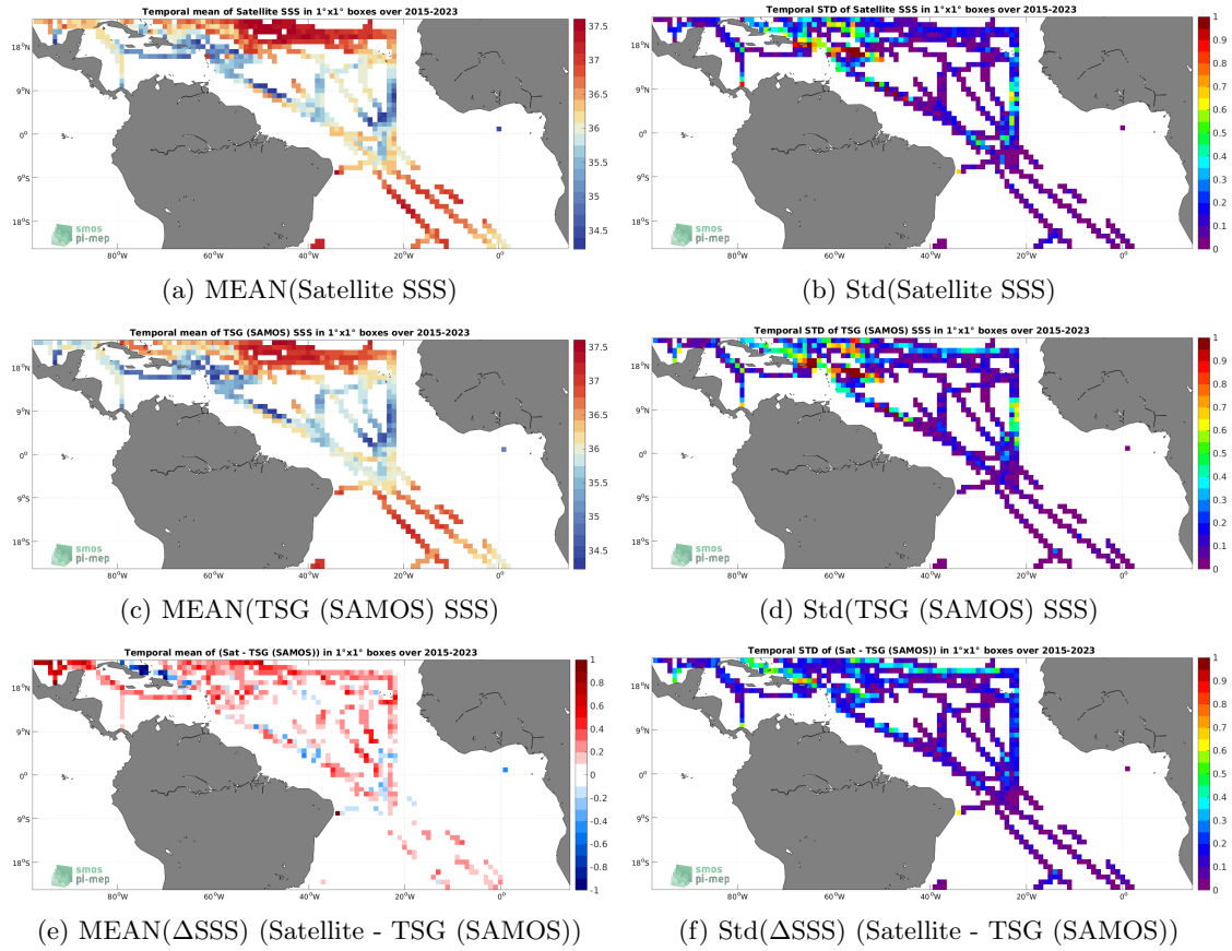
Figure 6: Temporal mean (left) and Std (right) of SSS from SMAP SSS L3 v5.0 - 8-Day running (JPL) (top), TSG (SAMOS) (middle), and of \Delta SSS (Satellite - TSG (SAMOS)). Only match-up pairs are used to generate these maps.
