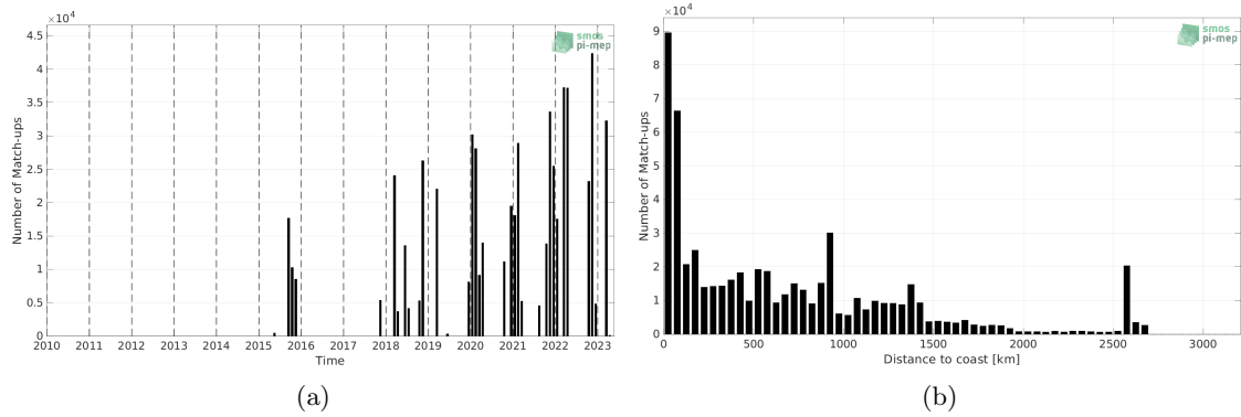
Figure 1: Number of match-ups between TSG (SAMOS) and SMAP SSS L3 v5.0 - 8-Day running (JPL) SSS as a function of time (a) and as function of the distance to coast (b) over the Tropical Atlantic Ocean Pi-MEP region and for the full satellite product period.
