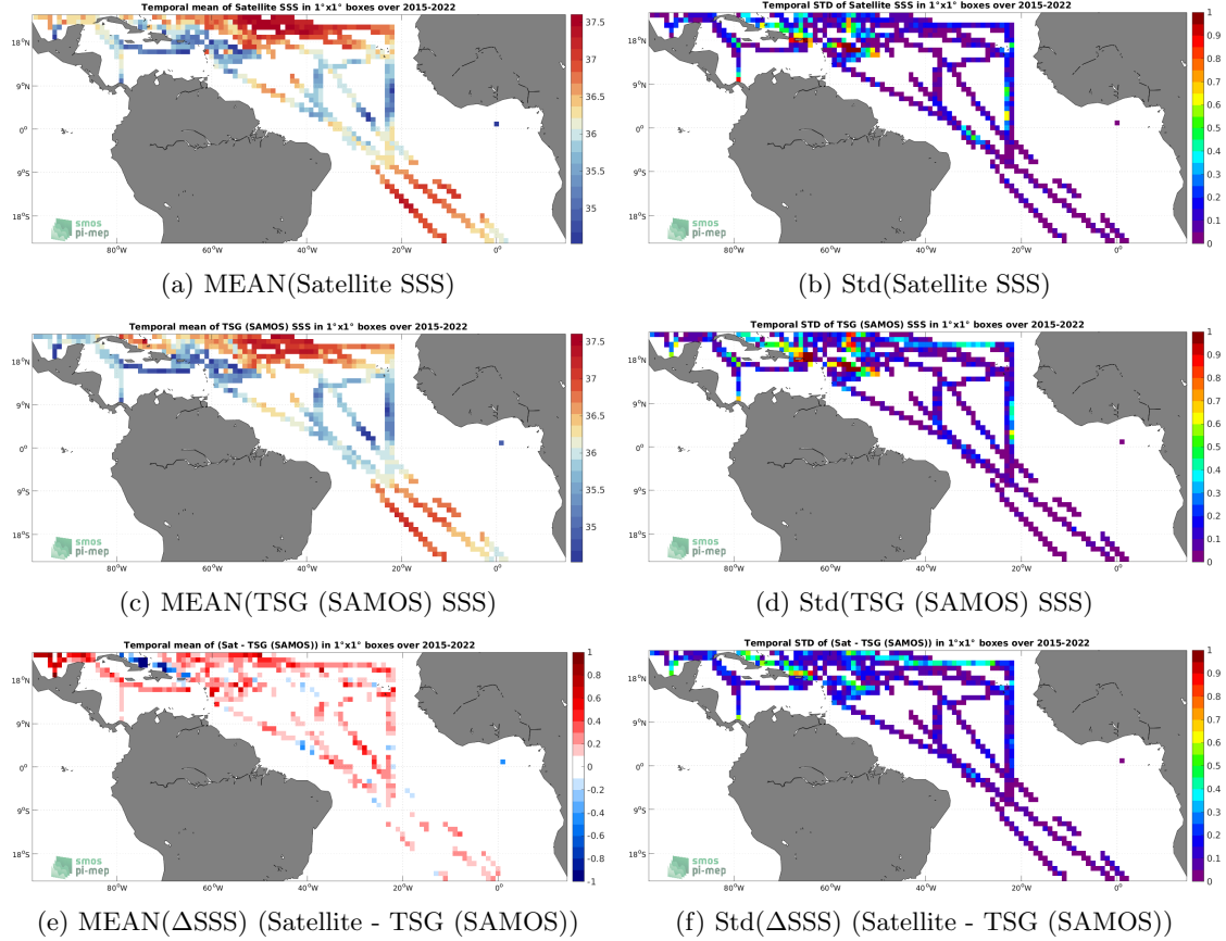
Figure 6: Temporal mean (left) and Std (right) of SSS from SMAP SSS L3 v5.0 - 8-Day running (JPL) (top), TSG (SAMOS) (middle), and of \Delta\text{SSS} (Satellite - TSG (SAMOS)). Only match-up pairs are used to generate these maps.
