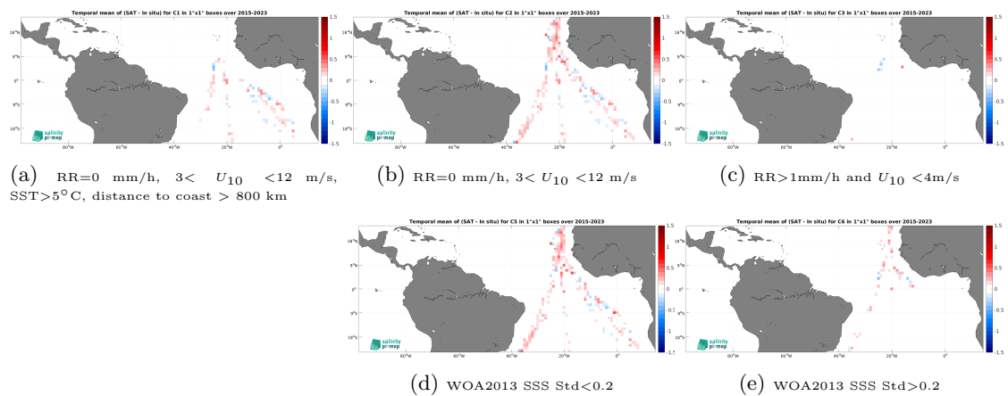
Figure 14: Temporal mean gridded over spatial boxes of size 1^\circ \times 1^\circ of \Delta SSS (SMAP SSS L3 v5.0 - 8-Day running (JPL) - TSG (Polarstern)) for 5 different subdatasets corresponding to:RR=0 mm/h, 3 < U_{10} < 12 m/s, SST >5^\circ C, distance to coast > 800 km (a), RR=0 mm/h, 3 < U_{10} < 12 m/s (b), RR >1 mm/h and U_{10} < 4 m/s (c), WOA2013 SSS Std <0.2 (d), WOA2013 SSS Std >0.2 (e).
