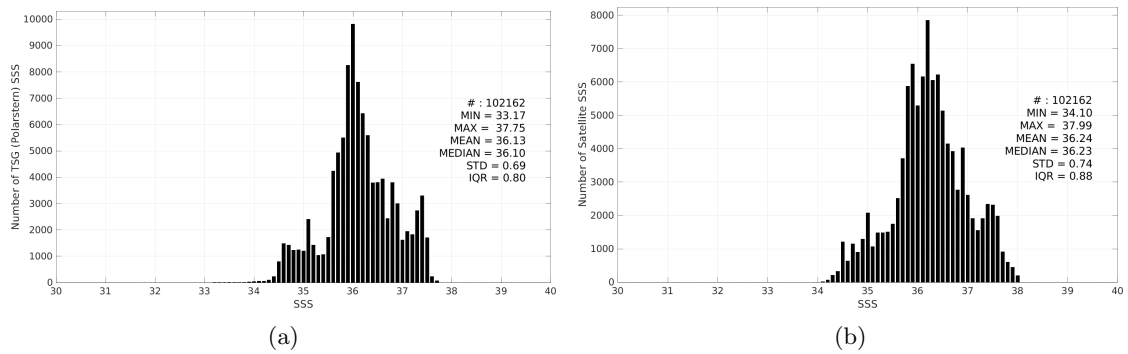
Figure 3: Histograms of SSS from TSG (Polarstern) (a) and SMAP SSS L3 v5.0 - 8-Day running (JPL) (b) considering all match-up pairs per bins of 0.1 over the Tropical Atlantic Ocean Pi-MEP region and for the full satellite product period.
