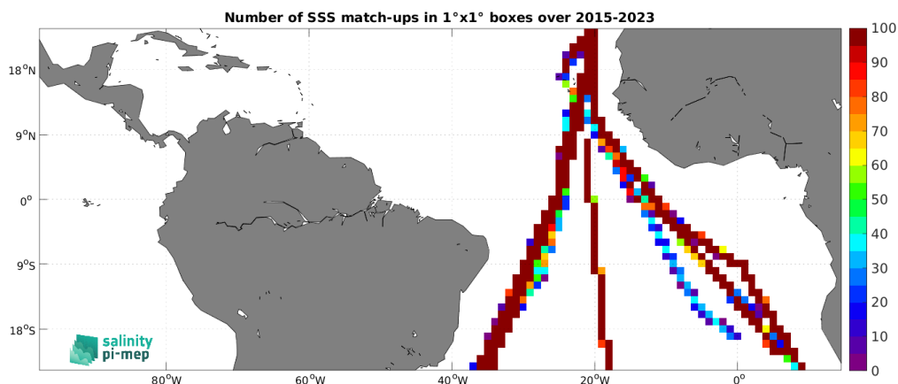
Figure 5: Number of SSS match-ups between TSG (Polarstern) SSS and the SMAP SSS L3 v5.0 - 8-Day running (JPL) SSS product for the Tropical Atlantic Ocean Pi-MEP region over 1^\circ \times 1^\circ boxes and for the full satellite product period.
