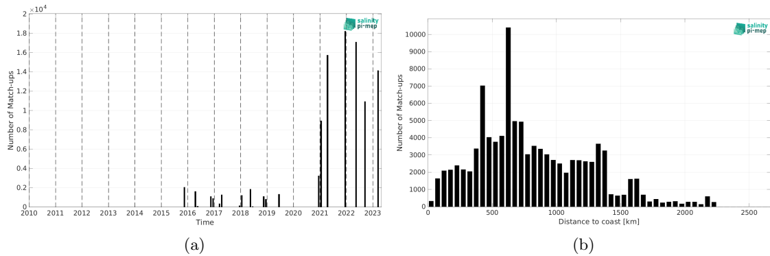
Figure 2: Number of match-ups between TSG (Polarstern) and SMAP SSS L3 v5.0 - 8-Day running (JPL) SSS as a function of time (a) and as function of the distance to coast (b) over the Tropical Atlantic Ocean Pi-MEP region and for the full satellite product period.
