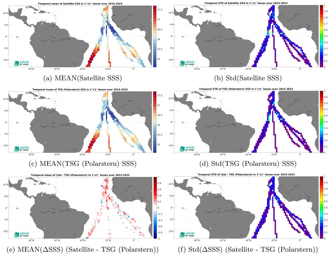
Figure 7: Temporal mean (left) and Std (right) of SSS from SMAP SSS L3 v5.0 - 8-Day running (JPL) (top), TSG (Polarstern) (middle), and of \Delta SSS (Satellite - TSG (Polarstern)). Only match-up pairs are used to generate these maps.
