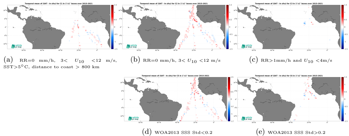
Figure 12: Temporal mean gridded over spatial boxes of size 1^\circ \times 1^\circ of \Delta\text{SSS} (SMAP SSS L3 v5.0 - 8-Day running (JPL) - TSG (Polarstern)) for 5 different subdatasets corresponding to:RR=0 mm/h, 3 < U_{10} < 12 m/s, SST >5^\circ\text{C} , distance to coast > 800 km (a), RR=0 mm/h, 3 < U_{10} < 12 m/s (b), RR >1 mm/h and U_{10} < 4 m/s (c), WOA2013 SSS Std <0.2 (d), WOA2013 SSS Std >0.2 (e).
