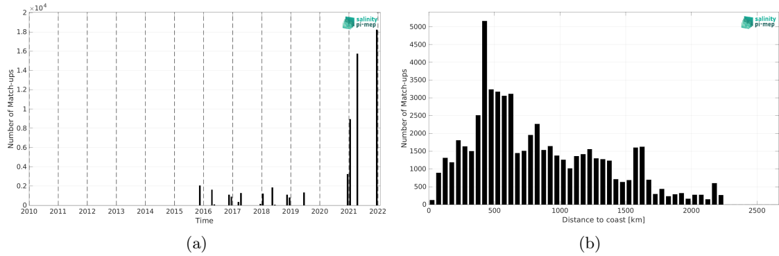
Figure 1: Number of match-ups between TSG (Polarstern) and SMAP SSS L3 v5.0 - 8-Day running (JPL) SSS as a function of time (a) and as function of the distance to coast (b) over the Tropical Atlantic Ocean Pi-MEP region and for the full satellite product period.
