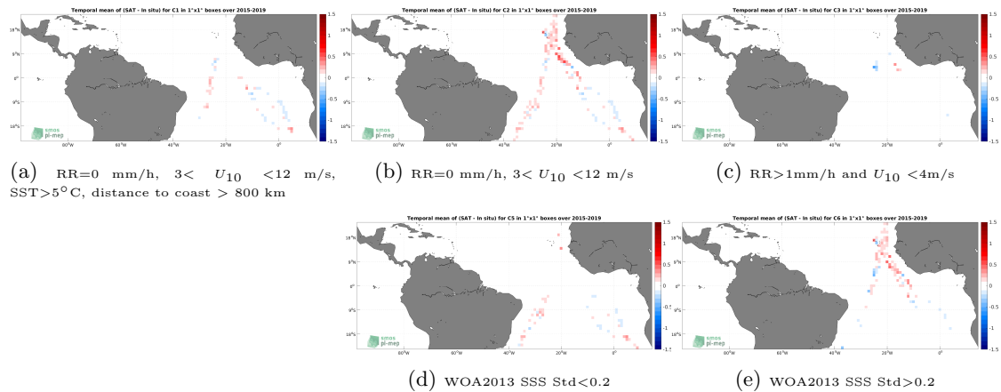
Figure 12: Temporal mean gridded over spatial boxes of size 1^\circ \times 1^\circ of \Delta SSS (SMAP SSS L3 v5.0 - 8-Day running (JPL) - TSG (Polarstern)) for 5 different subdatasets corresponding to:RR=0 mm/h, 3 < U_{10} < 12 m/s, SST >5^\circ C, distance to coast > 800 km (a), RR=0 mm/h, 3 < U_{10} < 12 m/s (b), RR >1 mm/h and U_{10} < 4 m/s (c), WOA2013 SSS Std <0.2 (d), WOA2013 SSS Std >0.2 (e).
