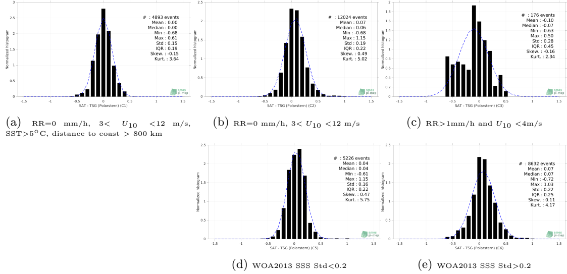
Figure 13: Normalized histogram of \Delta\text{SSS} (SMAP SSS L3 v5.0 - 8-Day running (JPL) - TSG (Polarstern)) for 5 different subdatasets corresponding to: RR=0 mm/h, 3 < U_{10} < 12 m/s, SST>5°C, distance to coast > 800 km (a), RR=0 mm/h, 3 < U_{10} < 12 m/s (b), RR>1mm/h and U_{10} < 4 m/s (c), WOA2013 SSS Std<0.2 (d), WOA2013 SSS Std>0.2 (e).
