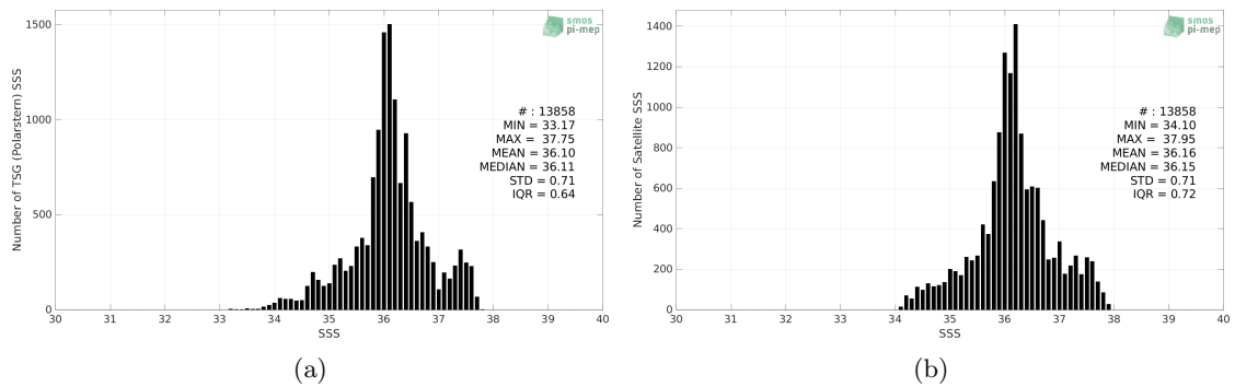
Figure 2: Histograms of SSS from TSG (Polarstern) (a) and SMAP SSS L3 v5.0 - 8-Day running (JPL) (b) considering all match-up pairs per bins of 0.1 over the Tropical Atlantic Ocean Pi-MEP region and for the full satellite product period.
