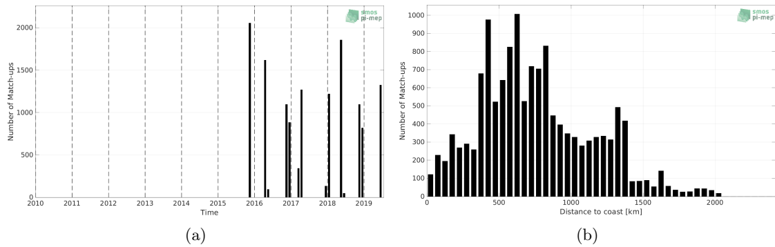
Figure 1: Number of match-ups between TSG (Polarstern) and SMAP SSS L3 v5.0 - 8-Day running (JPL) SSS as a function of time (a) and as function of the distance to coast (b) over the Tropical Atlantic Ocean Pi-MEP region and for the full satellite product period.
