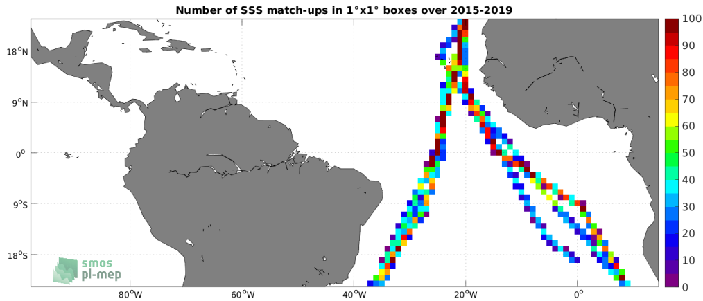
Figure 4: Number of SSS match-ups between TSG (Polarstern) SSS and the SMAP SSS L3 v5.0 - 8-Day running (JPL) SSS product for the Tropical Atlantic Ocean Pi-MEP region over 1^\circ \times 1^\circ boxes and for the full satellite product period.
