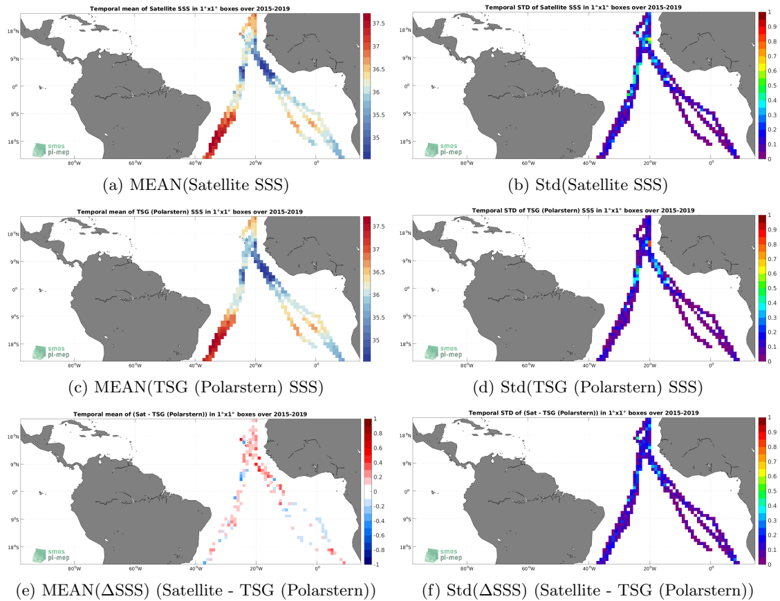
Figure 6: Temporal mean (left) and Std (right) of SSS from SMAP SSS L3 v5.0 - 8-Day running (JPL) (top), TSG (Polarstern) (middle), and of \Delta SSS (Satellite - TSG (Polarstern)). Only match-up pairs are used to generate these maps.
