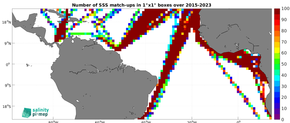
Figure 5: Number of SSS match-ups between TSG (LEGOS-DM) SSS and the SMAP SSS L3 v5.0 - 8-Day running (JPL) SSS product for the Tropical Atlantic Ocean Pi-MEP region over 1°×1° boxes and for the full satellite product period.
