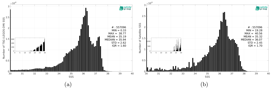
Figure 3: Histograms of SSS from TSG (LEGOS-DM) (a) and SMAP SSS L3 v5.0 - 8-Day running (JPL) (b) considering all match-up pairs per bins of 0.1 over the Tropical Atlantic Ocean Pi-MEP region and for the full satellite product period.
