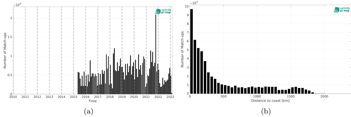
Figure 2: Number of match-ups between TSG (LEGOS-DM) and SMAP SSS L3 v5.0 - 8-Day running (JPL) SSS as a function of time (a) and as function of the distance to coast (b) over the Tropical Atlantic Ocean Pi-MEP region and for the full satellite product period.
