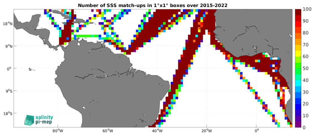
Figure 5: Number of SSS match-ups between TSG (LEGOS-DM) SSS and the SMAP SSS L3 v5.0 - 8-Day running (JPL) SSS product for the Tropical Atlantic Ocean Pi-MEP region over 1^\circ \times 1^\circ boxes and for the full satellite product period.
