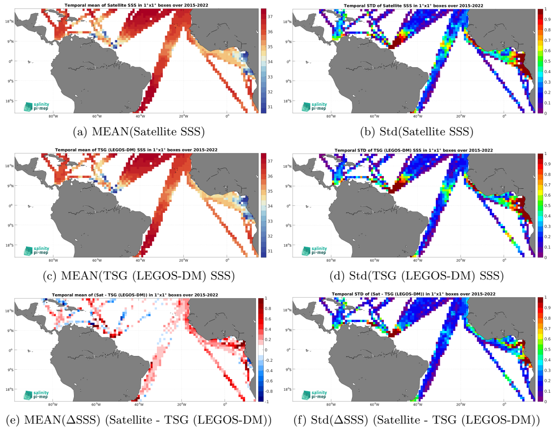
Figure 6: Temporal mean (left) and Std (right) of SSS from SMAP SSS L3 v5.0 - 8-Day running (JPL) (top), TSG (LEGOS-DM) (middle), and of \Delta SSS (Satellite - TSG (LEGOS-DM)). Only match-up pairs are used to generate these maps.
