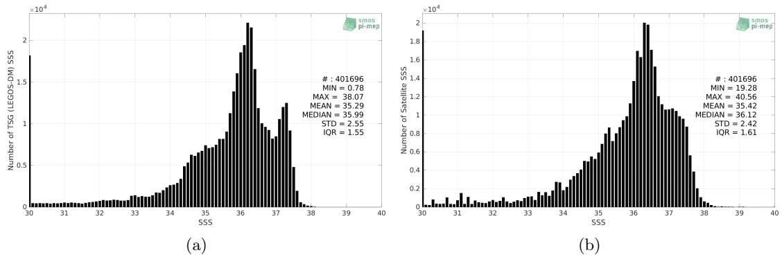
Figure 2: Histograms of SSS from TSG (LEGOS-DM) (a) and SMAP SSS L3 v5.0 - 8-Day running (JPL) (b) considering all match-up pairs per bins of 0.1 over the Tropical Atlantic Ocean Pi-MEP region and for the full satellite product period.
