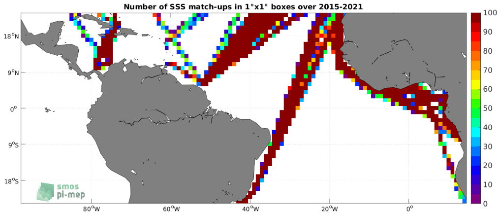
Figure 4: Number of SSS match-ups between TSG (LEGOS-DM) SSS and the SMAP SSS L3 v5.0 - 8-Day running (JPL) SSS product for the Tropical Atlantic Ocean Pi-MEP region over 1^\circ \times 1^\circ boxes and for the full satellite product period.
