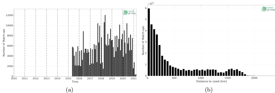
Figure 1: Number of match-ups between TSG (LEGOS-DM) and SMAP SSS L3 v5.0 - 8-Day running (JPL) SSS as a function of time (a) and as function of the distance to coast (b) over the Tropical Atlantic Ocean Pi-MEP region and for the full satellite product period.
