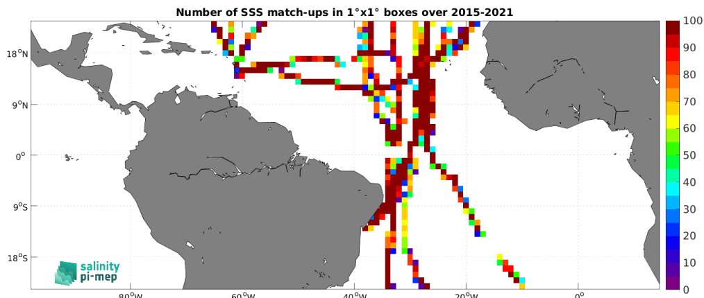
Figure 5: Number of SSS match-ups between TSG (GOSUD-Sailing-ship) SSS and the SMAP SSS L3 v5.0 - 8-Day running (JPL) SSS product for the Tropical Atlantic Ocean Pi-MEP region over 1^\circ \times 1^\circ boxes and for the full satellite product period.
