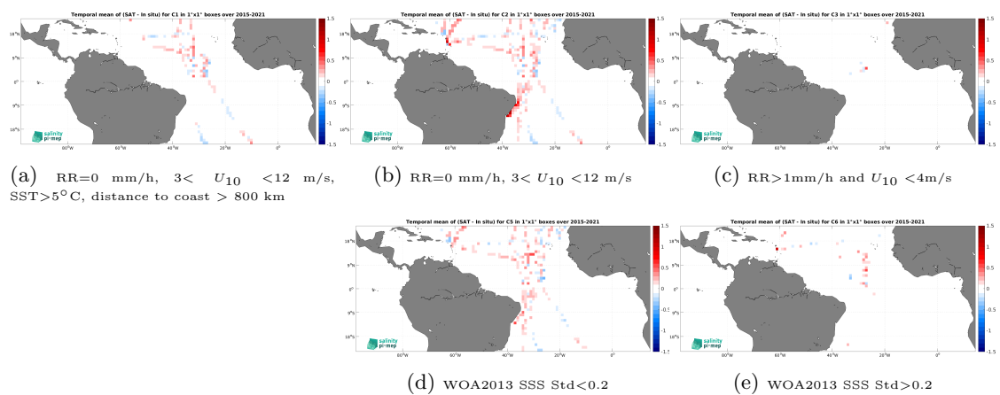
Figure 14: Temporal mean gridded over spatial boxes of size 1^\circ \times 1^\circ of \Delta\text{SSS} (SMAP SSS L3 v5.0 - 8-Day running (JPL) - TSG (GOSUD-Sailing-ship)) for 5 different subdatasets corresponding to:RR=0 mm/h, 3 < U_{10} < 12 m/s, SST>5°C, distance to coast > 800 km (a), RR=0 mm/h, 3 < U_{10} < 12 m/s (b), RR>1mm/h and U_{10} < 4 m/s (c), WOA2013 SSS Std<0.2 (d), WOA2013 SSS Std>0.2 (e).
