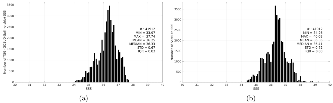
Figure 3: Histograms of SSS from TSG (GOSUD-Sailing-ship) (a) and SMAP SSS L3 v5.0 - 8-Day running (JPL) (b) considering all match-up pairs per bins of 0.1 over the Tropical Atlantic Ocean Pi-MEP region and for the full satellite product period.
