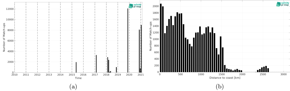
Figure 2: Number of match-ups between TSG (GOSUD-Sailing-ship) and SMAP SSS L3 v5.0 - 8-Day running (JPL) SSS as a function of time (a) and as function of the distance to coast (b) over the Tropical Atlantic Ocean Pi-MEP region and for the full satellite product period.
