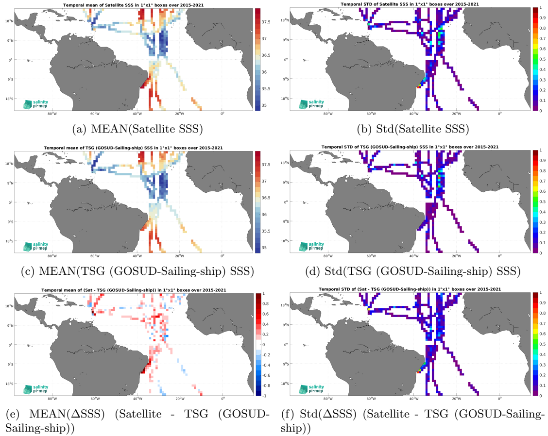
Figure 7: Temporal mean (left) and Std (right) of SSS from SMAP SSS L3 v5.0 - 8-Day running (JPL) (top), TSG (GOSUD-Sailing-ship) (middle), and of \Delta SSS (Satellite - TSG (GOSUD-Sailing-ship)). Only match-up pairs are used to generate these maps.
