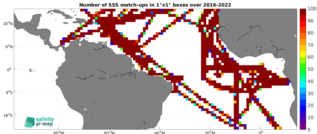
Figure 5: Number of SSS match-ups between TSG (GOSUD-Research-vessel) SSS and the SMAP SSS L3 v5.0 - 8-Day running (JPL) SSS product for the Tropical Atlantic Ocean Pi-MEP region over 1^\circ \times 1^\circ boxes and for the full satellite product period.
