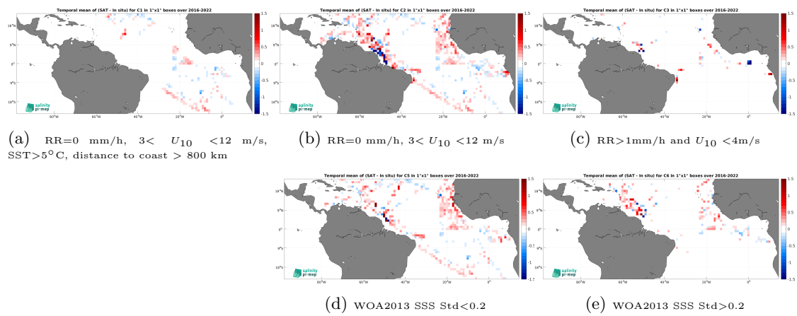
Figure 14: Temporal mean gridded over spatial boxes of size 1^\circ \times 1^\circ of \Delta SSS (SMAP SSS L3 v5.0 - 8-Day running (JPL) - TSG (GOSUD-Research-vessel)) for 5 different subdatasets corresponding to:RR=0 mm/h, 3 < U_{10} < 12 m/s, SST >5^\circ\text{C} , distance to coast > 800 km (a), RR=0 mm/h, 3 < U_{10} < 12 m/s (b), RR >1 mm/h and U_{10} < 4 m/s (c), WOA2013 SSS Std <0.2 (d), WOA2013 SSS Std >0.2 (e).
