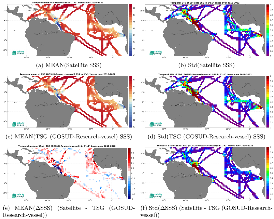
Figure 7: Temporal mean (left) and Std (right) of SSS from SMAP SSS L3 v5.0 - 8-Day running (JPL) (top), TSG (GOSUD-Research-vessel) (middle), and of \Delta SSS (Satellite - TSG (GOSUD-Research-vessel)). Only match-up pairs are used to generate these maps.
