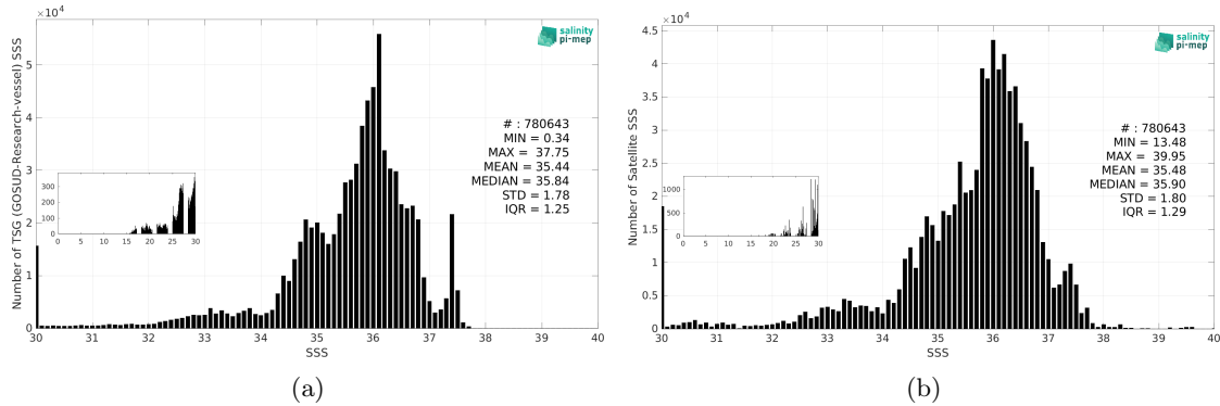
Figure 3: Histograms of SSS from TSG (GOSUD-Research-vessel) (a) and SMAP SSS L3 v5.0 - 8-Day running (JPL) (b) considering all match-up pairs per bins of 0.1 over the Tropical Atlantic Ocean Pi-MEP region and for the full satellite product period.
