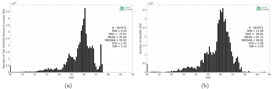
Figure 2: Histograms of SSS from TSG (GOSUD-Research-vessel) (a) and SMAP SSS L3 v5.0 - 8-Day running (JPL) (b) considering all match-up pairs per bins of 0.1 over the Tropical Atlantic Ocean Pi-MEP region and for the full satellite product period.
