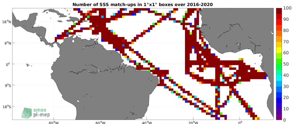
Figure 4: Number of SSS match-ups between TSG (GOSUD-Research-vessel) SSS and the SMAP SSS L3 v5.0 - 8-Day running (JPL) SSS product for the Tropical Atlantic Ocean Pi-MEP region over 1^\circ \times 1^\circ boxes and for the full satellite product period.
