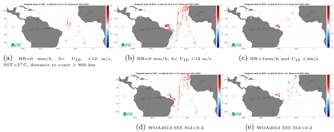
Figure 14: Temporal mean gridded over spatial boxes of size 1^\circ \times 1^\circ of \Delta SSS (SMAP SSS L3 v5.0 - 8-Day running (JPL) - TSG (CSIC-UTM)) for 5 different subdatasets corresponding to:RR=0 mm/h, 3 < U_{10} < 12 m/s, SST >5^\circ C, distance to coast > 800 km (a), RR=0 mm/h, 3 < U_{10} < 12 m/s (b), RR >1 mm/h and U_{10} < 4 m/s (c), WOA2013 SSS Std <0.2 (d), WOA2013 SSS Std >0.2 (e).
