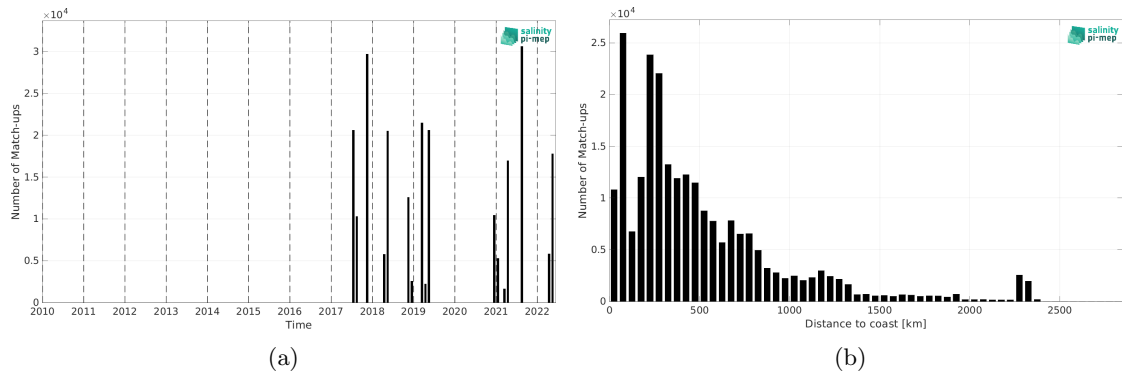
Figure 2: Number of match-ups between TSG (CSIC-UTM) and SMAP SSS L3 v5.0 - 8-Day running (JPL) SSS as a function of time (a) and as function of the distance to coast (b) over the Tropical Atlantic Ocean Pi-MEP region and for the full satellite product period.
