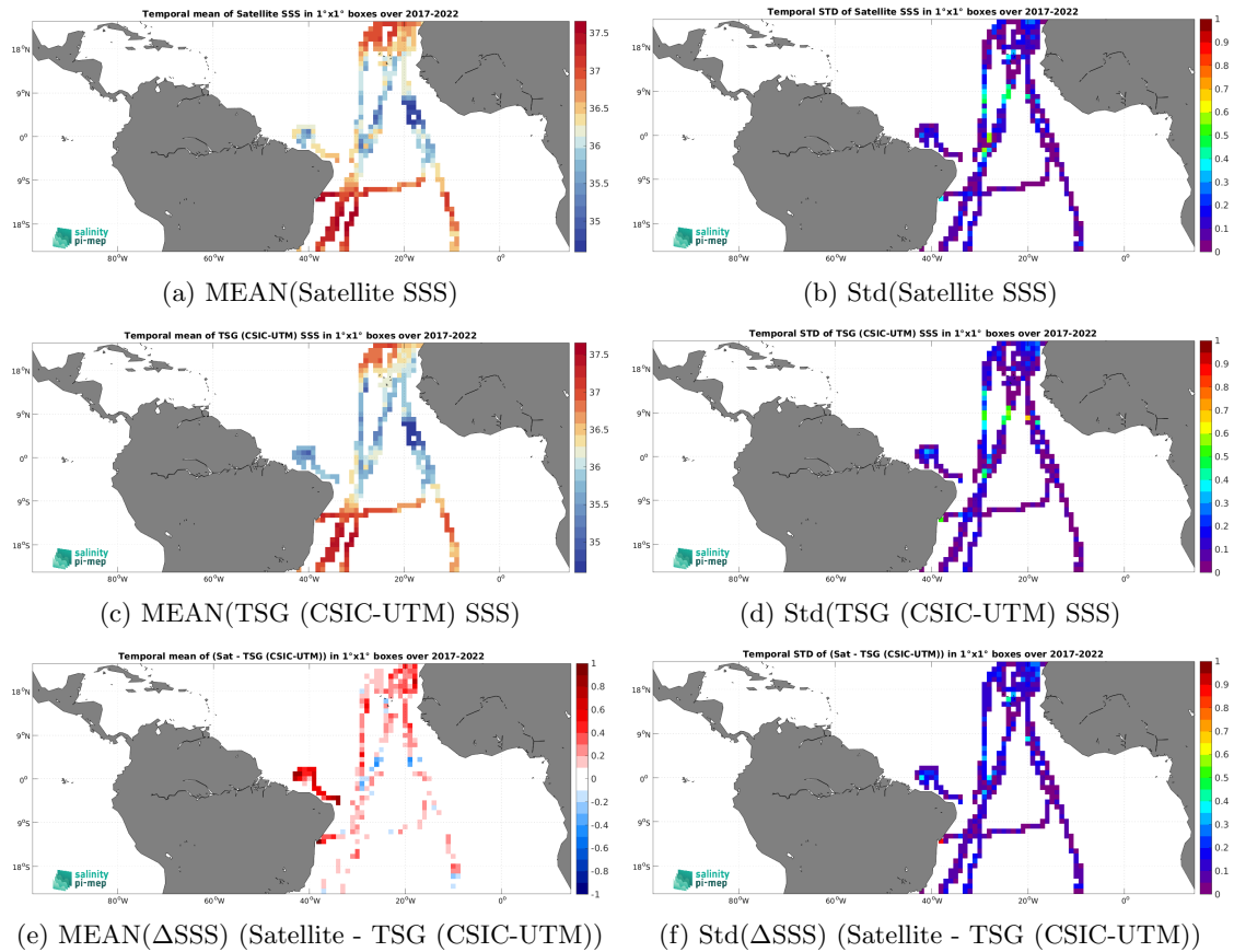
Figure 7: Temporal mean (left) and Std (right) of SSS from SMAP SSS L3 v5.0 - 8-Day running (JPL) (top), TSG (CSIC-UTM) (middle), and of \Delta SSS (Satellite - TSG (CSIC-UTM)). Only match-up pairs are used to generate these maps.
