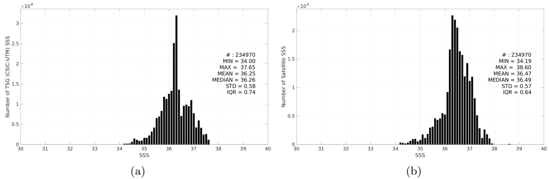
Figure 3: Histograms of SSS from TSG (CSIC-UTM) (a) and SMAP SSS L3 v5.0 - 8-Day running (JPL) (b) considering all match-up pairs per bins of 0.1 over the Tropical Atlantic Ocean Pi-MEP region and for the full satellite product period.
