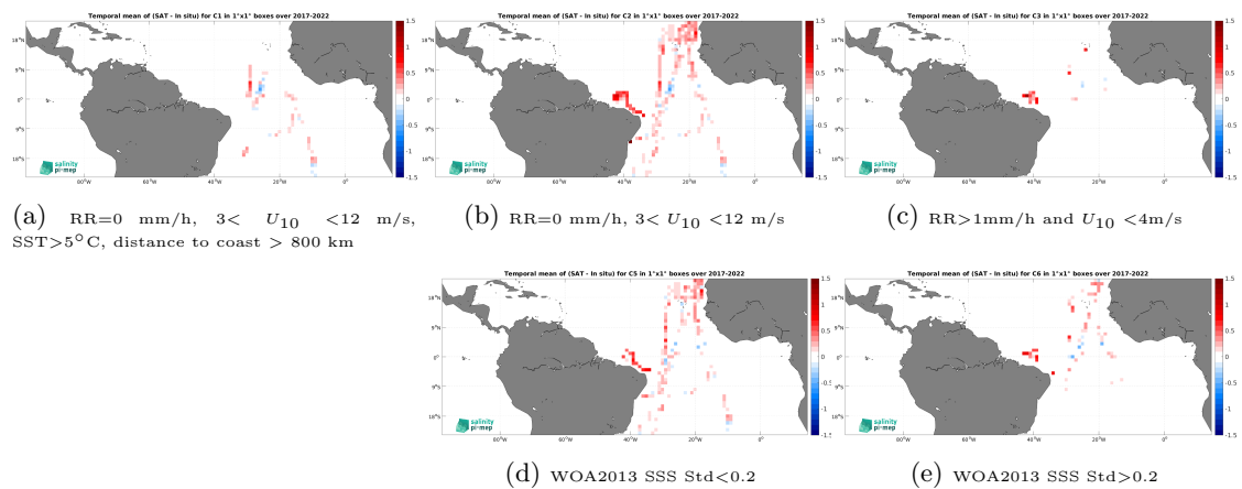
Figure 14: Temporal mean gridded over spatial boxes of size 1^\circ \times 1^\circ of \Delta SSS (SMAP SSS L3 v5.0 - 8-Day running (JPL) - TSG (CSIC-UTM)) for 5 different subdatasets corresponding to:RR=0 mm/h, 3 < U_{10} < 12 m/s, SST >5^\circ C, distance to coast > 800 km (a), RR=0 mm/h, 3 < U_{10} < 12 m/s (b), RR >1 mm/h and U_{10} < 4 m/s (c), WOA2013 SSS Std <0.2 (d), WOA2013 SSS Std >0.2 (e).
