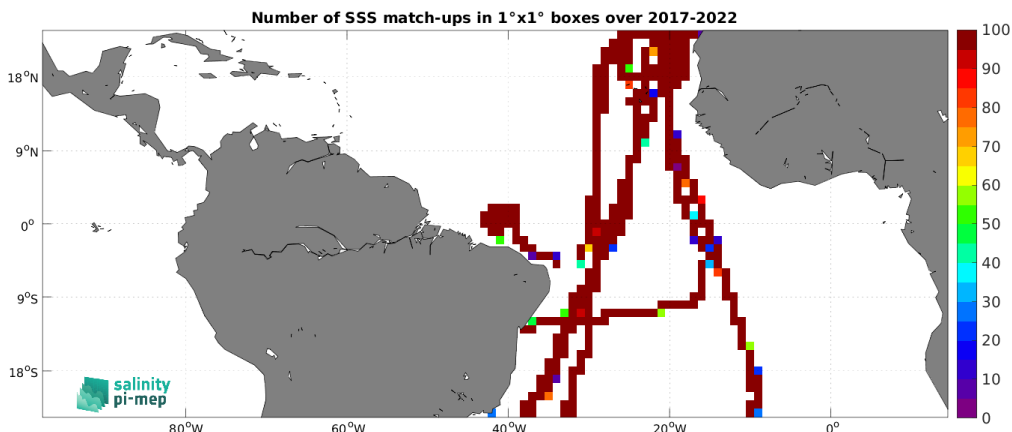
Figure 5: Number of SSS match-ups between TSG (CSIC-UTM) SSS and the SMAP SSS L3 v5.0 - 8-Day running (JPL) SSS product for the Tropical Atlantic Ocean Pi-MEP region over 1^\circ \times 1^\circ boxes and for the full satellite product period.
