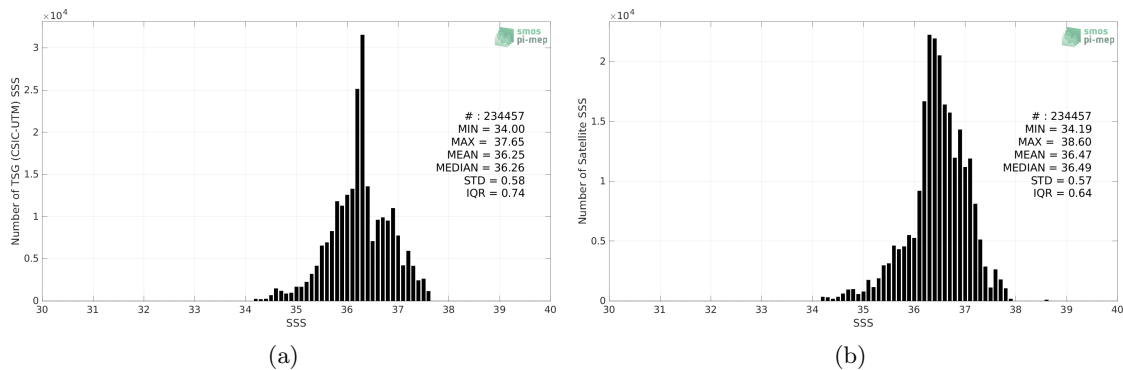
Figure 2: Histograms of SSS from TSG (CSIC-UTM) (a) and SMAP SSS L3 v5.0 - 8-Day running (JPL) (b) considering all match-up pairs per bins of 0.1 over the Tropical Atlantic Ocean Pi-MEP region and for the full satellite product period.
