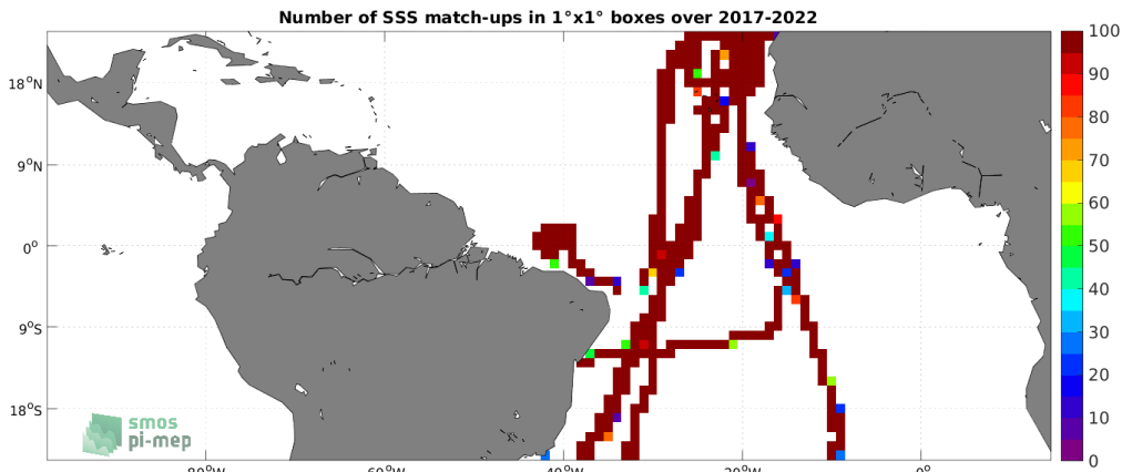
Figure 4: Number of SSS match-ups between TSG (CSIC-UTM) SSS and the SMAP SSS L3 v5.0 - 8-Day running (JPL) SSS product for the Tropical Atlantic Ocean Pi-MEP region over 1^\circ \times 1^\circ boxes and for the full satellite product period.
