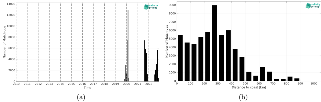
Figure 1: Number of match-ups between Sairdron and SMAP SSS L3 v5.0 - 8-Day running (JPL) SSS as a function of time (a) and as function of the distance to coast (b) over the Tropical Atlantic Ocean Pi-MEP region and for the full satellite product period.
