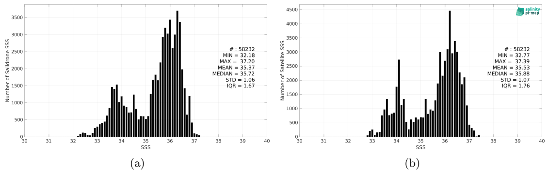
Figure 2: Histograms of SSS from Sairdron (a) and SMAP SSS L3 v5.0 - 8-Day running (JPL) (b) considering all match-up pairs per bins of 0.1 over the Tropical Atlantic Ocean Pi-MEP region and for the full satellite product period.
