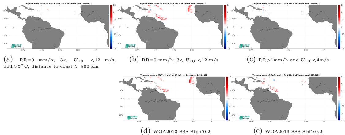
Figure 12: Temporal mean gridded over spatial boxes of size 1^\circ \times 1^\circ of \Delta\text{SSS} (SMAP SSS L3 v5.0 - 8-Day running (JPL) - Saildrone) for 5 different subdatasets corresponding to:RR=0 mm/h, 3 < U_{10} < 12 m/s, SST >5^\circ\text{C} , distance to coast > 800 km (a), RR=0 mm/h, 3 < U_{10} < 12 m/s (b), RR >1 mm/h and U_{10} < 4 m/s (c), WOA2013 SSS Std <0.2 (d), WOA2013 SSS Std >0.2 (e).
