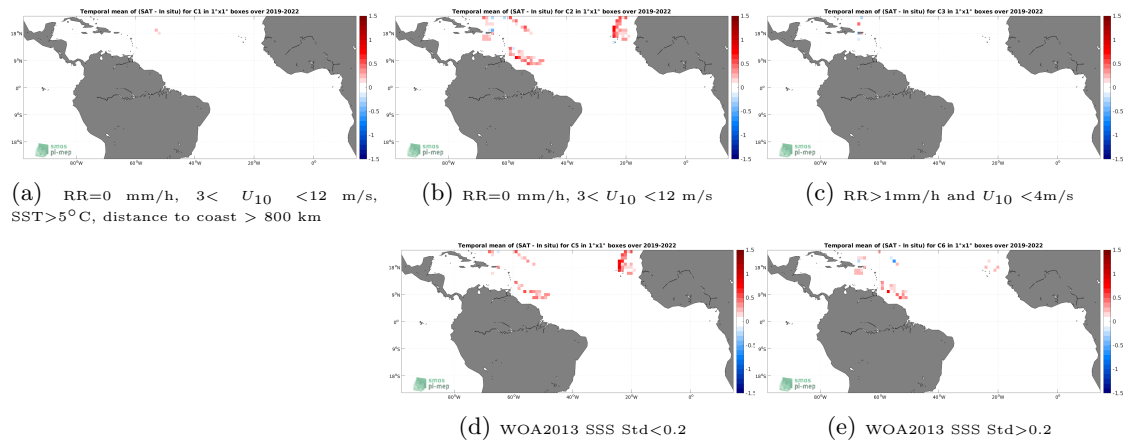
Figure 12: Temporal mean gridded over spatial boxes of size 1^\circ \times 1^\circ of \Delta SSS (SMAP SSS L3 v5.0 - 8-Day running (JPL) - Saildrone) for 5 different subdatasets corresponding to:RR=0 mm/h, 3 < U_{10} < 12 m/s, SST >5^\circ\text{C} , distance to coast > 800 km (a), RR=0 mm/h, 3 < U_{10} < 12 m/s (b), RR >1 mm/h and U_{10} < 4 m/s (c), WOA2013 SSS Std <0.2 (d), WOA2013 SSS Std >0.2 (e).
