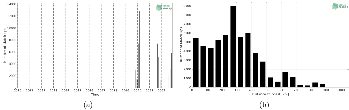
Figure 1: Number of match-ups between Saildrone and SMAP SSS L3 v5.0 - 8-Day running (JPL) SSS as a function of time (a) and as function of the distance to coast (b) over the Tropical Atlantic Ocean Pi-MEP region and for the full satellite product period.
