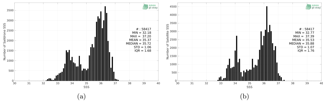
Figure 2: Histograms of SSS from Saildrone (a) and SMAP SSS L3 v5.0 - 8-Day running (JPL) (b) considering all match-up pairs per bins of 0.1 over the Tropical Atlantic Ocean Pi-MEP region and for the full satellite product period.
