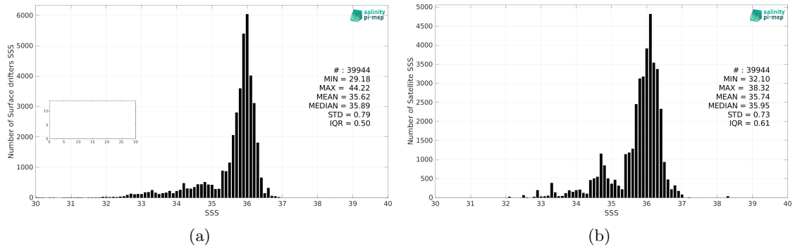
Figure 2: Histograms of SSS from Surface drifters (a) and SMAP SSS L3 v5.0 - 8-Day running (JPL) (b) considering all match-up pairs per bins of 0.1 over the Tropical Atlantic Ocean Pi-MEP region and for the full satellite product period.
