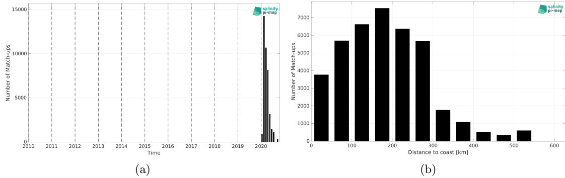
Figure 1: Number of match-ups between Surface drifters and SMAP SSS L3 v5.0 - 8-Day running (JPL) SSS as a function of time (a) and as function of the distance to coast (b) over the Tropical Atlantic Ocean Pi-MEP region and for the full satellite product period.
