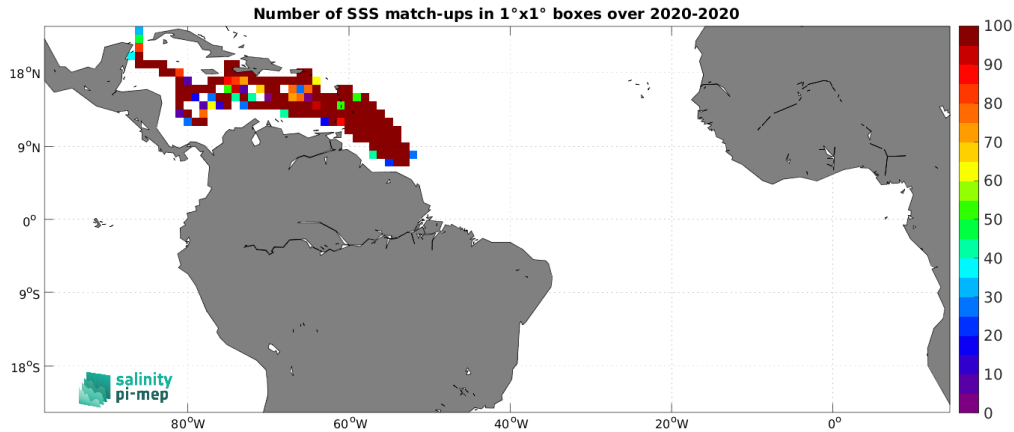
Figure 3: Number of SSS match-ups between Surface drifters SSS and the SMAP SSS L3 v5.0 - 8-Day running (JPL) SSS product for the Tropical Atlantic Ocean Pi-MEP region over 1^\circ \times 1^\circ boxes and for the full satellite product period.
