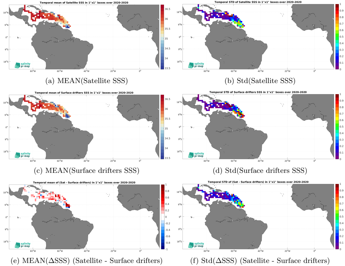
Figure 5: Temporal mean (left) and Std (right) of SSS from SMAP SSS L3 v5.0 - 8-Day running (JPL) (top), Surface drifters (middle), and of \Delta SSS (Satellite - Surface drifters). Only match-up pairs are used to generate these maps.
