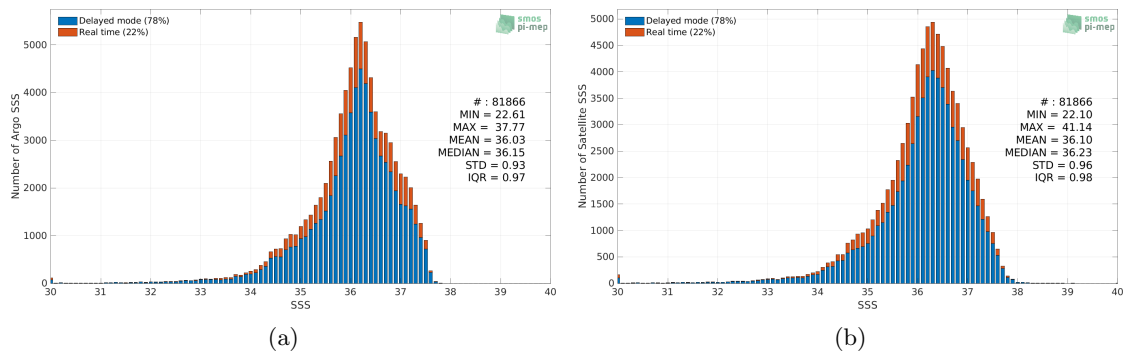
Figure 2: Histograms of SSS from Argo (a) and SMAP SSS L3 v5.0 - 8-Day running (JPL) (b) considering all match-up pairs per bins of 0.1 over the Tropical Atlantic Ocean Pi-MEP region and for the full satellite product period.
