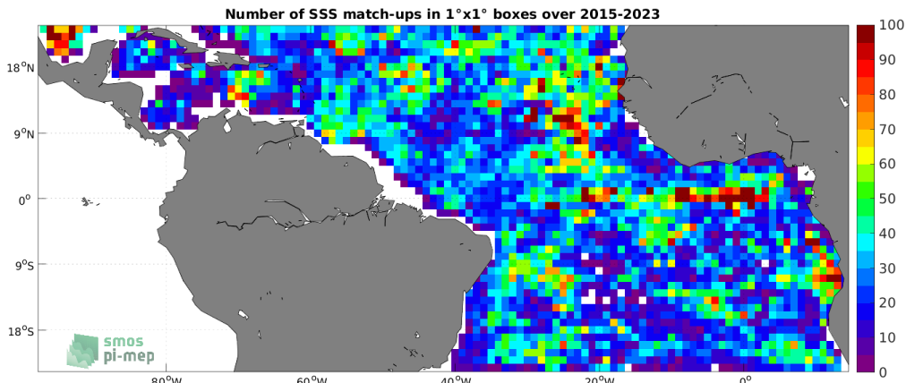
Figure 4: Number of SSS match-ups between Argo SSS and the SMAP SSS L3 v5.0 - 8-Day running (JPL) SSS product for the Tropical Atlantic Ocean Pi-MEP region over 1^\circ \times 1^\circ boxes and for the full satellite product period.
