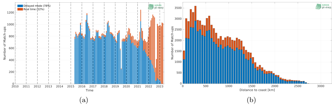
Figure 1: Number of match-ups between Argo and SMAP SSS L3 v5.0 - 8-Day running (JPL) SSS as a function of match-up time (a) and as function of the distance to coast (b) over the Tropical Atlantic Ocean Pi-MEP region and for the full satellite product period.
