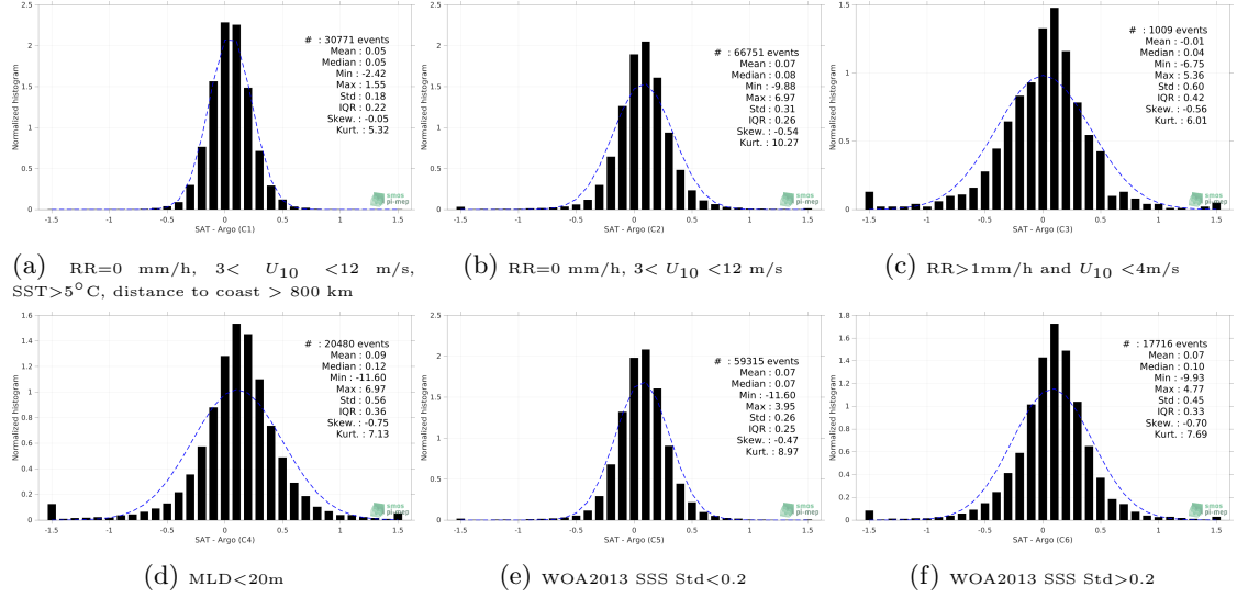
Figure 13: Normalized histogram of \Delta SSS (SMAP SSS L3 v5.0 - 8-Day running (JPL) - Argo) for 6 different subdatasets corresponding to: RR=0 mm/h, 3 < U_{10} < 12 m/s, SST > 5°C, distance to coast > 800 km (a), RR=0 mm/h, 3 < U_{10} < 12 m/s (b), RR > 1mm/h and U_{10} < 4 m/s (c), MLD < 20m (d), WOA2013 SSS Std < 0.2 (e), WOA2013 SSS Std > 0.2 (f).
