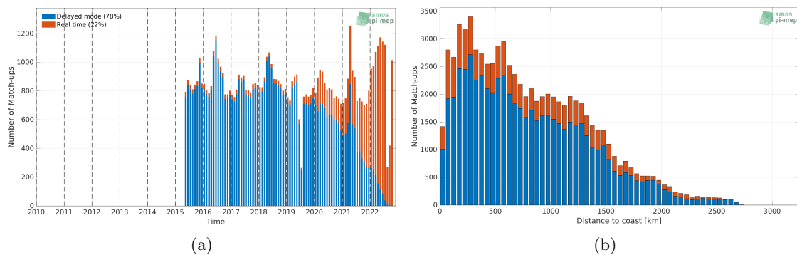
Figure 1: Number of match-ups between Argo and SMAP SSS L3 v5.0 - 8-Day running (JPL) SSS as a function of time (a) and as function of the distance to coast (b) over the Tropical Atlantic Ocean Pi-MEP region and for the full satellite product period.
