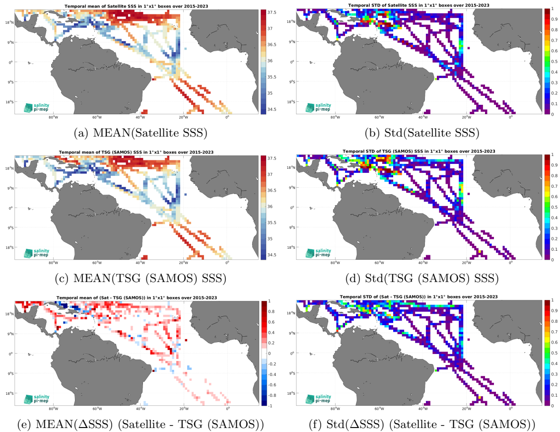
Figure 6: Temporal mean (left) and Std (right) of SSS from SMAP SSS L3 v5.0 - Monthly (JPL) (top), TSG (SAMOS) (middle), and of \Delta SSS (Satellite - TSG (SAMOS)). Only match-up pairs are used to generate these maps.
