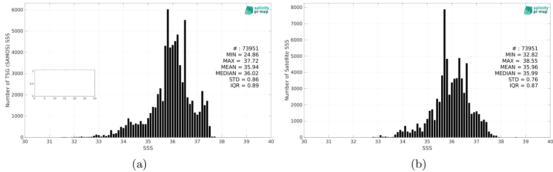
Figure 2: Histograms of SSS from TSG (SAMOS) (a) and SMAP SSS L3 v5.0 - Monthly (JPL) (b) considering all match-up pairs per bins of 0.1 over the Tropical Atlantic Ocean Pi-MEP region and for the full satellite product period.
