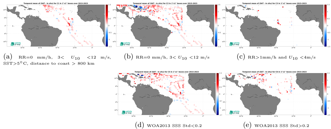
Figure 12: Temporal mean gridded over spatial boxes of size 1^\circ \times 1^\circ of \Delta\text{SSS} (SMAP SSS L3 v5.0 - Monthly (JPL) - TSG (SAMOS)) for 5 different subdatasets corresponding to:RR=0 mm/h, 3 < U_{10} < 12 m/s, SST >5^\circ\text{C} , distance to coast > 800 km (a), RR=0 mm/h, 3 < U_{10} < 12 m/s (b), RR >1 mm/h and U_{10} < 4 m/s (c), WOA2013 SSS Std <0.2 (d), WOA2013 SSS Std >0.2 (e).
