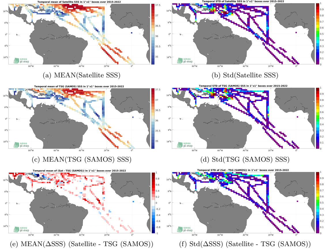
Figure 6: Temporal mean (left) and Std (right) of SSS from SMAP SSS L3 v5.0 - Monthly (JPL) (top), TSG (SAMOS) (middle), and of \Delta\text{SSS} (Satellite - TSG (SAMOS)). Only match-up pairs are used to generate these maps.
