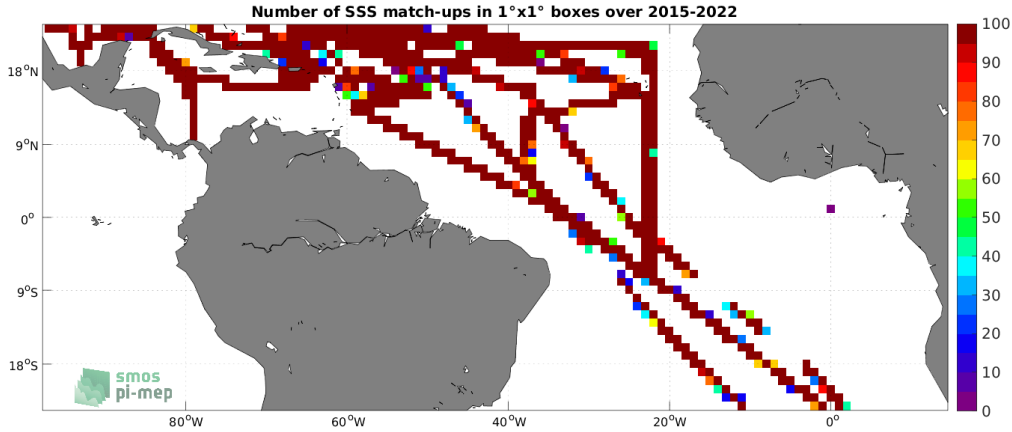
Figure 4: Number of SSS match-ups between TSG (SAMOS) SSS and the SMAP SSS L3 v5.0 - Monthly (JPL) SSS product for the Tropical Atlantic Ocean Pi-MEP region over 1^\circ \times 1^\circ boxes and for the full satellite product period.
