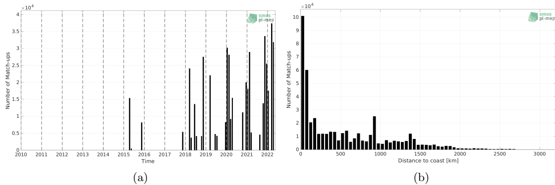
Figure 1: Number of match-ups between TSG (SAMOS) and SMAP SSS L3 v5.0 - Monthly (JPL) SSS as a function of time (a) and as function of the distance to coast (b) over the Tropical Atlantic Ocean Pi-MEP region and for the full satellite product period.
