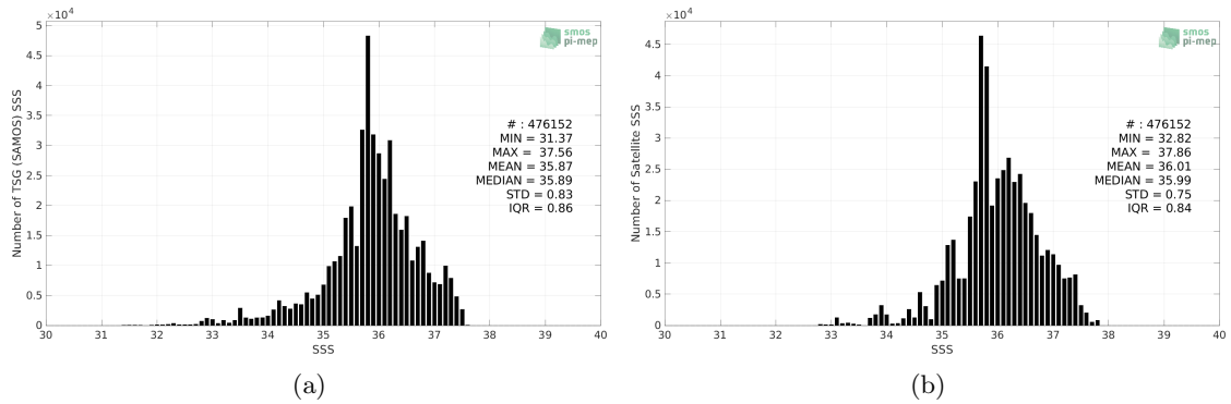
Figure 2: Histograms of SSS from TSG (SAMOS) (a) and SMAP SSS L3 v5.0 - Monthly (JPL) (b) considering all match-up pairs per bins of 0.1 over the Tropical Atlantic Ocean Pi-MEP region and for the full satellite product period.
