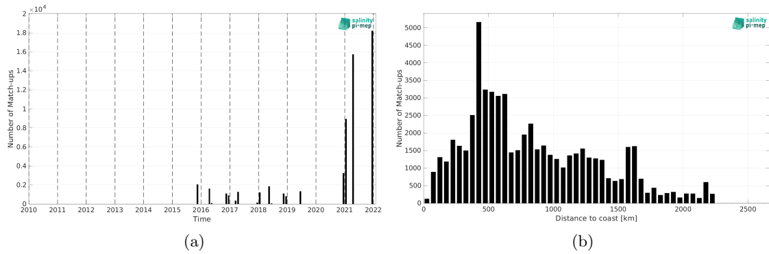
Figure 1: Number of match-ups between TSG (Polarstern) and SMAP SSS L3 v5.0 - Monthly (JPL) SSS as a function of time (a) and as function of the distance to coast (b) over the Tropical Atlantic Ocean Pi-MEP region and for the full satellite product period.
