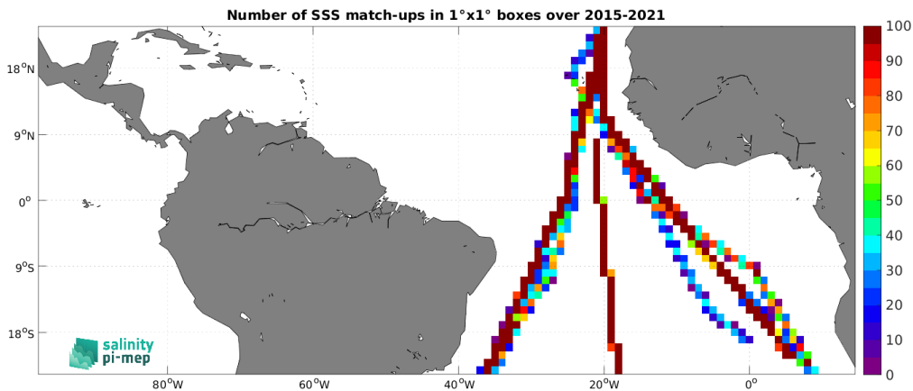
Figure 4: Number of SSS match-ups between TSG (Polarstern) SSS and the SMAP SSS L3 v5.0 - Monthly (JPL) SSS product for the Tropical Atlantic Ocean Pi-MEP region over 1^\circ \times 1^\circ boxes and for the full satellite product period.
